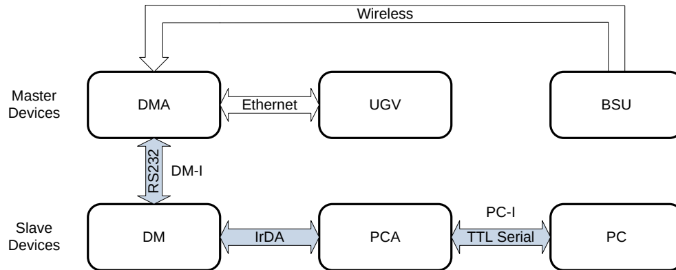
Figure 9. Communications flow. The Ethernet interface is subject to change as required by the UGV. Shaded arrows signify communications using the AIC protocol.
