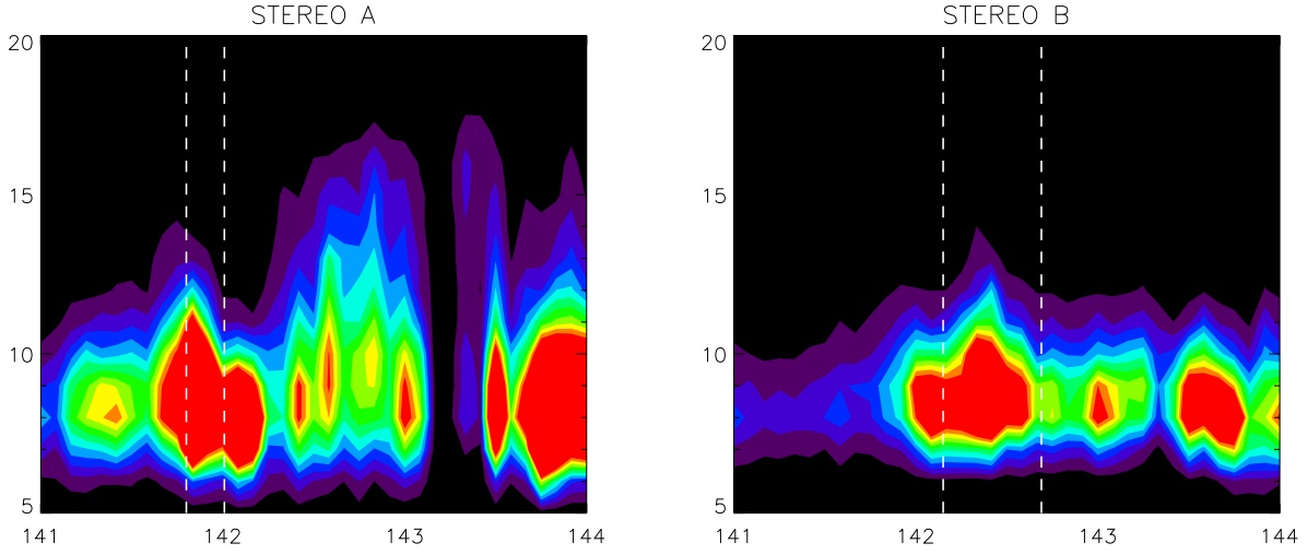
Fig. 1.— Fe charge state distributions detected by STEREO A and B during the 2007 May 19 CME passage. Highest Fe charge states are detected by STEREO A, though the magnetic cloud is more clearly detected in STEREO B. Magnetic field and other data indicate cloud passage between 3:36 hr and 16:34 hr on day 142 (22 May) for STEREO B and 21 May 19:12 until 22 May 00:14 for STEREO A (Liu et al. 2008). The dashed vertical white lines show the temporal extent of the magnetic cloud (or flux rope) in this event.
