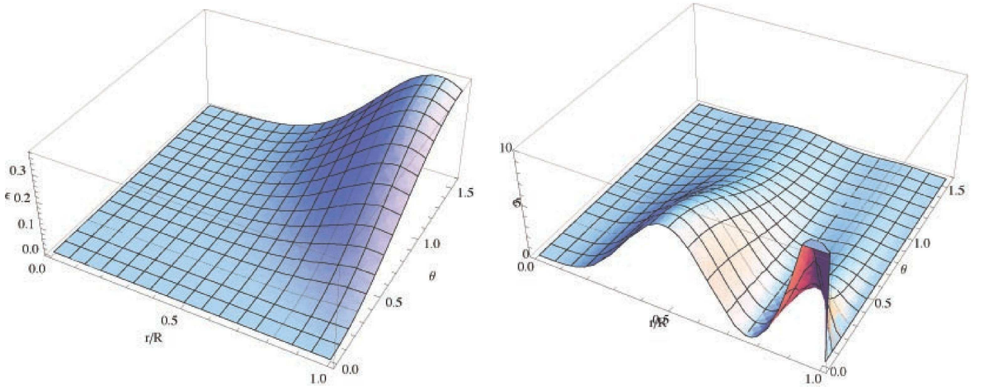
Fig. 3.— Normalized dissipation rate \epsilon as function of radial distance r/R(t) and polar angle \theta for two self-similar dissipative structures, m=1 . Left Panel: solutions (5-6). Right Panel: solutions (7-8).
