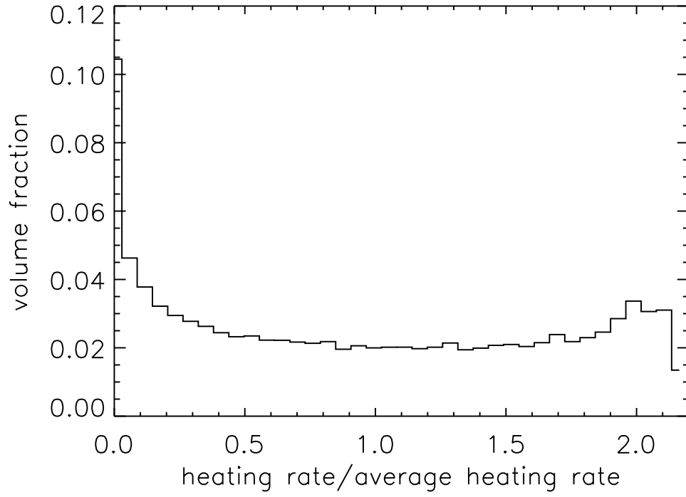
Fig. 4.— Distribution of volumetric heating rates in the spheromak model of the first type, solution (5-6), in terms of the average heating rate over the whole volume.
