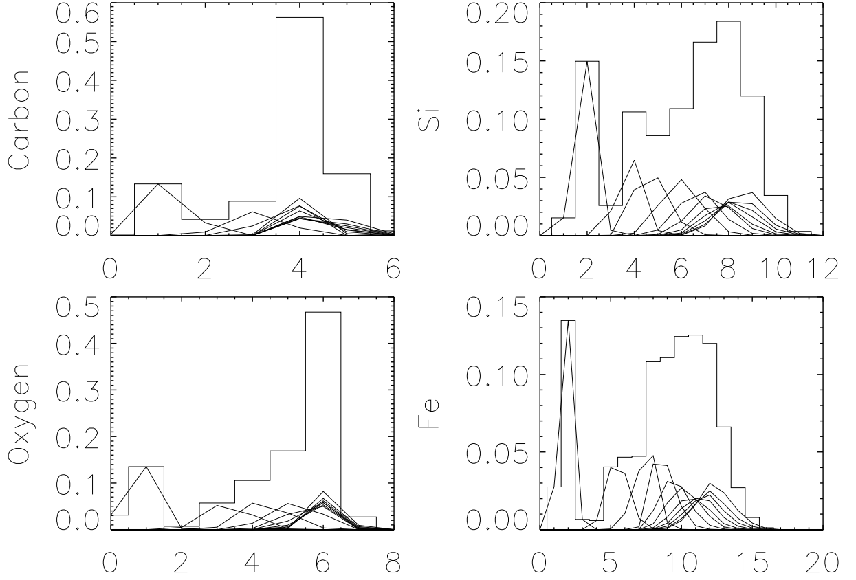
Fig. 5.— Final charge state distributions of C, O, Si and Fe for model 1. The individual lines show the contributions from regions within the spheromak with different heating rates. The histograms show the cumulative charge distribution assuming a volume weighted summation.
