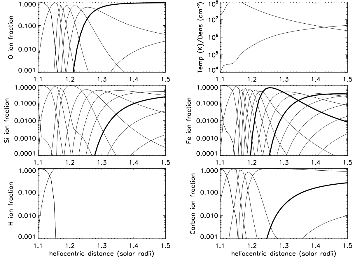
Fig. 6.— Evolution of charge state distributions for the highest anomalous resistivity considered in model 1 for H, C, O, Si, and Fe. Thick lines highlight \text{O}^{+6} , \text{Si}^{+9} , \text{Fe}^{+8} , \text{Fe}^{+11} , \text{C}^{+5} .
