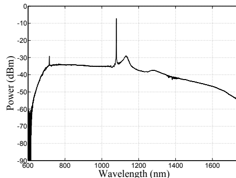
Figure 8: SC generated in the PCF-LMA-8 in OPG configuration at a pump peak power of 3 kW. The spectrum shows a sharp feature at 715 nm, together with features at the pump (1079 nm) and Raman Stokes (1131 nm) wavelengths. The OSA spectral resolution is 1 nm.
