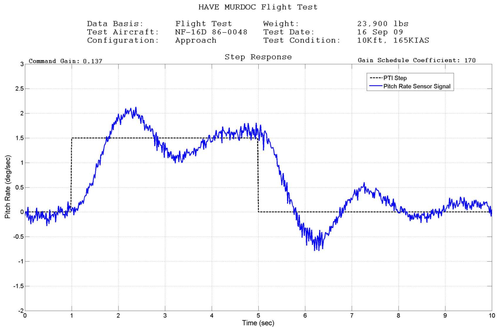
Figure C-35: Step (10K, 165KIAS)
