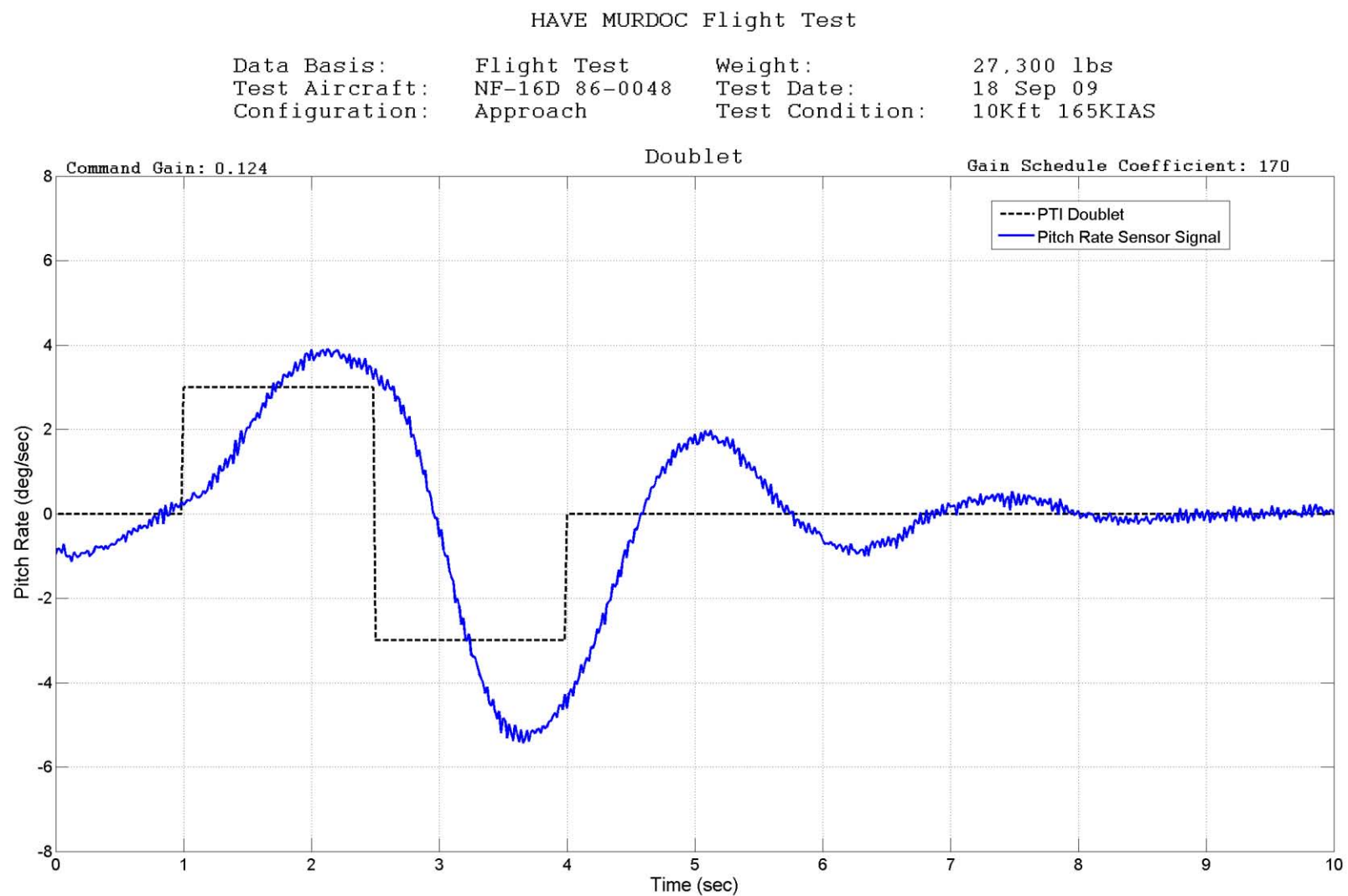
Figure C-21: Doublet (10K, 165KIAS)
