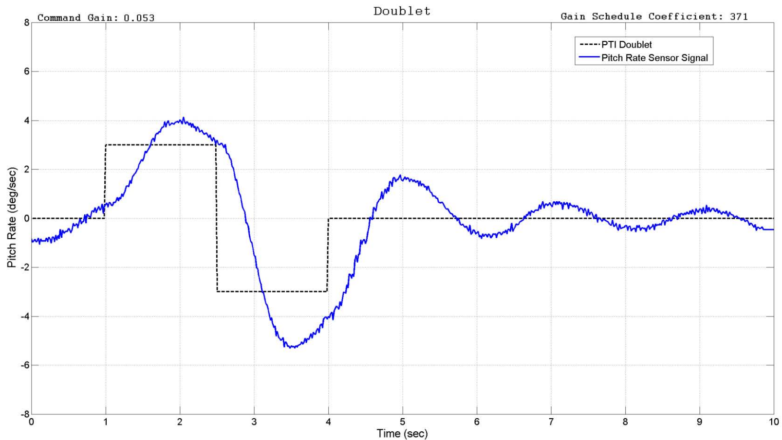
Figure C-15: Doublet (20K, 0.8 Mach)
