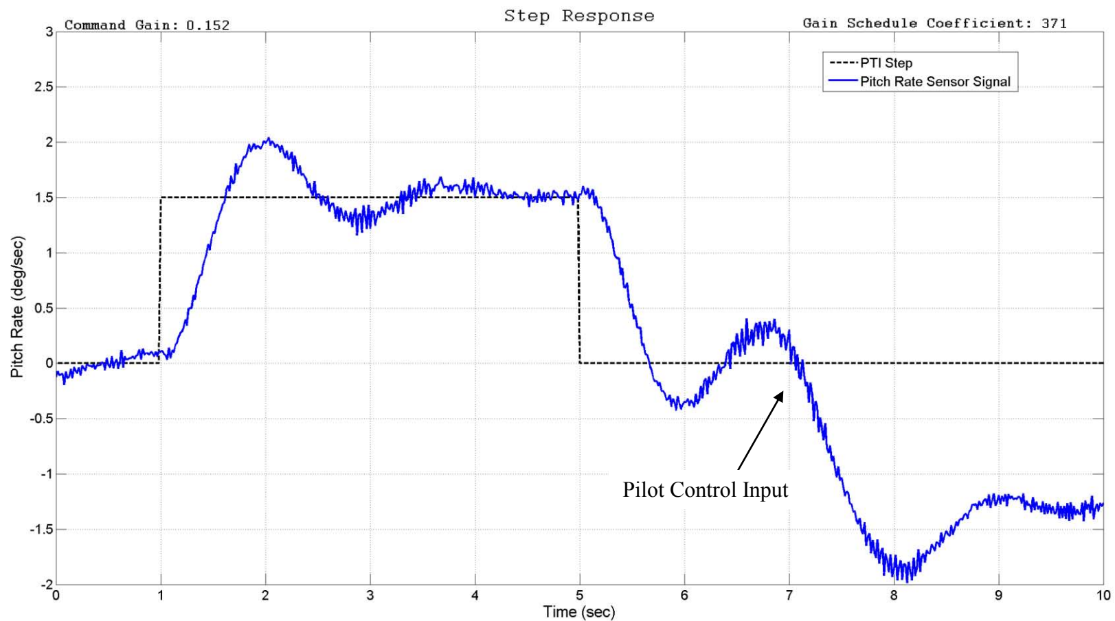
Figure C-29: Step (10K, 0.4 Mach)
