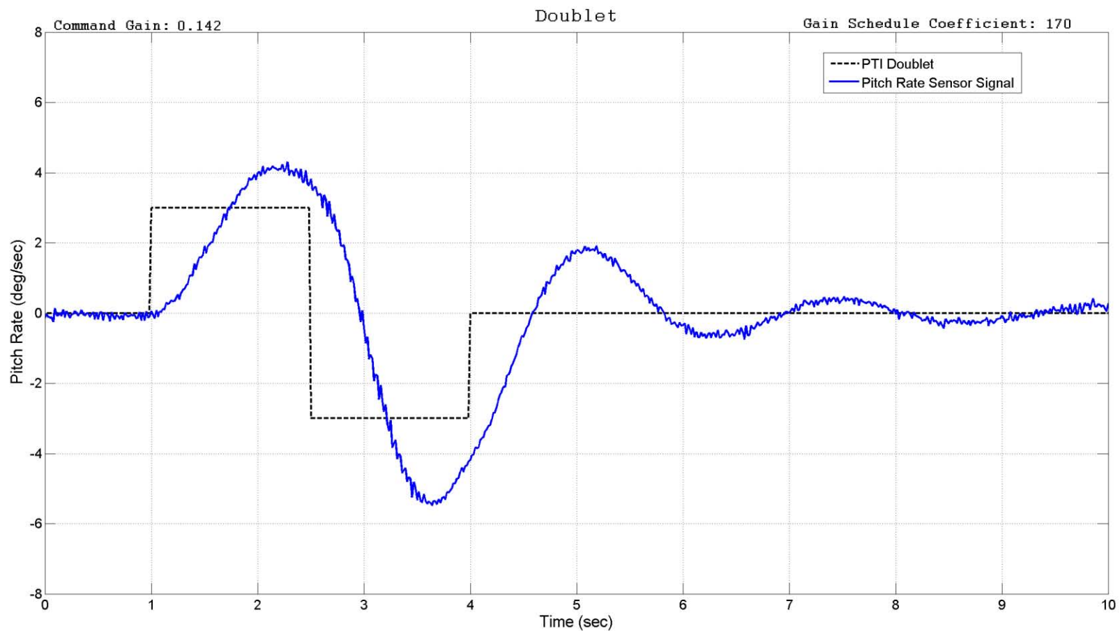
Figure C-17: Doublet (10K, 160KIAS)
