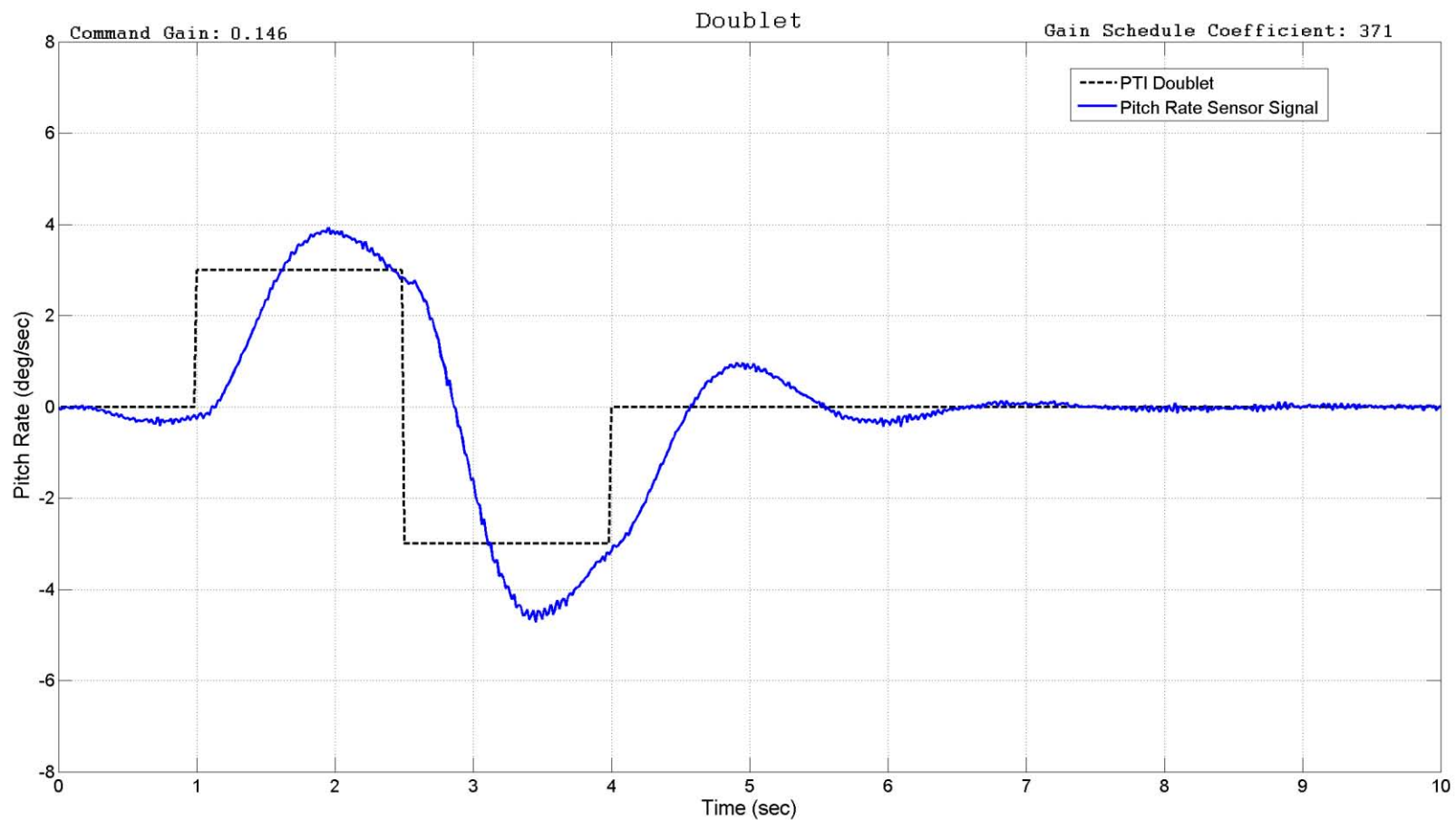
Figure C-8: Doublet (10K, 0.4 Mach)
