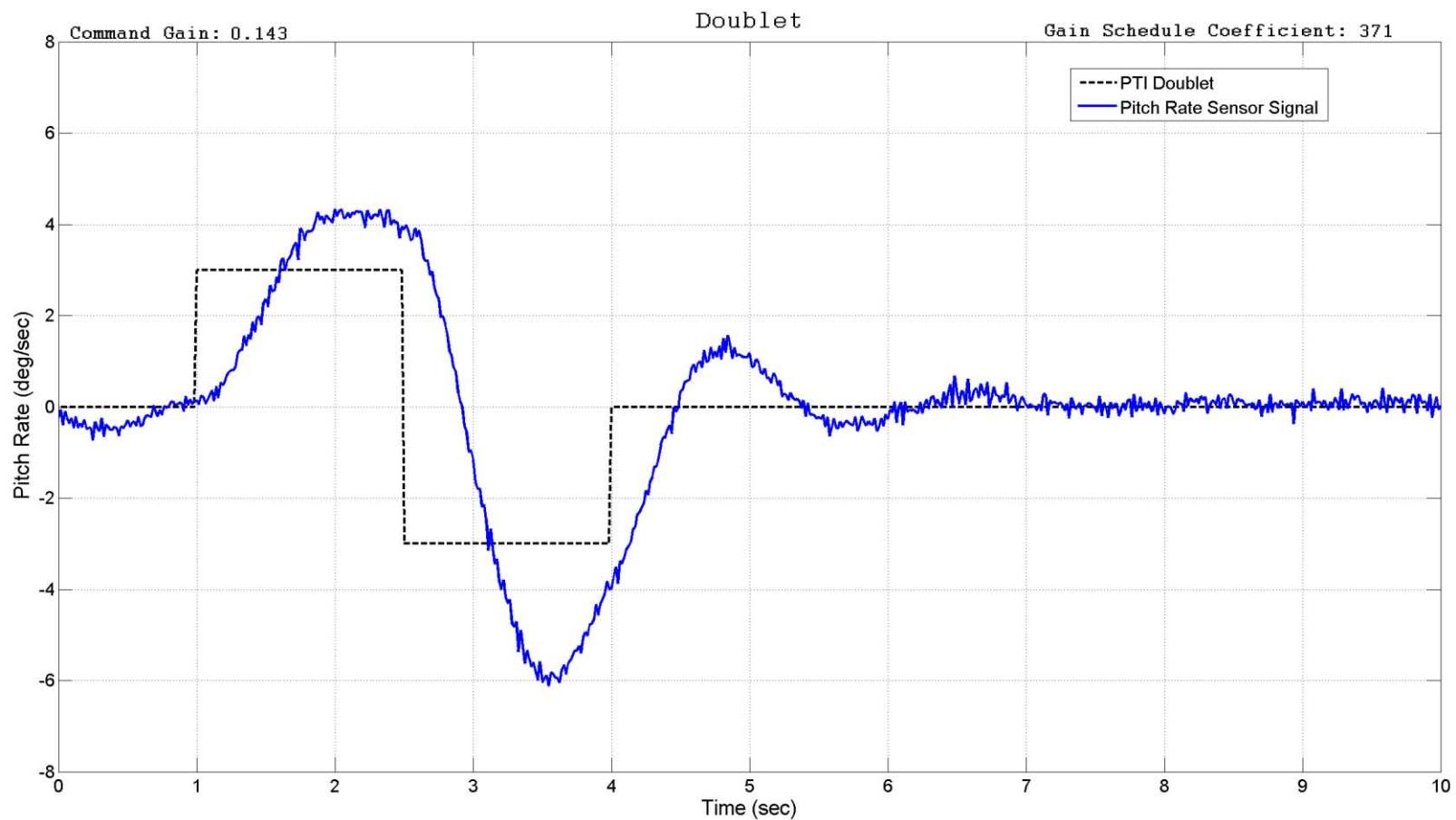
Figure C-25: Doublet (10K, 220KIAS)
