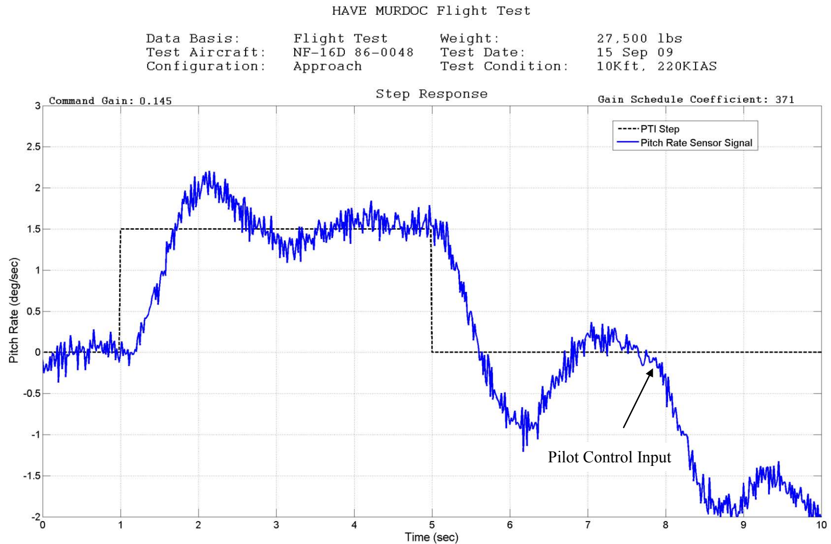
Figure C-36: Step (10K, 220KIAS)
