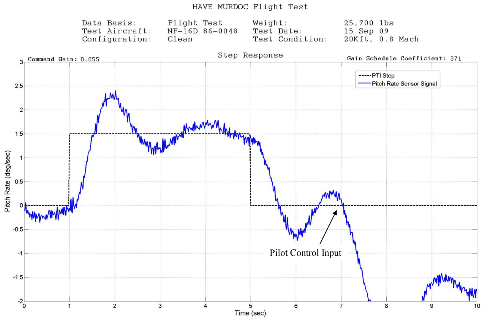
Figure C-32: Step (20K, 0.8 Mach)
