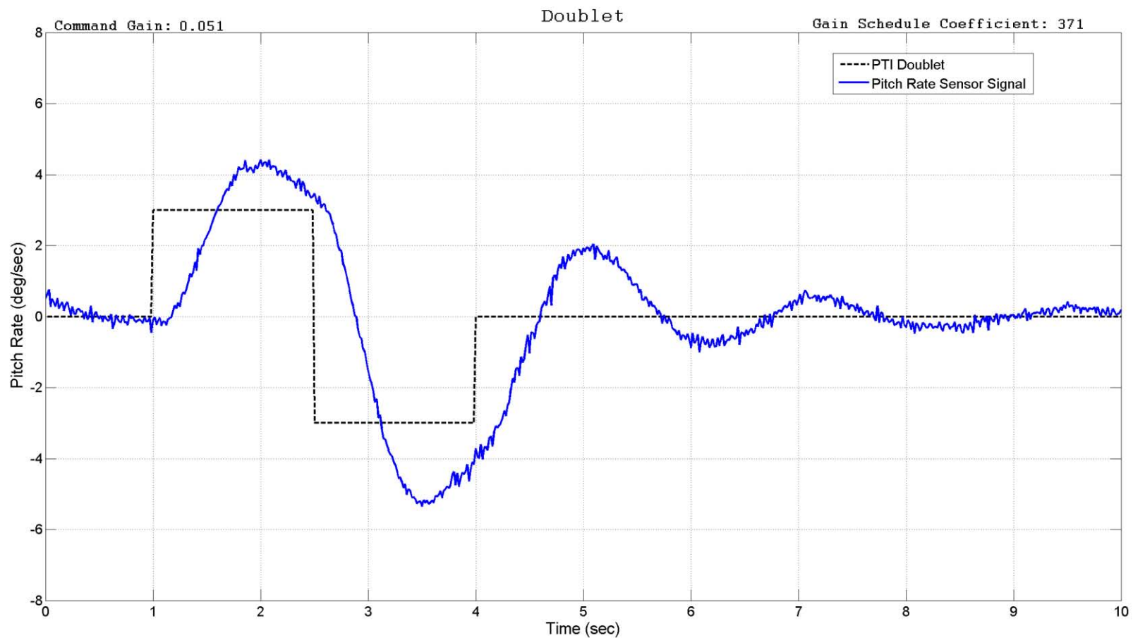
Figure C-16: Doublet (20K, 0.8 Mach)
