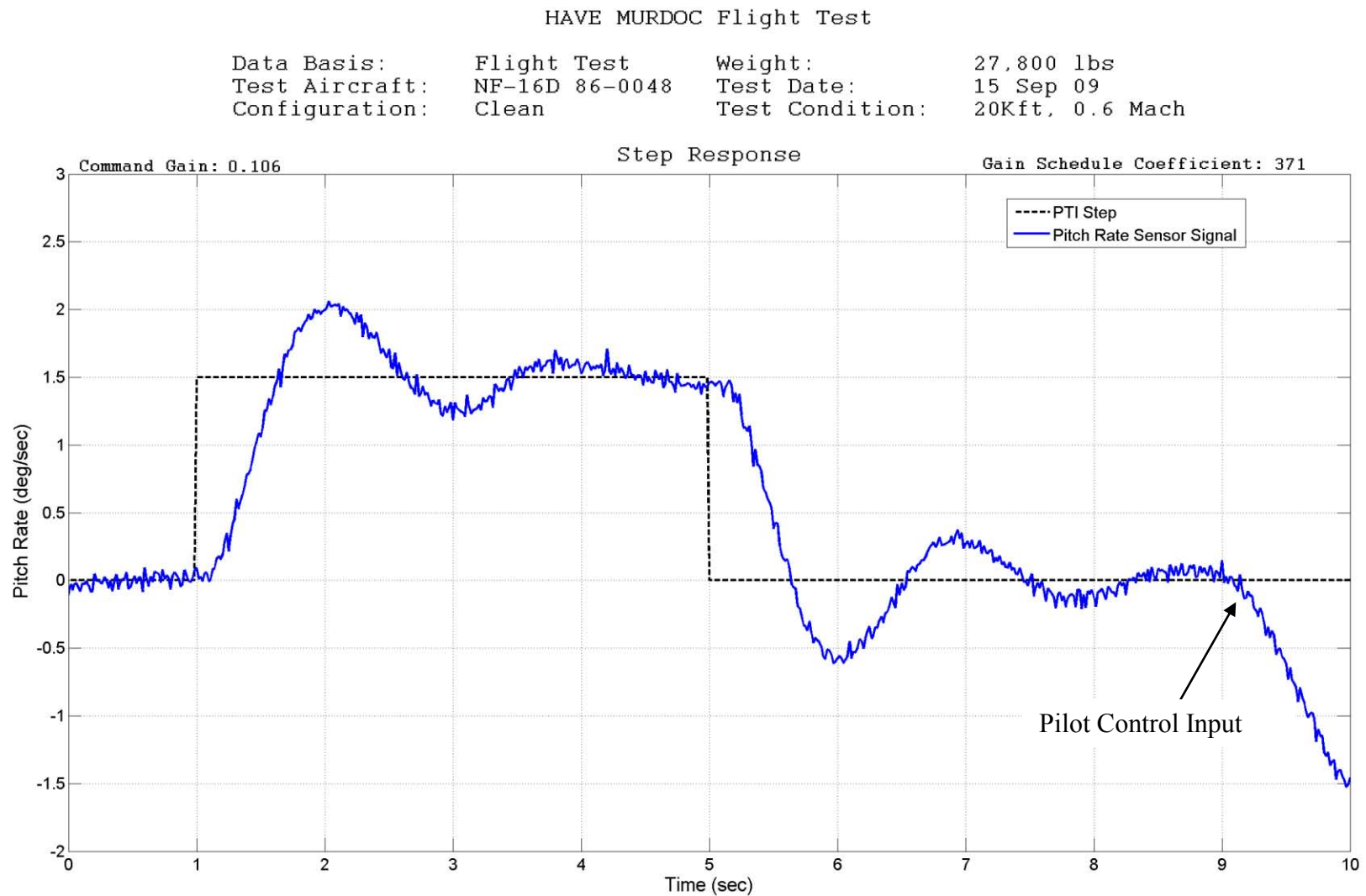
Figure C-31: Step (20K, 0.6 Mach)
