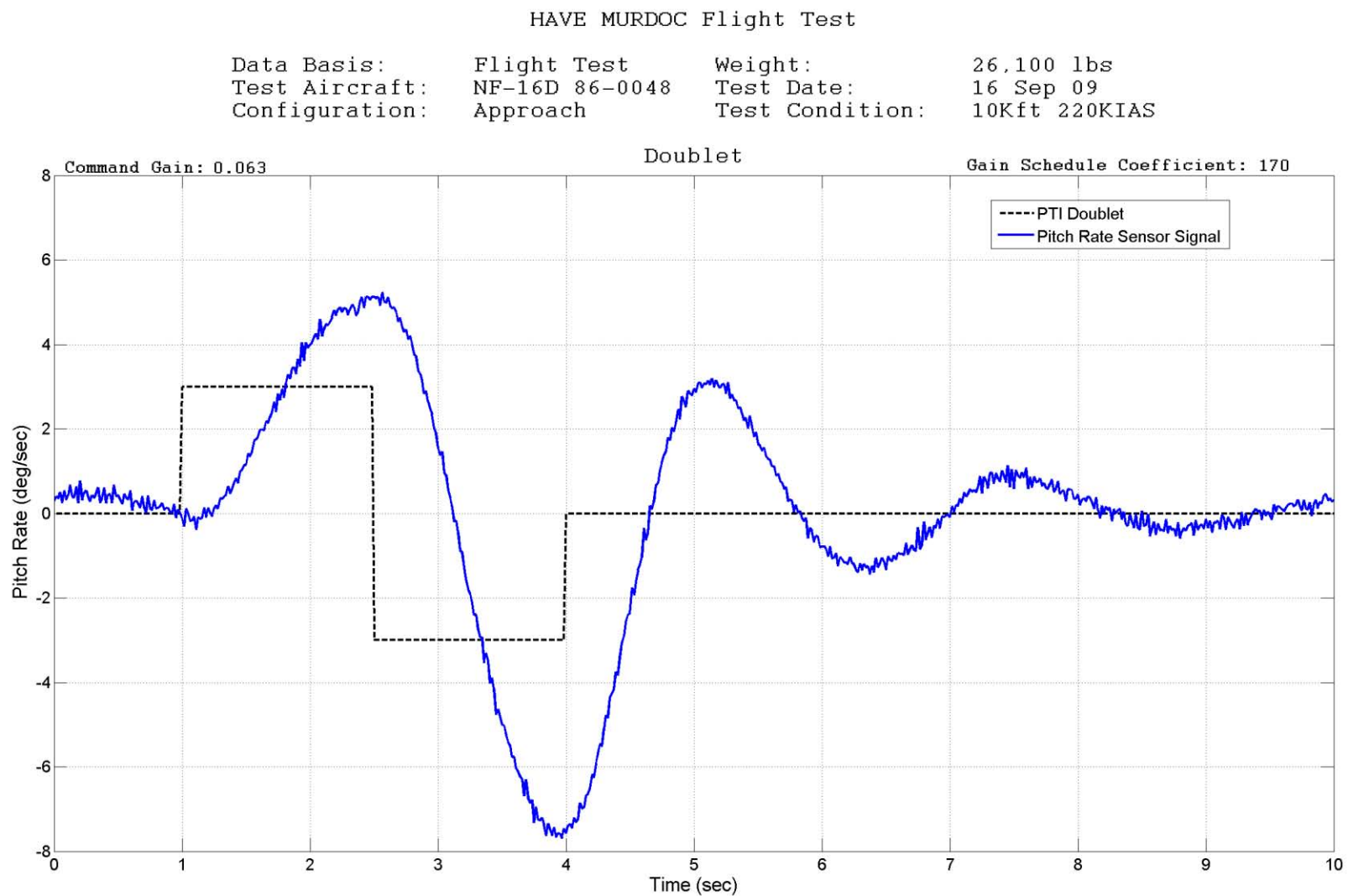
Figure C-27: Doublet (10K, 220KIAS)
