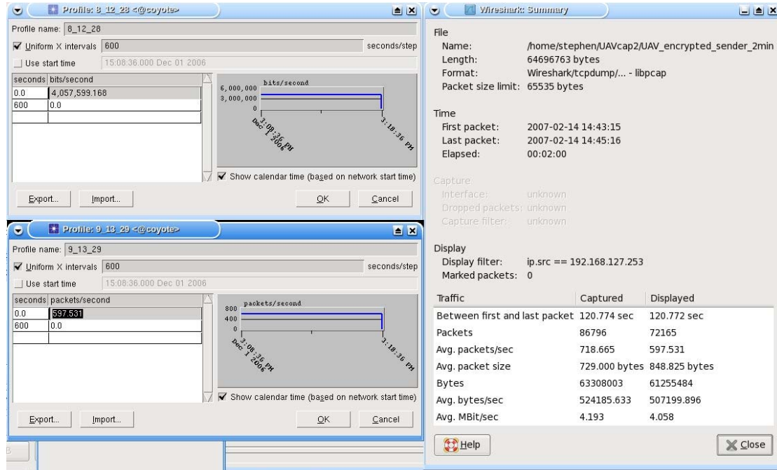
Figure 5. Wireshark traffic capture.
