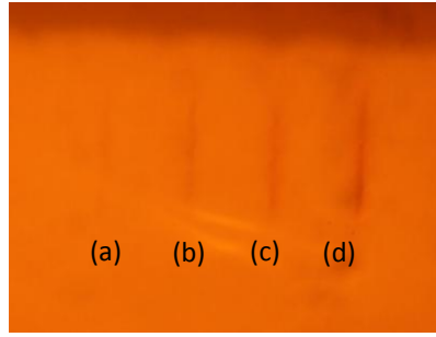
Figure 5. Optical micrograph of sample end facet displaying asymmetric modification of ZnSe with multiscan technique. (a) 1.5 mm.s-1, (b) 1 mm.s-1, (c) 0.5 mm.s-1, (d) 0.25 mm.s-1. The field view is 600 \mu\text{m} x 200 \mu\text{m} .
