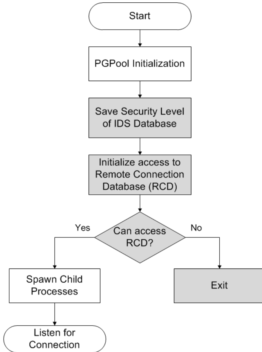
Figure 8. PGPool-II startup
