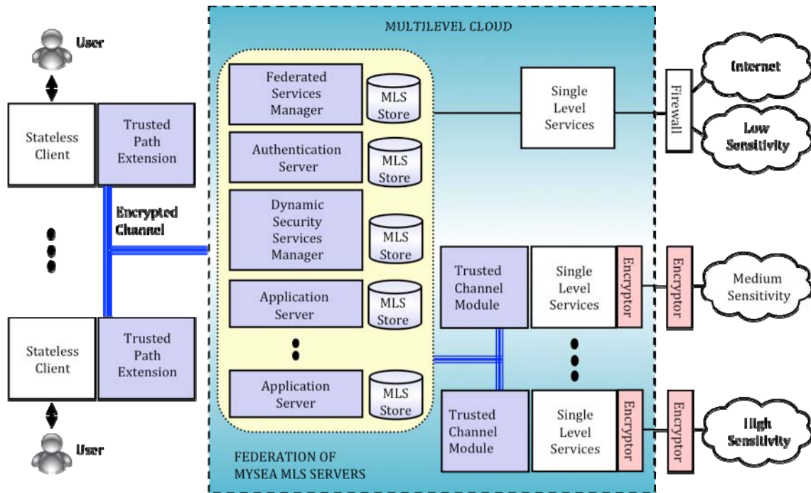
Figure 1. MYSEA environment
