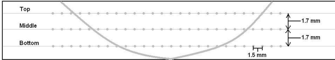
Figure 4. Depiction of the grid pattern used for microhardness testing. Gray curved line represents SZ general shape.
