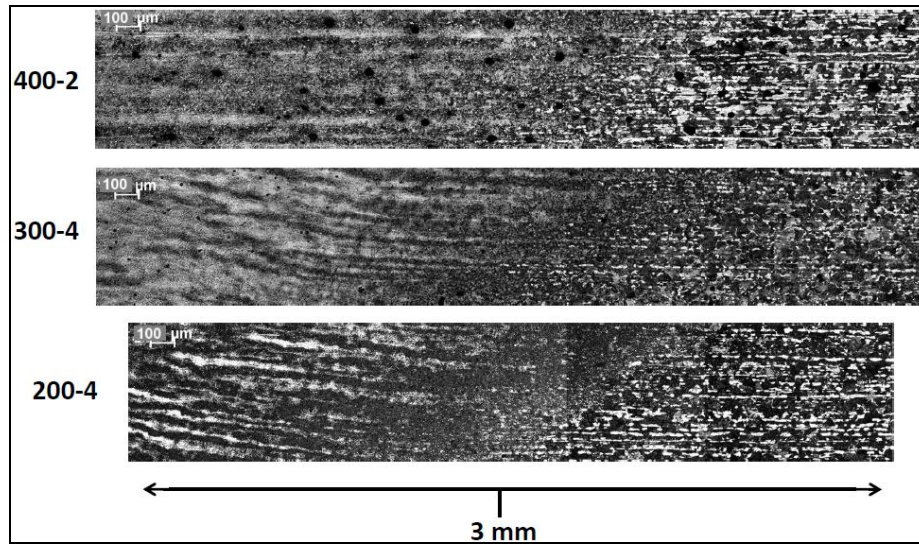
Figure 11. Optical micrographs showing different RPM (wet) FSP bead TMAZs. The advancing side is on the right side of the montages and the direction of tool travel is into the page.
