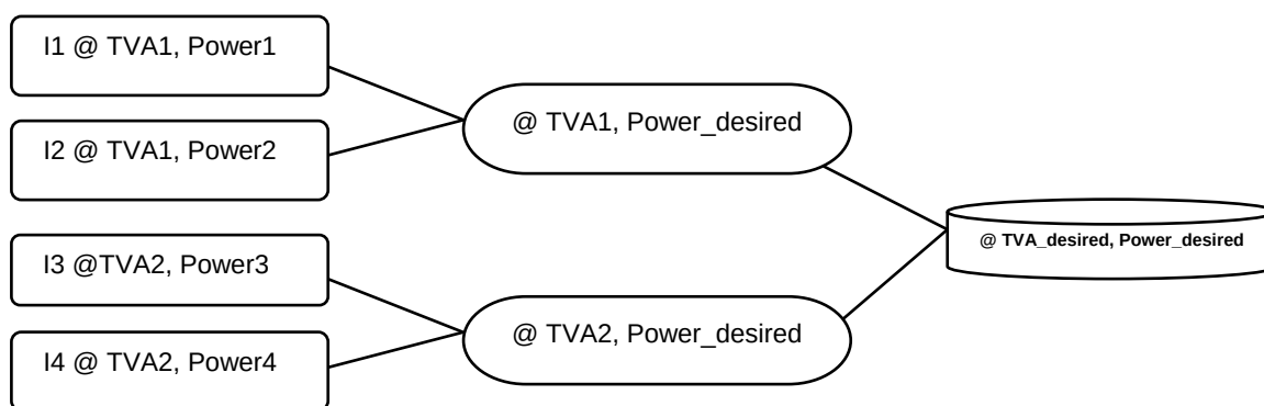
Figure 2-21. Interpolation Procedure for Fixed Wing Aircraft
