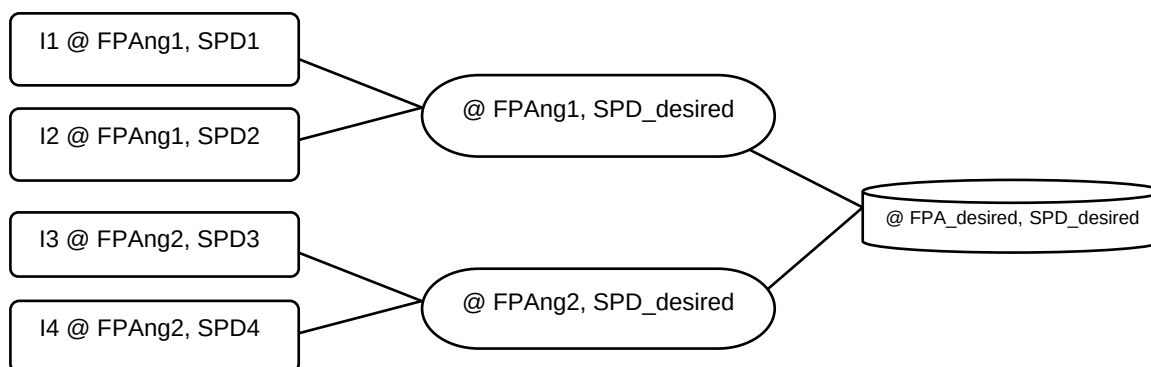
Figure 2-19. Interpolation Procedure
