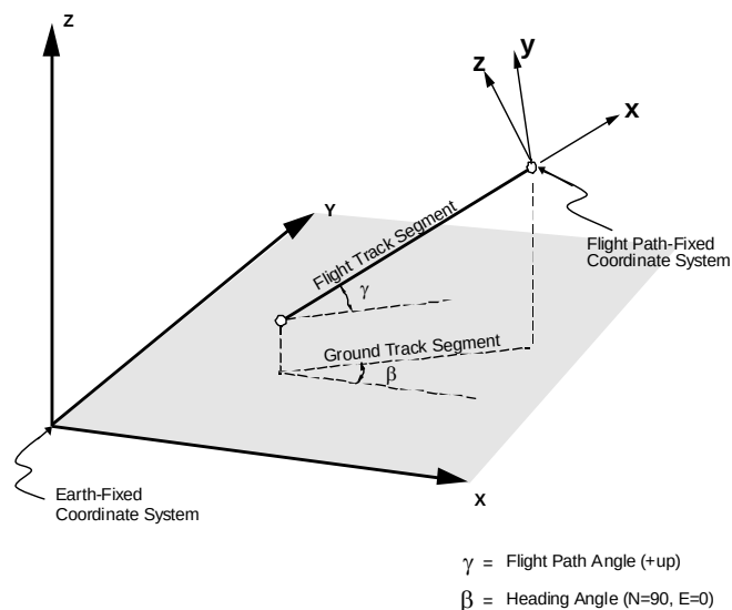
Figure 2-10. Earth-Fixed and Flight Path-Fixed Coordinate Systems
