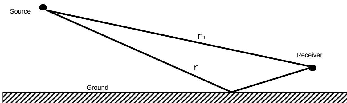
Figure 2-5. Ground Attenuation Geometry: Direct and Reflected Rays
