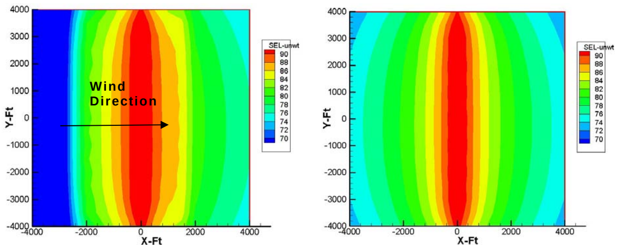
Figure 2-7. Weather Effect on Noise with and without Winds
