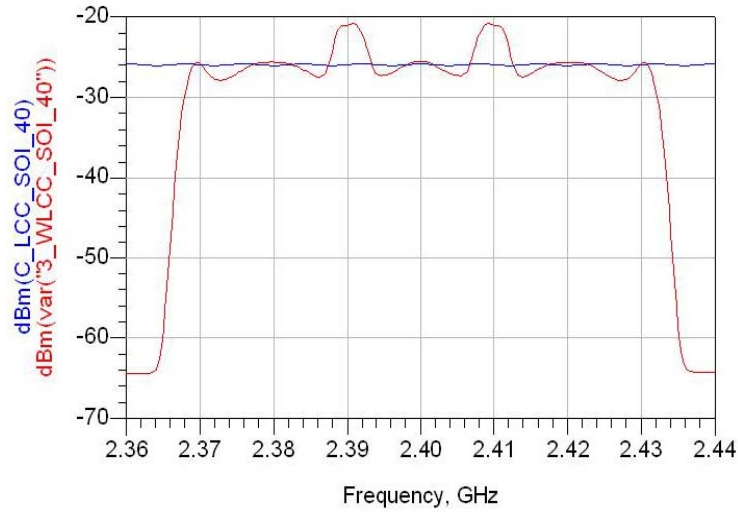
Figure 115. Amplitude Plot of SOI for both WLCC and LCC with Non-Ideal Component Parameter Settings in dBm with 40 \Omega Load.
