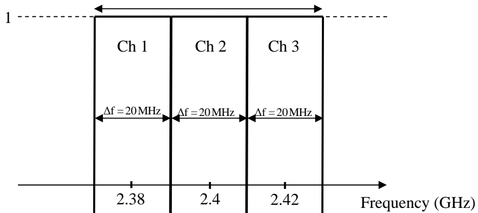
Figure 28. Ideal Transfer Function of a Three-Channel FDMC.
