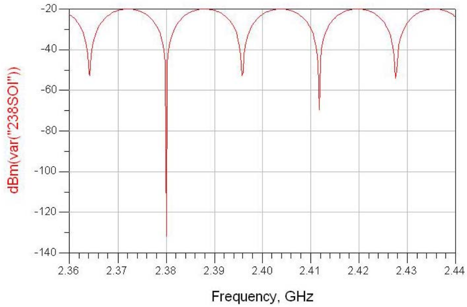
Figure 13. Amplitude Plot of SOI for l = 18.908 m.
