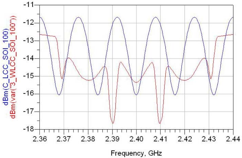
Figure 114. Amplitude Plot of SOI for both WLCC and LCC with Non-Ideal Component Parameter Settings in dBm with 100 Ω Load.
