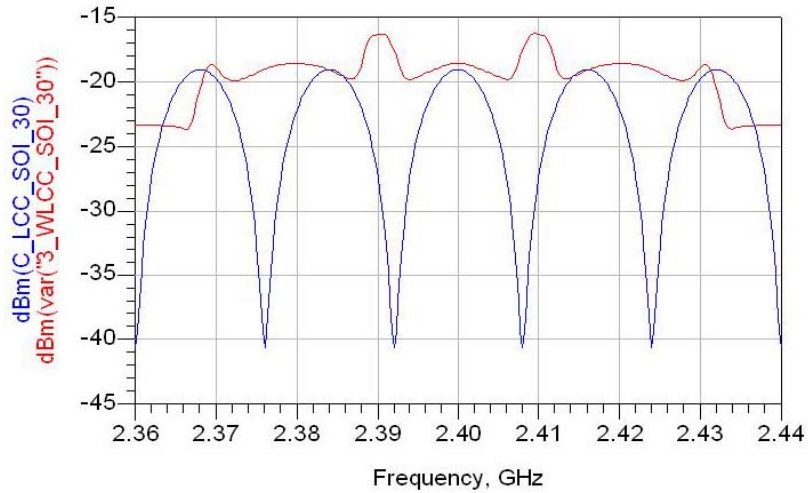
Figure 116. Amplitude Plot of SOI for both WLCC and LCC with Non-Ideal Component Parameter Settings in dBm with 30 \Omega Load.
