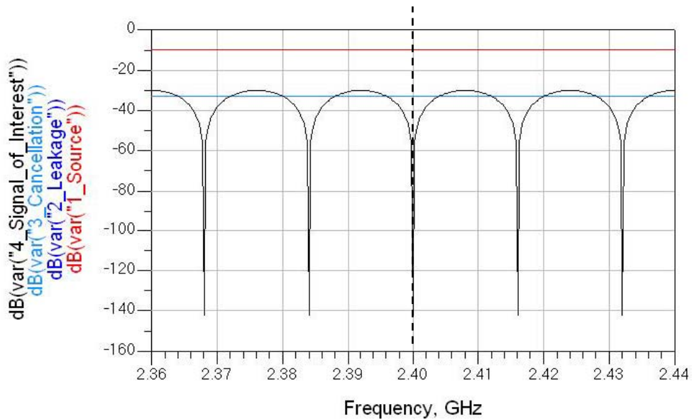
Figure 22. LCC Frequency-Domain Plots in dB.
