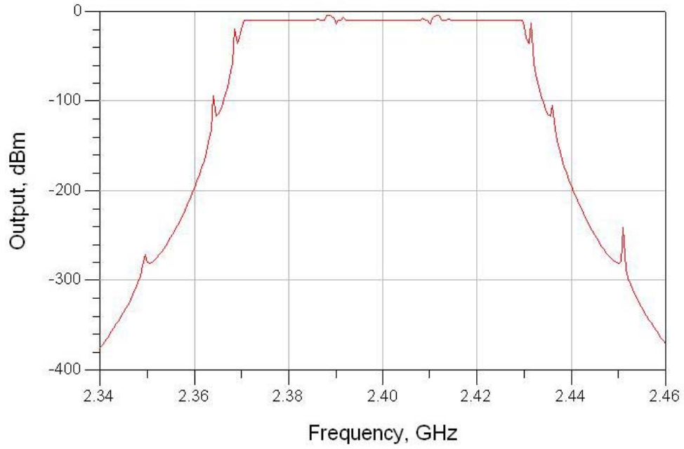
Figure 60. Output Amplitude Plot for the FDMC that uses Couplers and Butterworth Filters.
