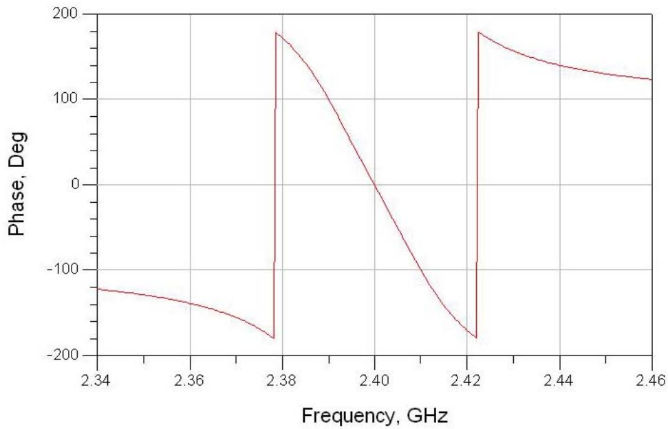
Figure 45. Output Phase Plot for the Bessel BPF.
