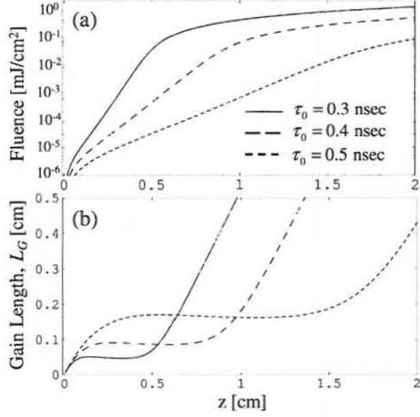
Figure 2: (a) UV fluence as a function of propagation distance, z , for heating pulses with \lambda_o = 1 \mu\text{m} , I_o \tau_o = 285 \text{ J}/\text{cm}^2 and pulse durations \tau_o = 0.3, 0.4 , and 0.5 nsec. (b) Fluence gain length, L_G , as a function of z , corresponding to panel (a).
