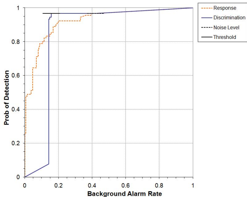
Figure 9. Saint/hand held blind grid probability of detection for response and discrimination stages versus their respective probability of background alarm.
