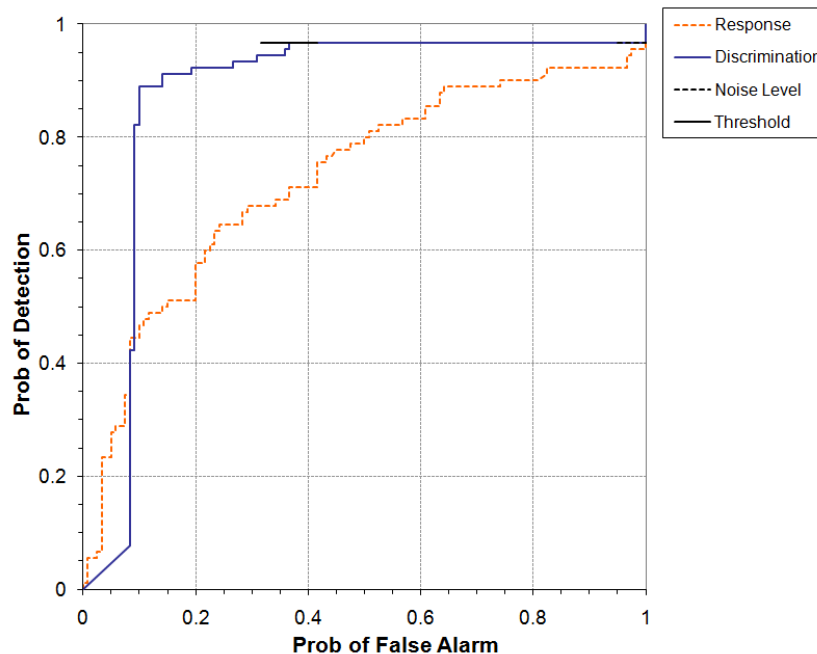
Figure 3. Saint/hand held blind grid probability of detection for response and discrimination stages versus their respective probability of false positive.
