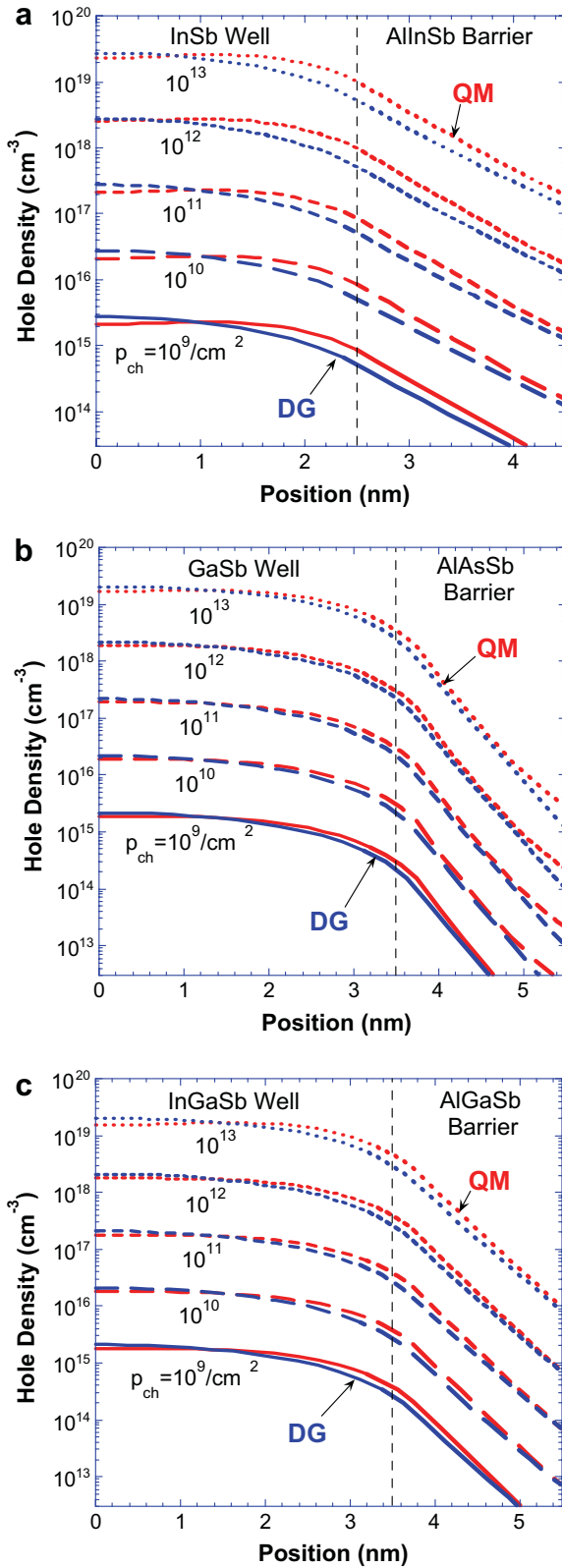
Fig. 3. (a–c) Density profiles across the quantum wells studied in this paper as simulated by quantum mechanics and fit by DG theory. The perpendicular components of the DG effective masses as determined by these fits are given in Table 2.
