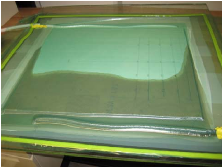
Figure 3. Resin flowing through the layup
