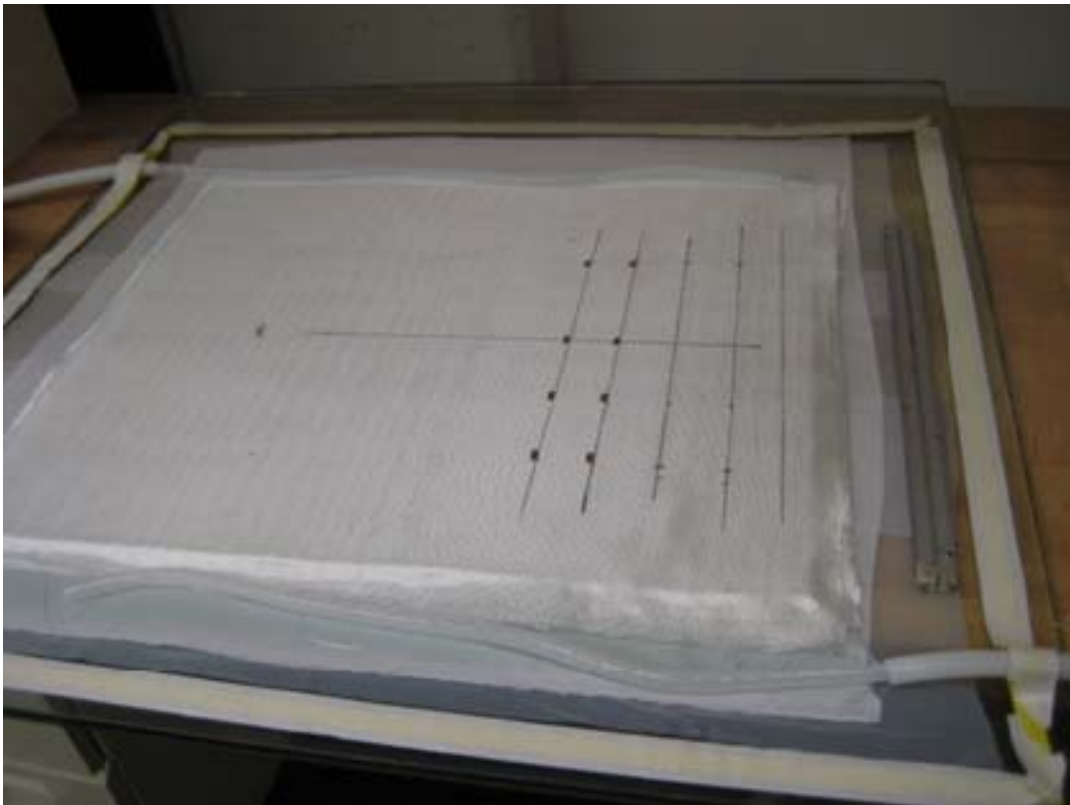
Figure 5. Strain gage placement on dry layup
