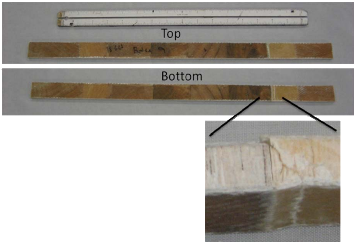
Figure 12. Dry impact damage with core shearing. The rightmost fracture line was right at the edge of the clamped boundary.
