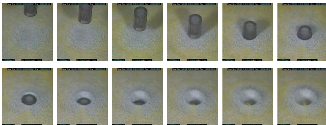
Fig.8 High-speed visualization of detailed behavior of projectile during penetration.
