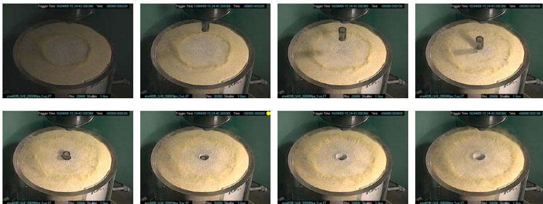
Fig.7 High-speed visualization of behavior of projectile during penetration.
