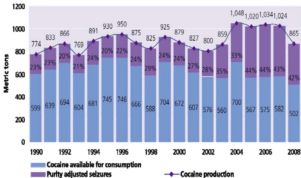
Figure 5. Cocaine Production, Seizures, and Supply to Markets, 1990–2008. 208
