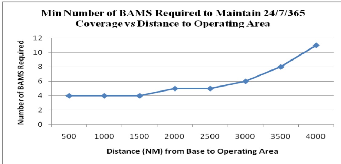
Figure 14. Minimum Number of BAMS Required Versus Distance to Operating Area
