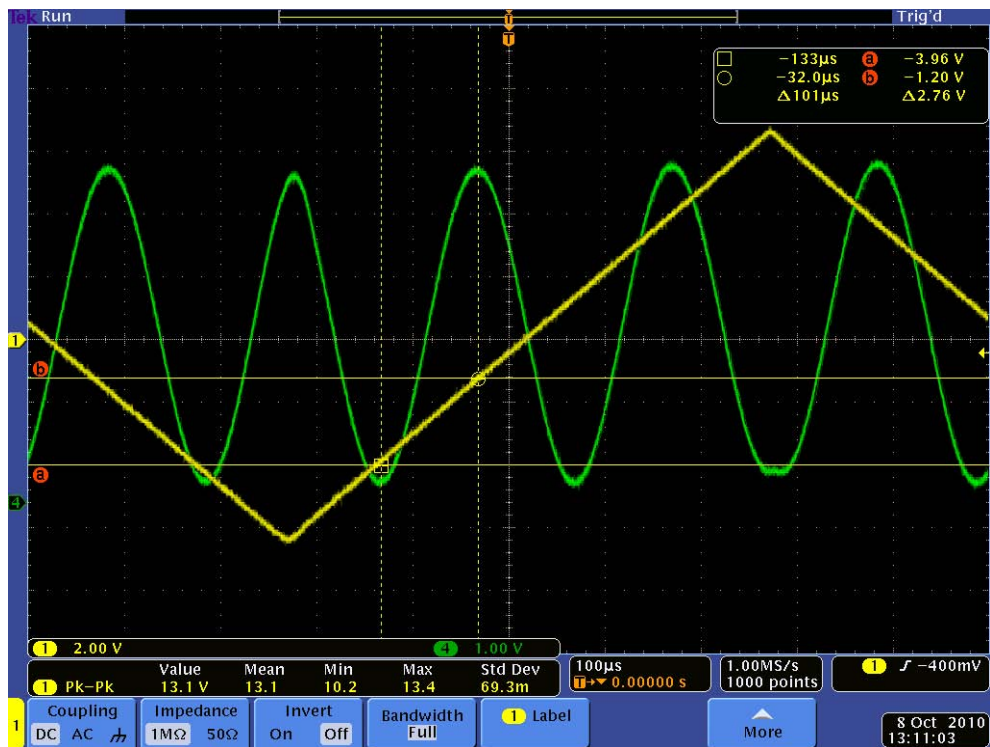
Figure 19. Aligned RSNS waveform for mod 9 (channel 3).
