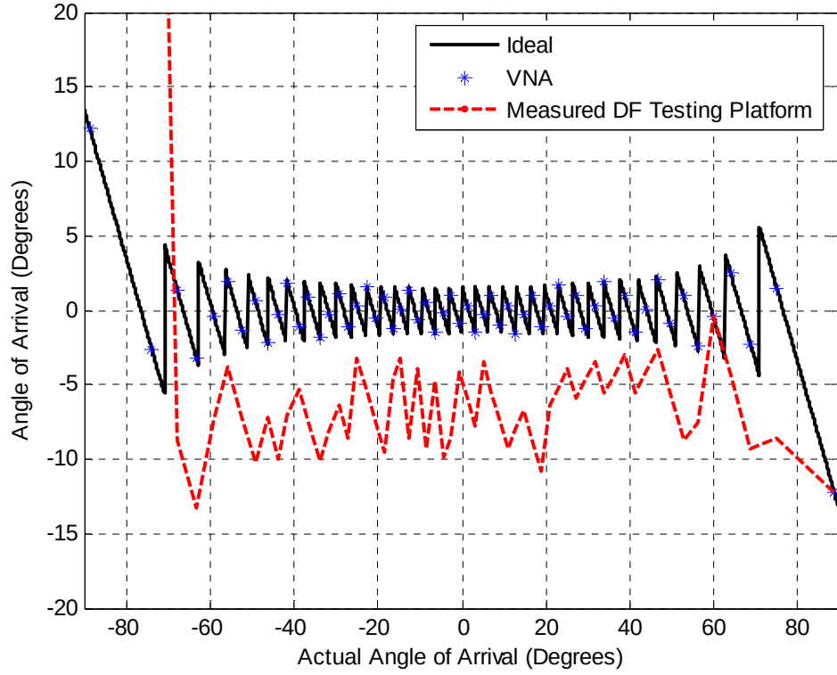
Figure 43. Comparisons of AOA errors from ideal, mesaured DF testing platform and VNA.
