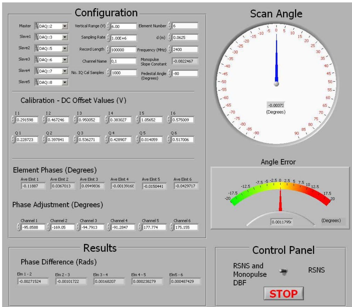
Figure 54. Front panel of the tracking module.
