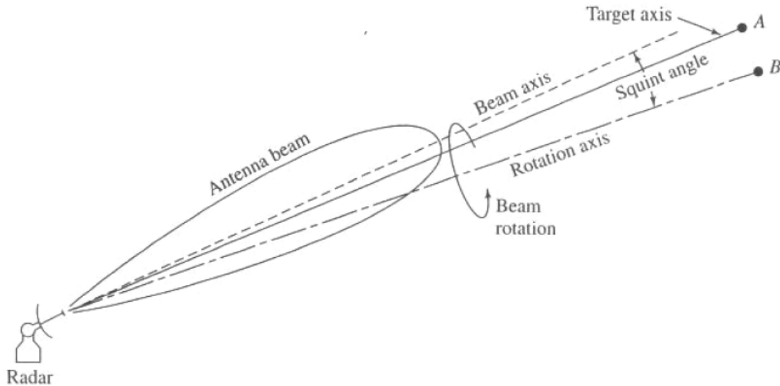
Figure 15. Scan structure of conical scan (from [4]).
