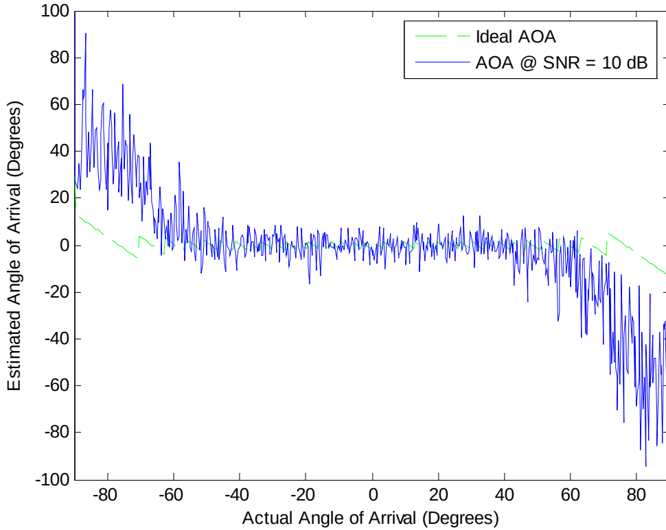
Figure 44. AOA error for noiseless and for SNR = 10 dB.
