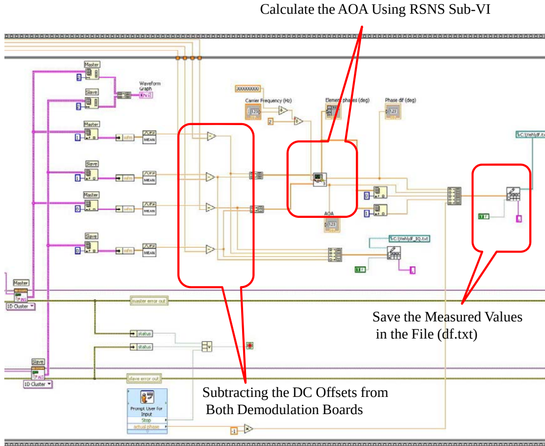
Figure 36. The second portion of the DF block diagram (after [10]).
