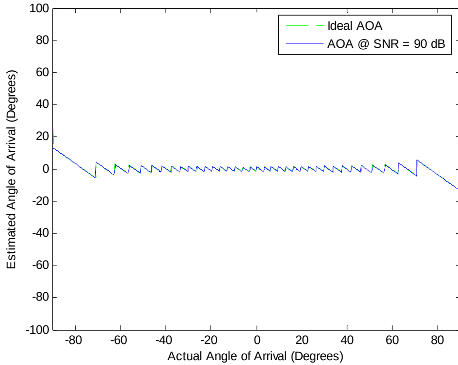
Figure 48. AOA error for noiseless and for SNR = 90 dB.
