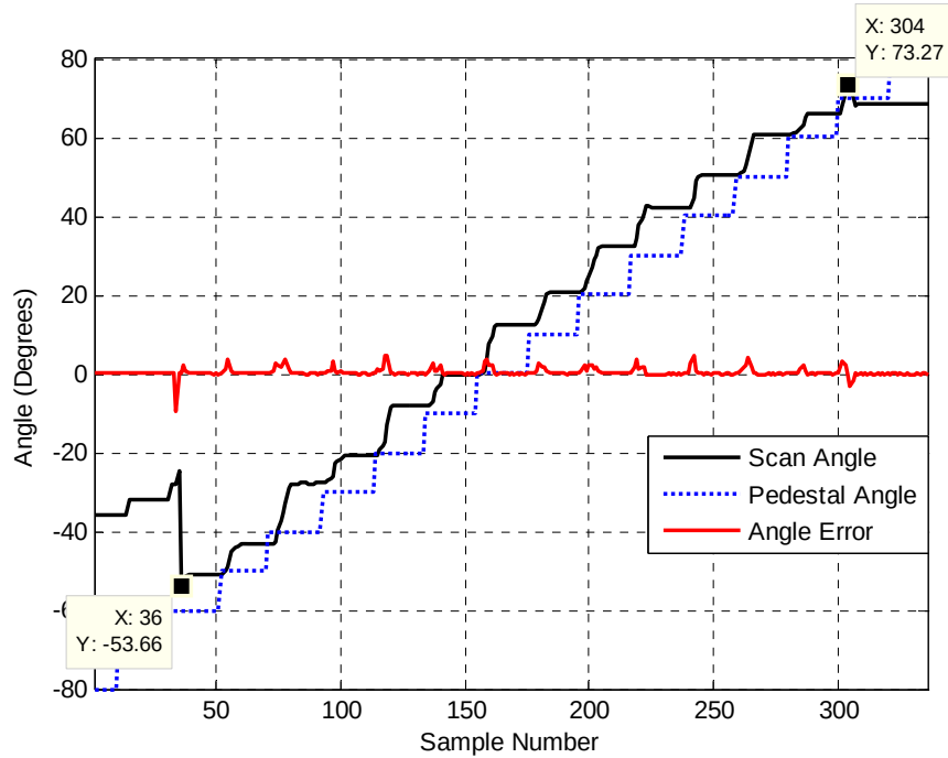
Figure 81. Tracking with RSNS and monopulse DBF mode using five phase differences (elements 1-2, 2-3, 3-4, 4-5, 5-6) , 10 degree steps and 10^\circ angle error limitation.
