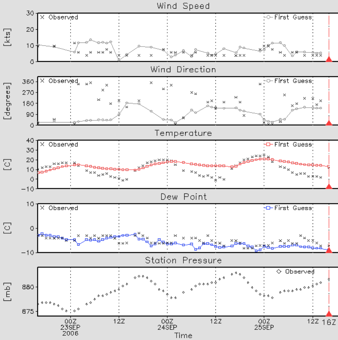
Fig. 4a. MetQC web page graphic for station KNFL (NAS Fallon) showing time series of observations and model forecasts. Station pressure forecasts were not processed.
