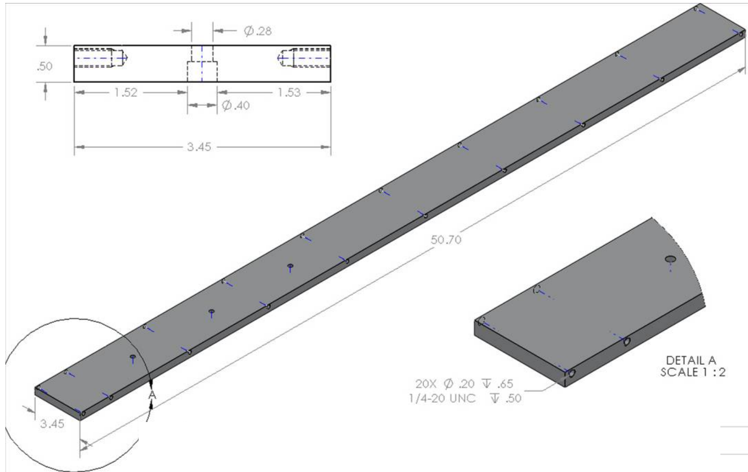
Figure 90. Insert bottom (1 of 2)
