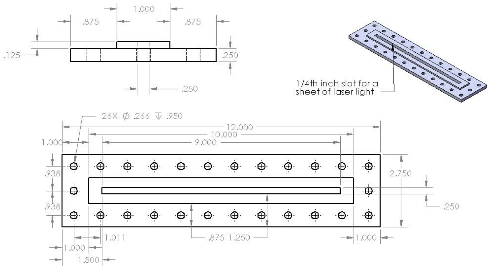
Figure 82. PIV Glass Holder
