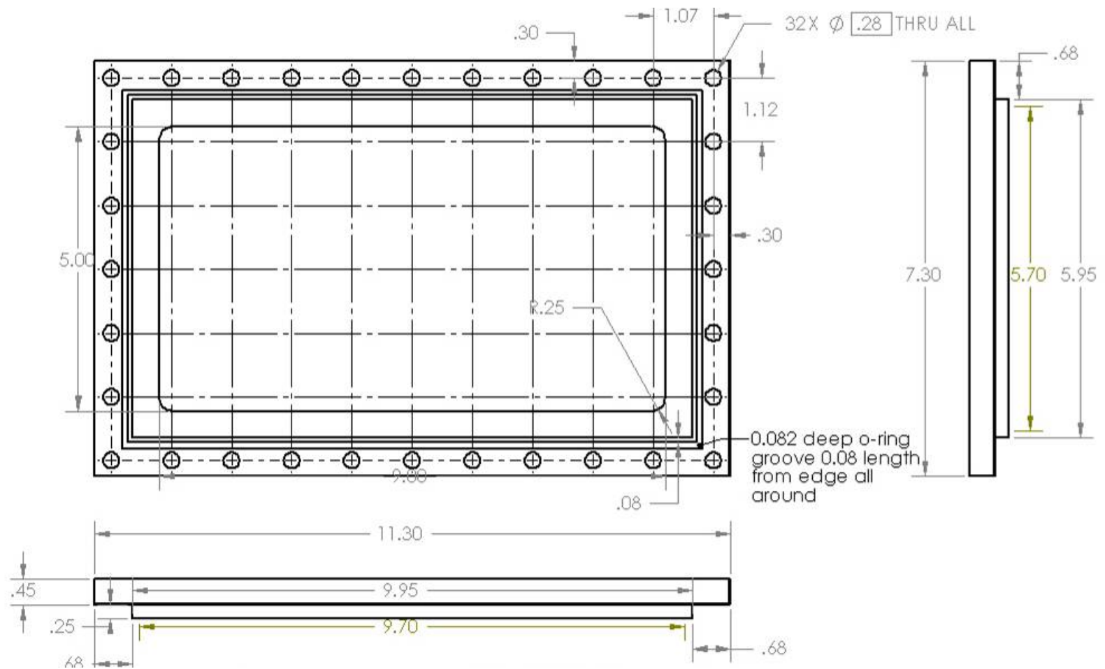
Figure 76. Glass Holder optical (2 of 2)
