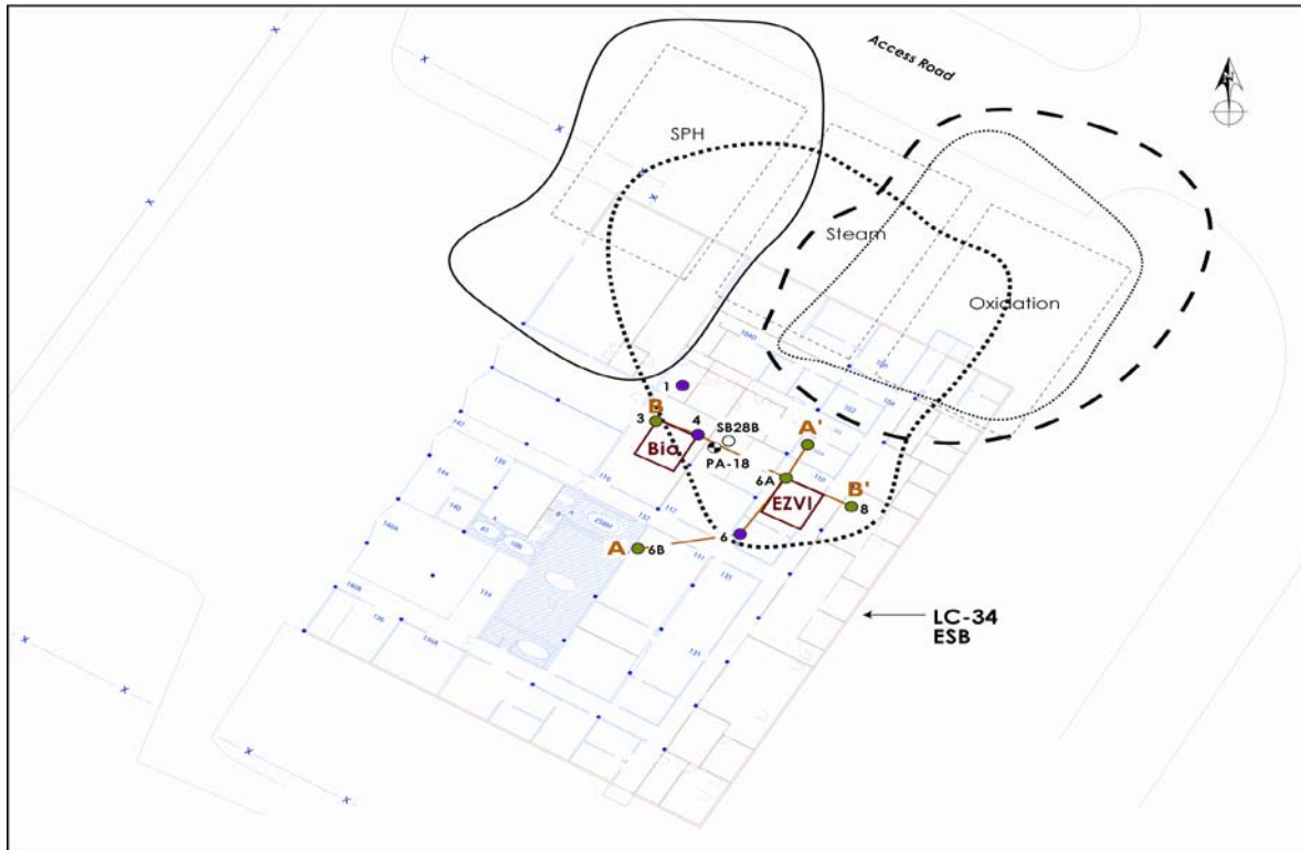
Figure 3. Site plan and technology demonstration locations at LC-34.
