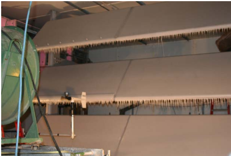
Figure 1.8. A large fan was used to generate wind loading on ice. The fan was located on the vertical centerline of the fins with the discharge directed at one of the fins. A Young anemometer was used to measure the wind speed during the test; for this test the average wind speed was 23 mph.
