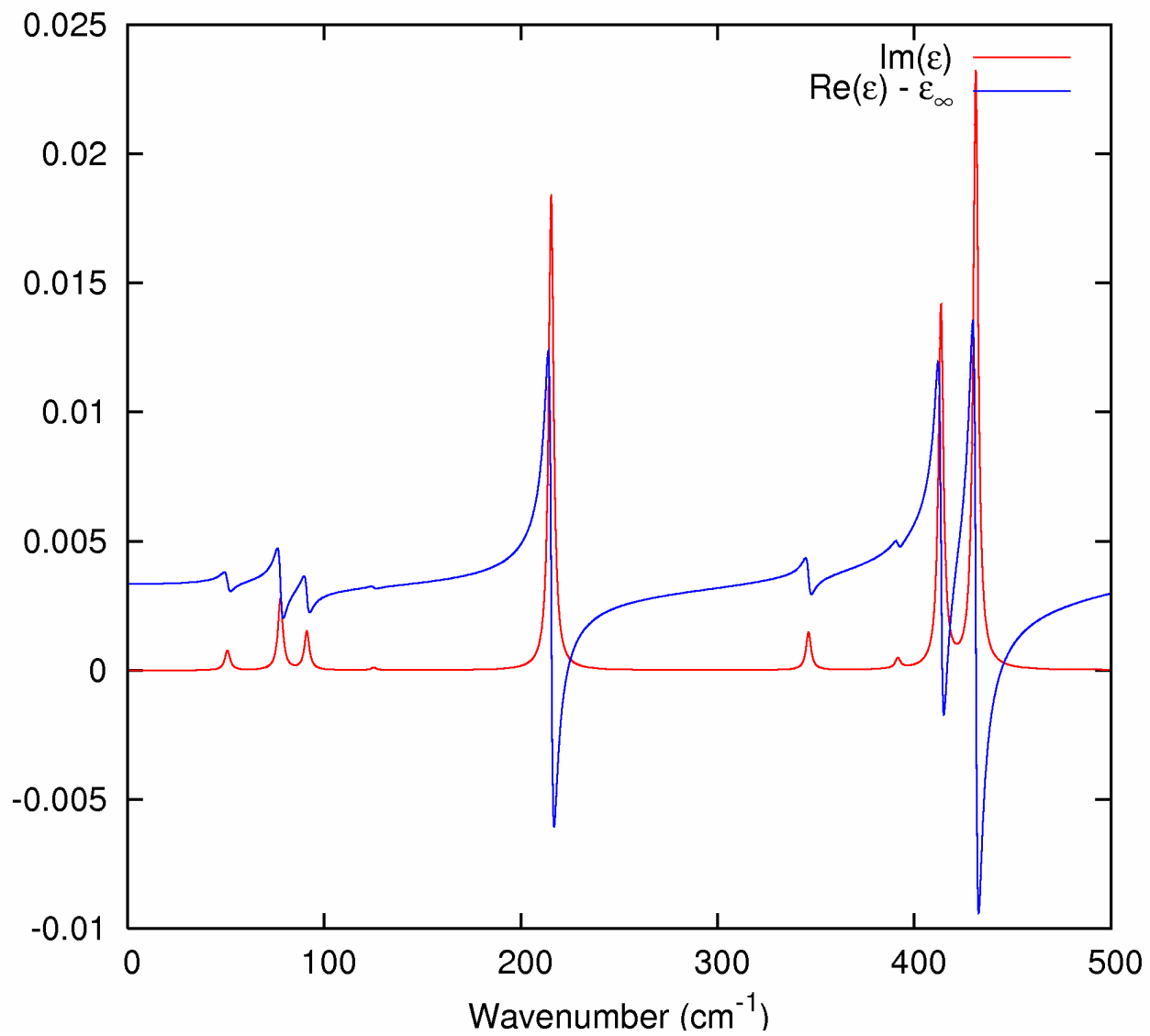
Figure 9. Real (blue) and imaginary (red) parts of permittivity function of RDX molecules with \gamma_n = 3 \text{ cm}^{-1} and \rho = 2.4 \cdot 10^{19} \text{ cm}^{-3} for frequencies within THz range.
