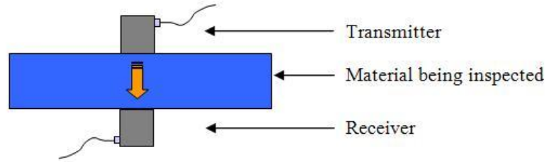
Figure 17 Schematic of through-transmission testing
