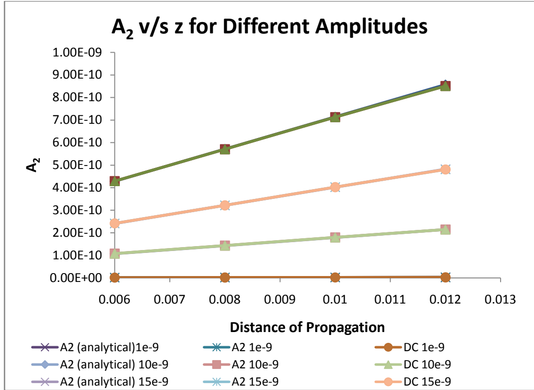
Figure 49 Variation of the Second Harmonic Amplitude and Static Displacement Component with Distance of Propagation for different Input wave amplitudes for f=5\text{MHz} , \beta=30
