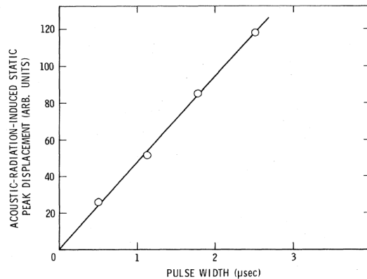
Figure 6 Acoustic Radiation Induced Static Peak Displacement as a function of Pulse width
