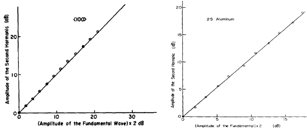
Figure 1 Amplitude change of Second Harmonic Wave as a function of Fundamental wave Amplitude (a) Aluminum Single Crystal <100> Direction (b) aluminum 2S polycrystal (Hikata et al (1965))
