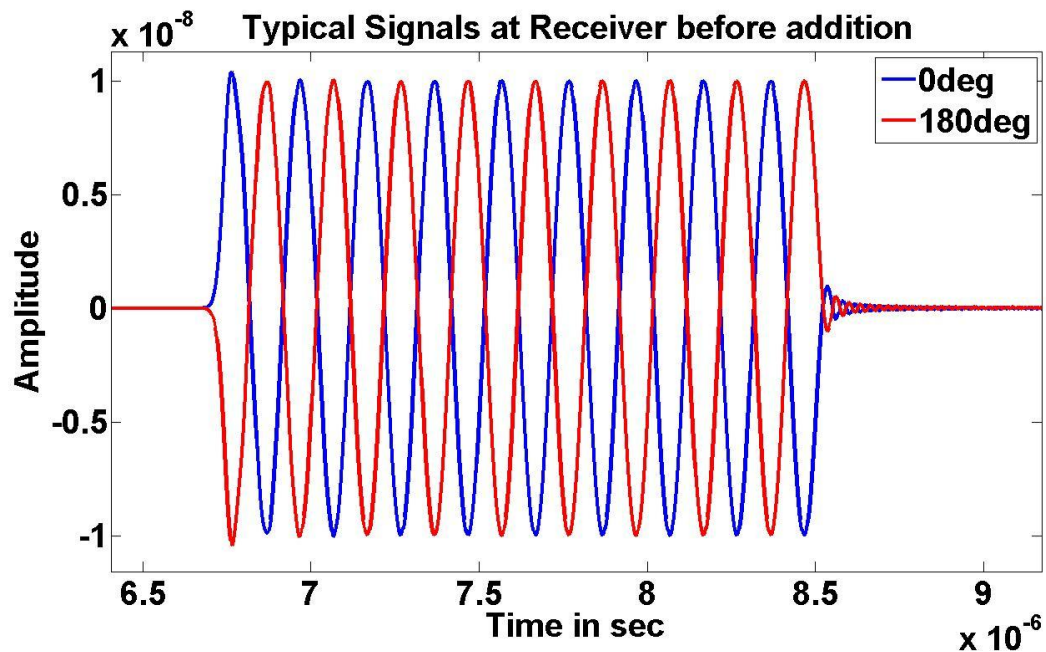
Figure 44 The two pulses at the receiver where the blue is in-phase and red is out-of-phase
