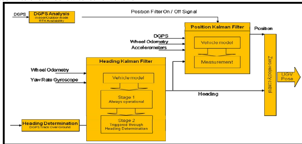
Figure 14: Flow chart for the state-sensing module
