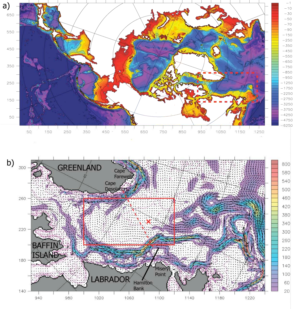
Figure 30. a) domain bathymetry with Labrador Sea bathymetry (m) and red dashed box denoting Labrador Sea region; b) Labrador 26 year 0-122m mean TKE (cm²/s²) (shading) and velocity (vectors). Red box is convective study area, dashed line is AR7W section and x is OWSB.
