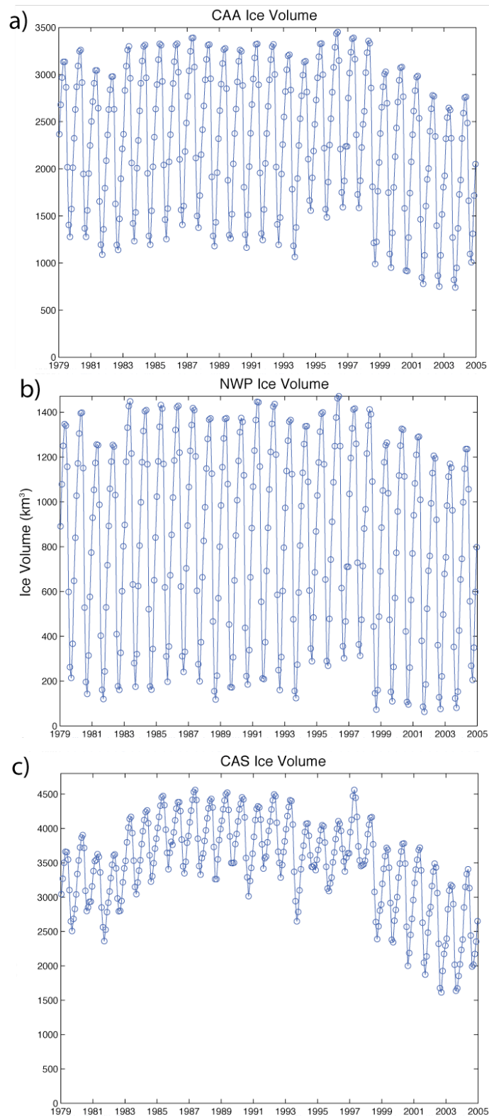
Figure 53. Time series of ice volume ( \text{km}^3 ) a) Canadian Arctic Archipelago (CAA), b) Northwest Passage (NWP) and c) Canadian Arctic Slope (CAS).
