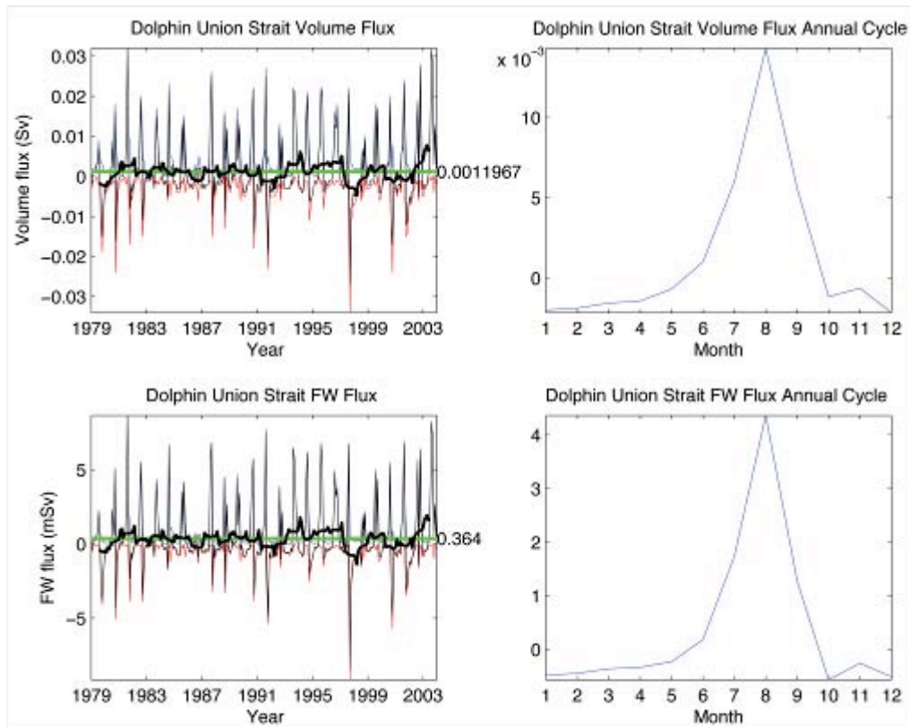
Figure 77. Dolphin Union Strait fluxes. a) volume 26-year time series, b) volume annual cycle, c) freshwater 26-year time series, and d) freshwater annual cycle. For a) and c), blue=flux from west to east, red=flux from east to west, black=net, thick black=13-month running mean of the net. b) and d) are net only.
