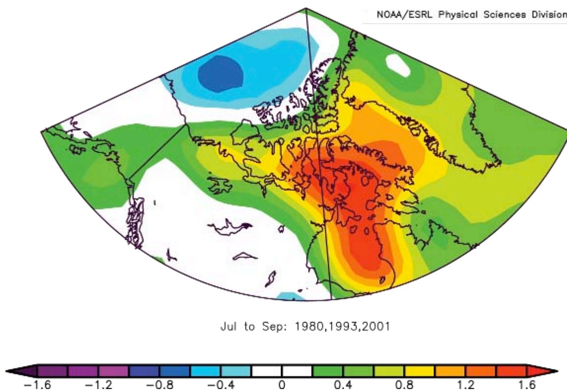
Figure 57. NCEP/NCAR Reanalysis 1000mb air temperature composite anomaly for summers (JAS) during trafficable conditions in the Northwest Passage.
