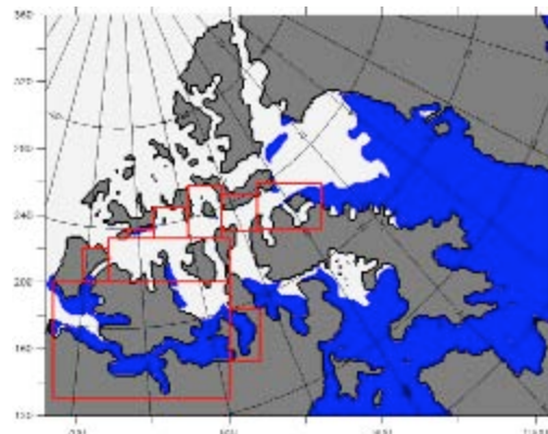
Figure 55. Open water conditions. Blue areas are “open” ( < 1/10 ice concentration) and white are not. This is from August 2001, when both routes through the Northwest Passage were trafficable. However, neither route fit the definition of “open.”
