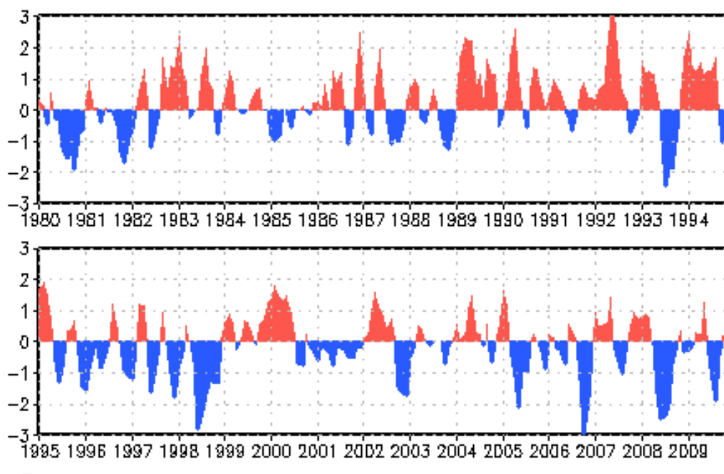
Figure 56. Standardized 3-month running mean NAO Index (From NOAA 2010).
