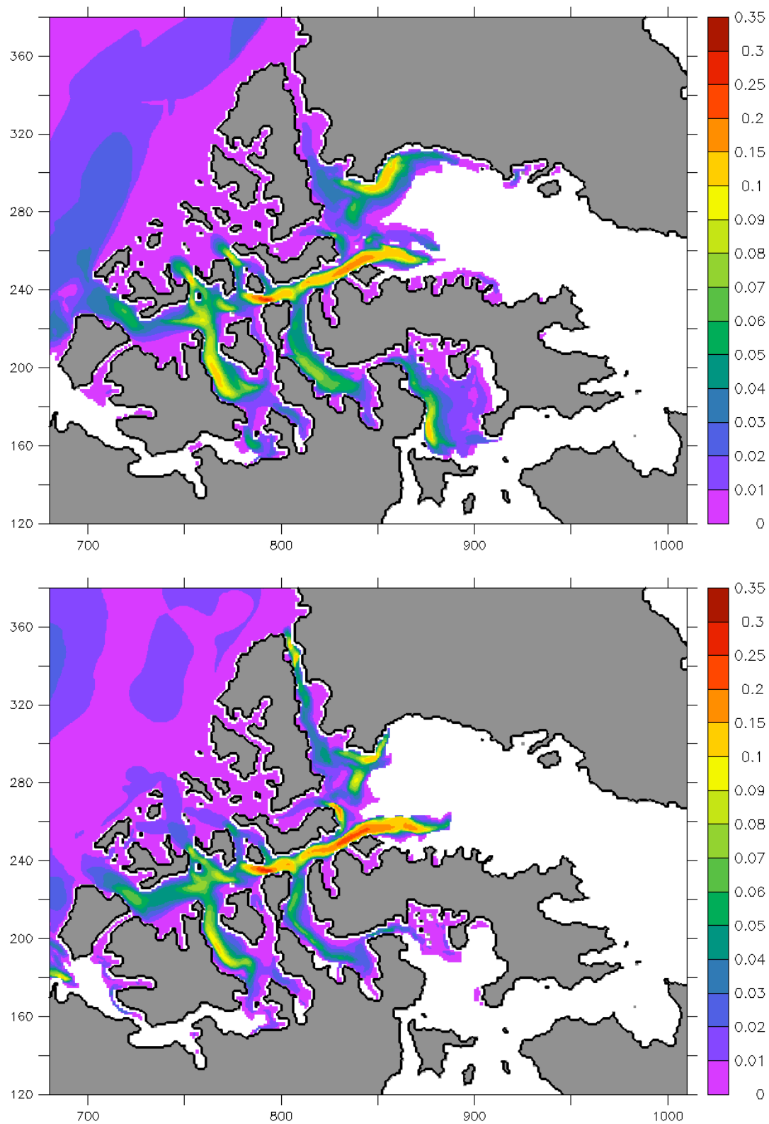
Figure 60. September ice speed (m/s). a) 1979, and b) 2004.
