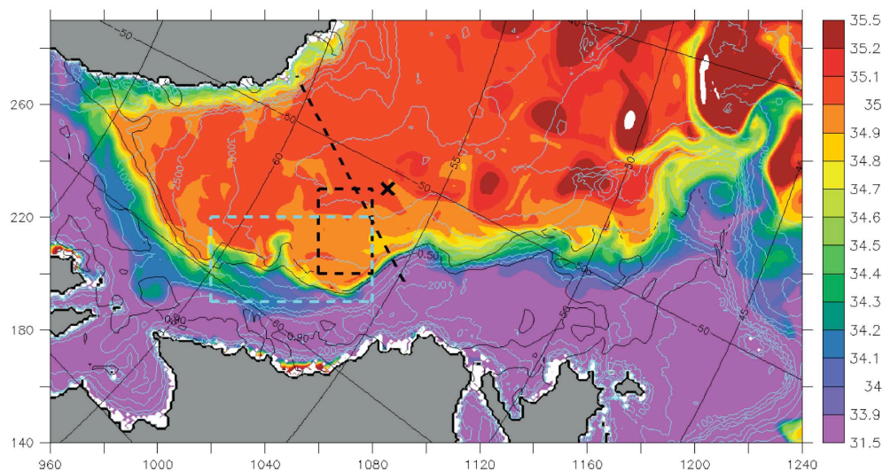
Figure 43. SSS 31 Mar 2002. Light blue dashed box delineates area of focus for this case, dashed black box is the convective area observed by Pickart et al. (2002), dashed black diagonal line is AR7W transect, and black x is OWSB.
