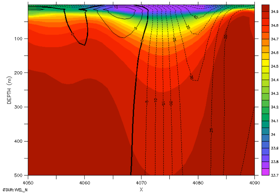
Figure 67. Cross-section of anticyclonic eddy S (shading) and velocity (contours).
