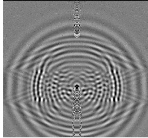
Figure 5.5. Experiment thin(3mm) excitation
