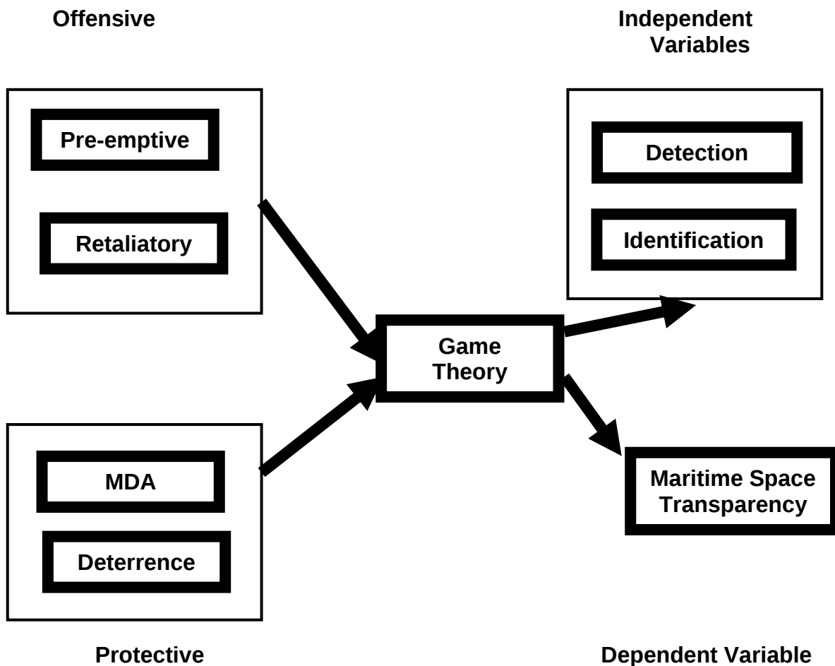
Figure 3. GAME THEORY FLOW CHART
