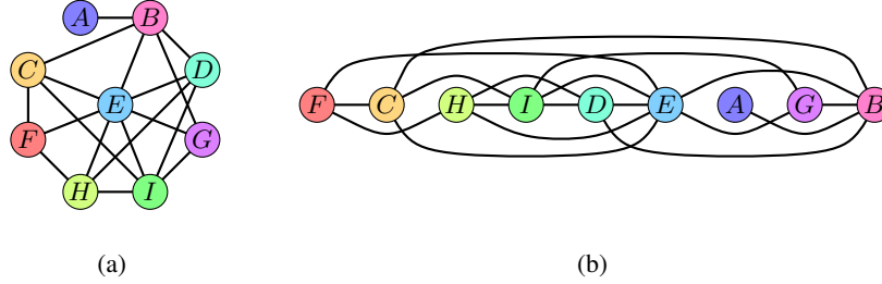
Fig. 1. (a) A graph with degeneracy 3. (b) A vertex ordering showing that the degeneracy is not larger than 3.
