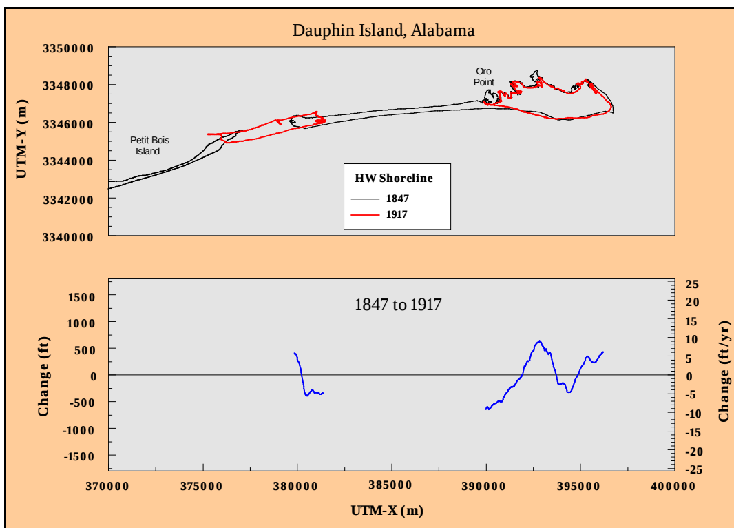
Figure 2-27. Gulf shoreline position change between 1847 and 1917, Dauphin Island, AL.
