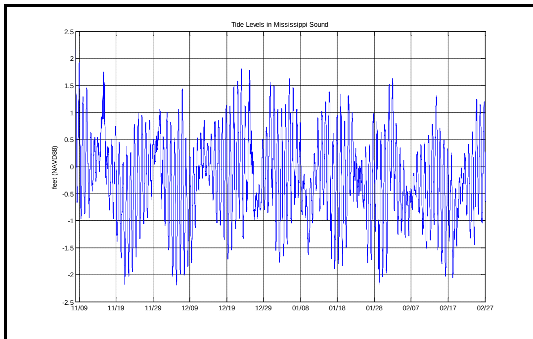
Figure 5-16. Tide data recorded in Mississippi Sound. Elevations are in feet NAVD 88.
