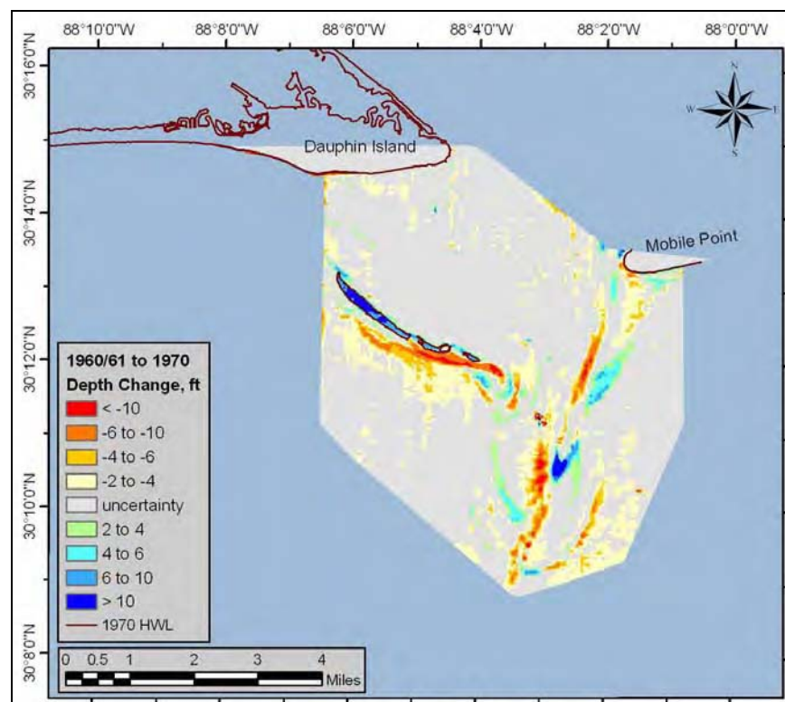
Figure 4-8. Bathymetric changes on the Mobile ebb-tidal delta, 1960/61 to 1970.
