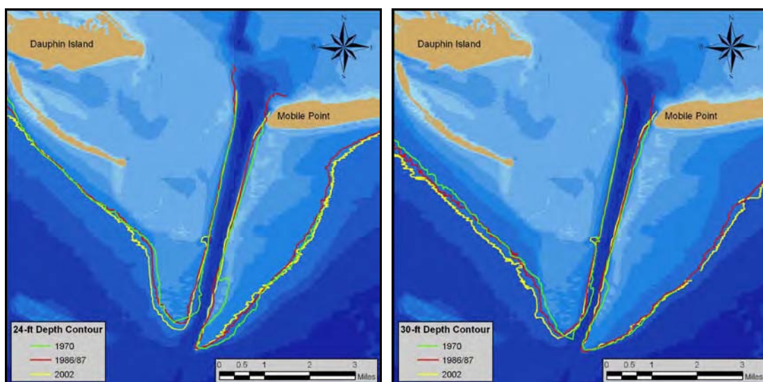
Figure 3-18. Variations in location of the 24- and 30-ft depth contours, 1970, 1986/87, and 2002.
