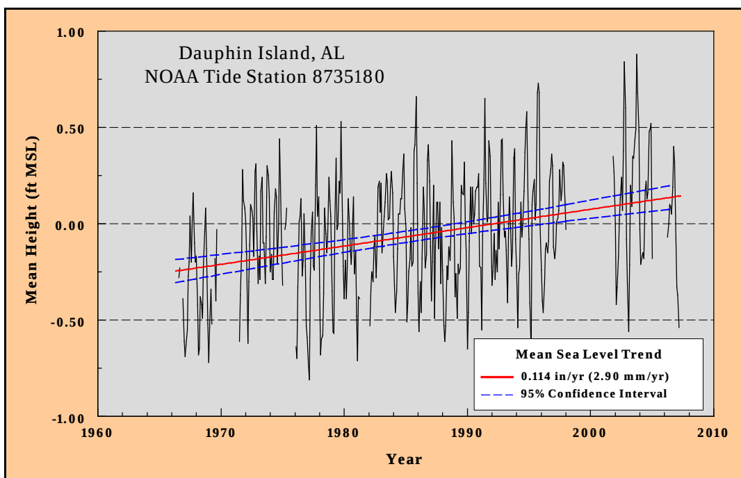
Figure 2-38. Monthly mean water level measurements and sea-level rise trend at Dauphin Island, AL gauge 8735180, 1966 to 2007.
