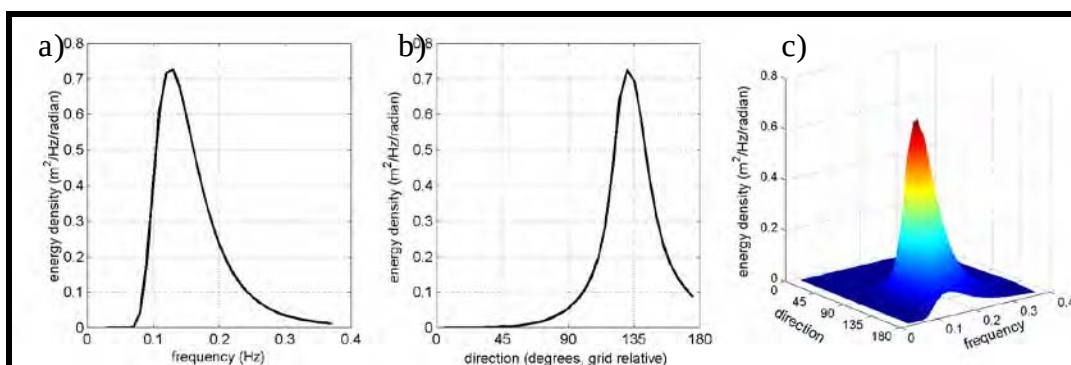
Figure 5-6. STWAVE input spectrum developed using WIS 20-year hindcast data with Goda (1985) method of computing frequency and direction spectrum. Plots show a) frequency distribution of energy at peak direction, b) directional distribution of energy at peak frequency, and c) surface plot of two-dimensional energy spectrum ( H_{m0} = 0.9 m, \theta_{\text{mean}} = 130 deg).
