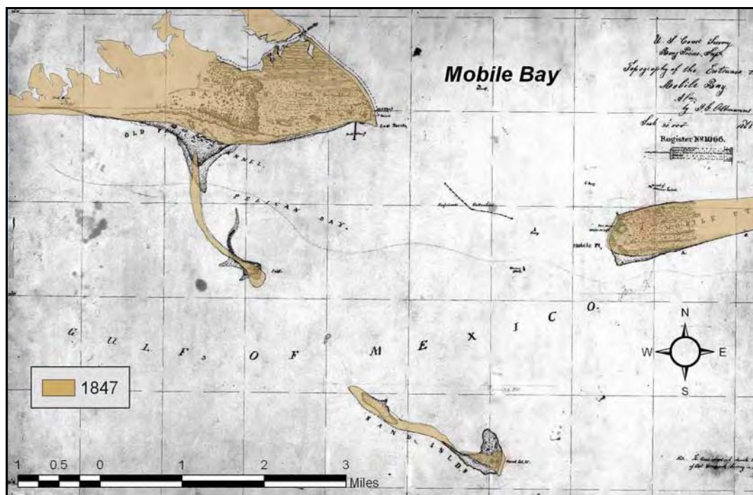
Figure 2-6. 1847 shoreline superimposed on the 1868 registered T-sheet illustrating mass migration of sand from Pelican Island to eastern Dauphin Island.
