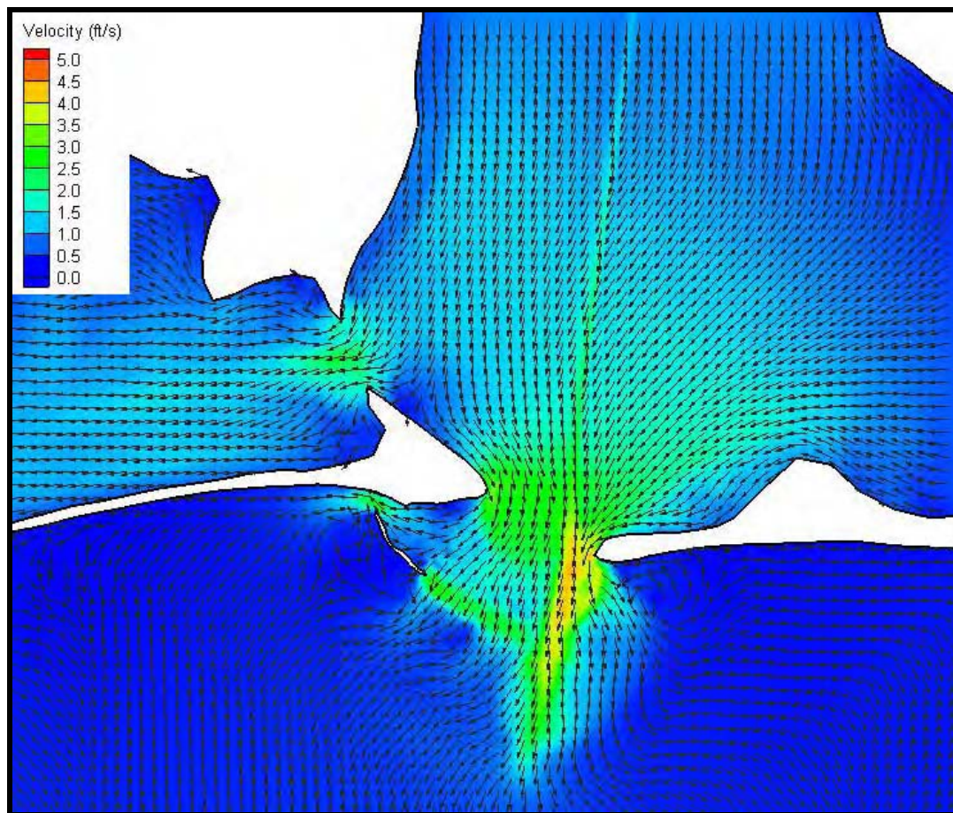
Figure 5-26. Velocity contours and vectors for maximum ebbing tide at Mobile Pass February 26, 2007.
