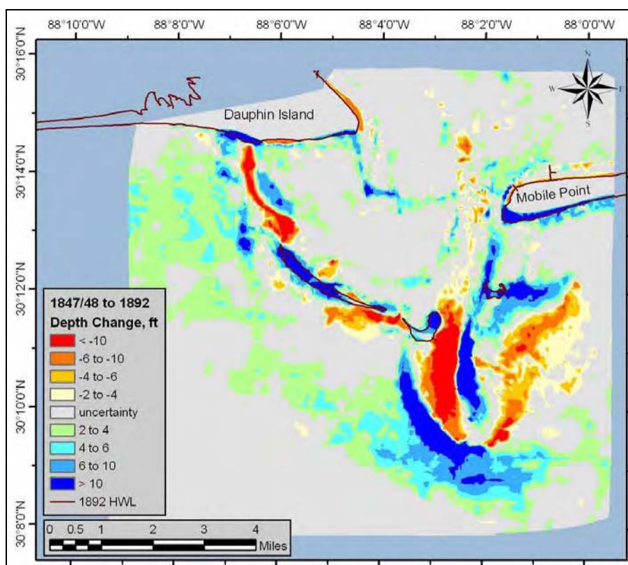
Figure 4-3. Areas of erosion and deposition on the Mobile Pass ebb tidal delta illustrating net movement of the channel and shoals from east to west, 1847/48 to 1892.
