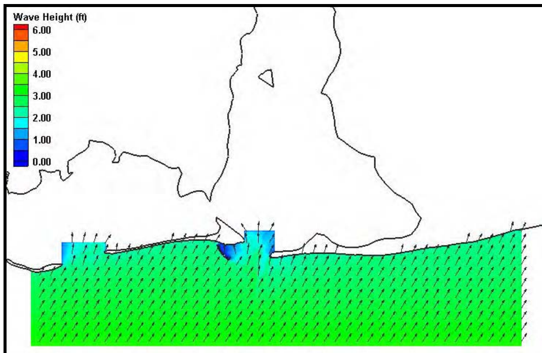
Figure H8. Coarse grid (200m x 200m) wave results for Case 8. Wave heights are shown by color while wave direction is indicated by the arrow direction.
