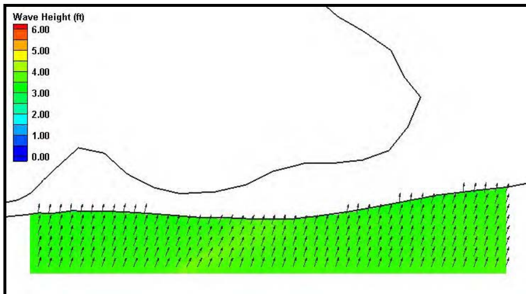
Figure H37. Fine grid (25m x 25m) wave results for Case 7, Morgan Peninsula. Wave heights are shown by color while wave direction is indicated by the arrow direction.
