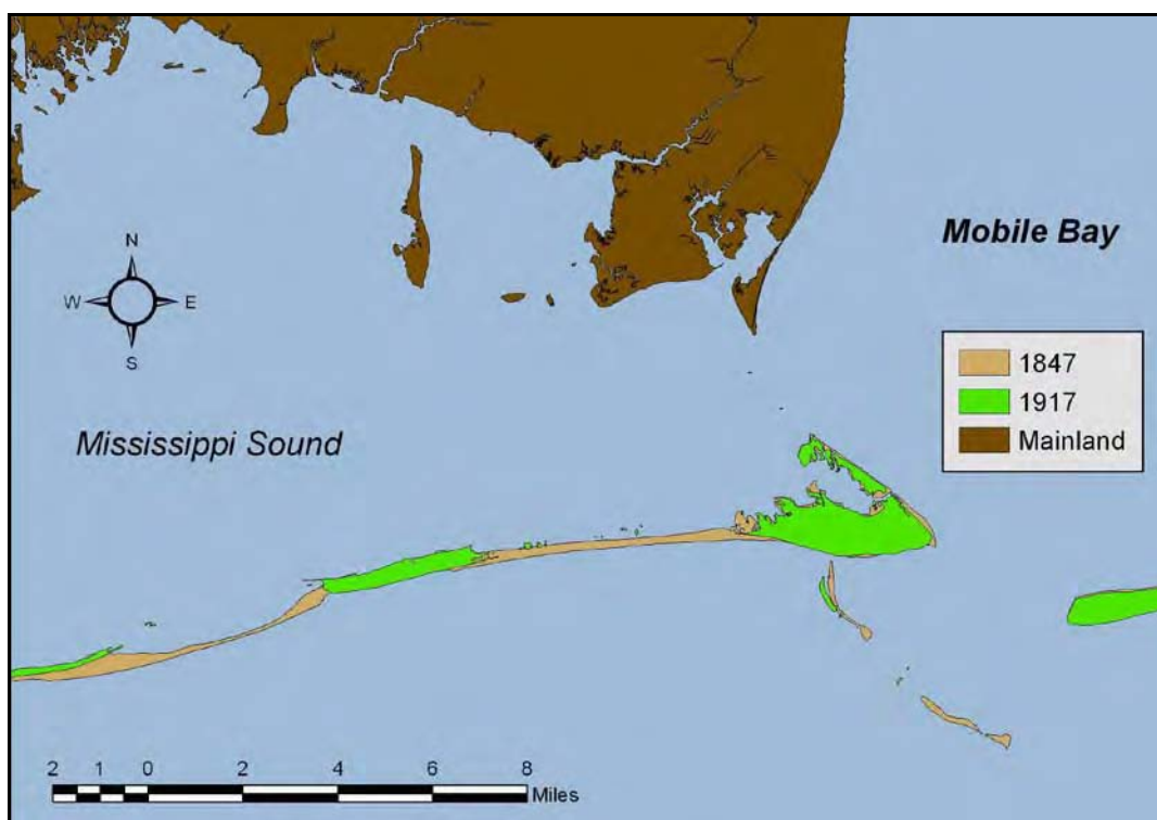
Figure 2-5. 1917 shoreline superimposed on the 1847 shoreline illustrating westward growth of Dauphin Island, forcing Petit Bois Pass and Island to the west. The large breach between east and west Dauphin Island in 1917 is the result of the July 1916 hurricane.
