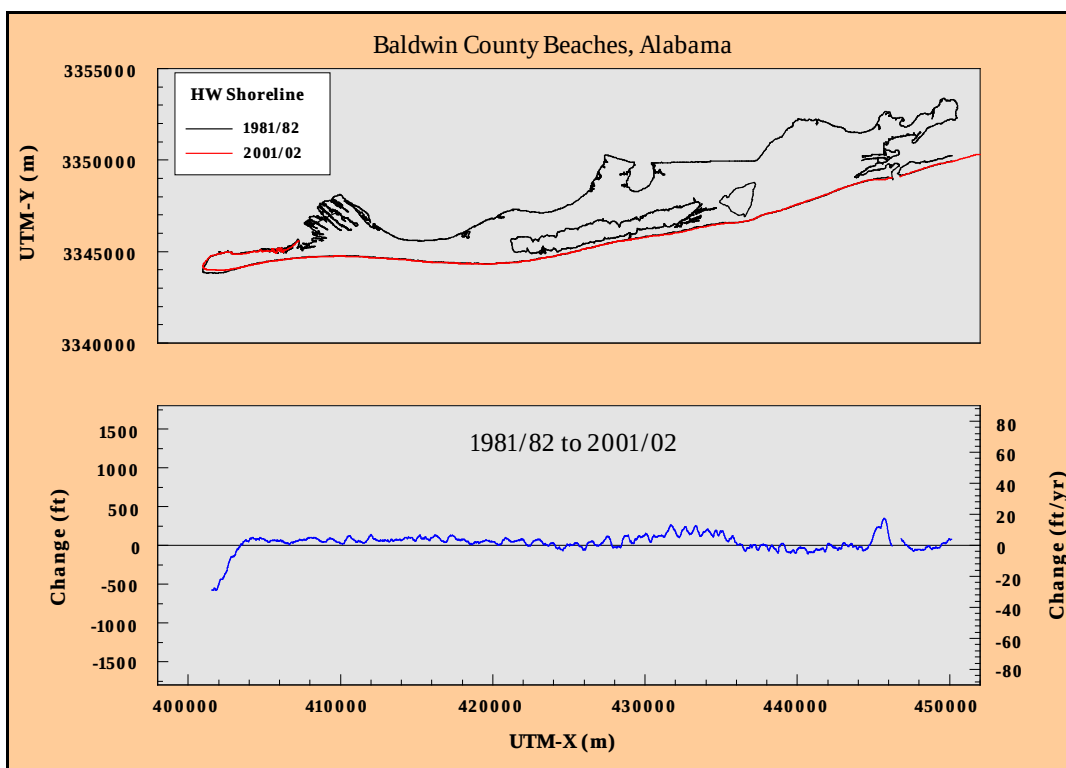
Figure D8. Historical shoreline position change, Perdido Pass to Mobile Point, Alabama: 1981/82 to 2001/02.
