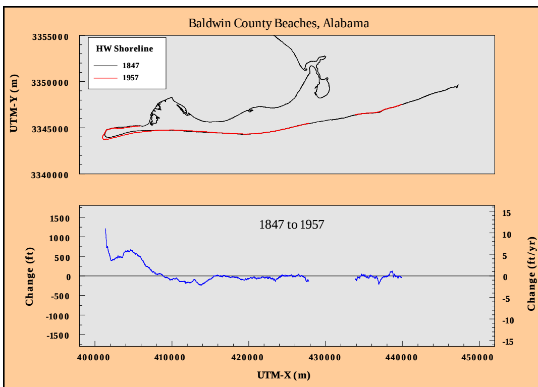
Figure D5. Historical shoreline position change, Perdido Pass to Mobile Point, Alabama: 1847 to 1957.
