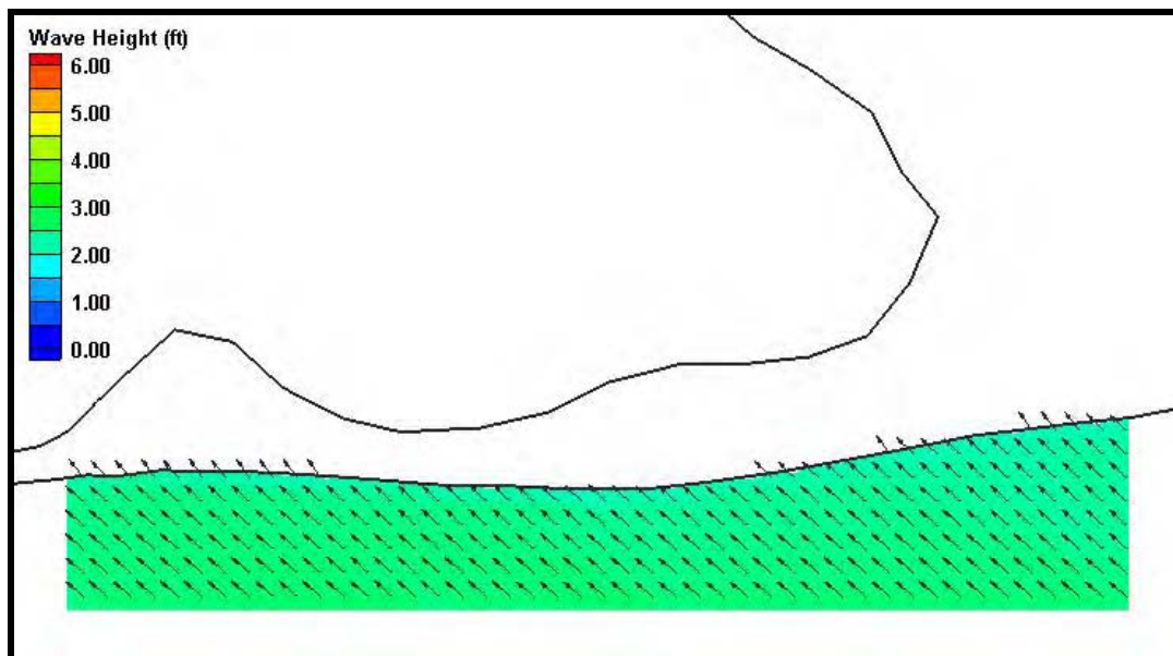
Figure H31. Fine grid (25m x 25m) wave results for Case 1, Morgan Peninsula. Wave heights are shown by color while wave direction is indicated by the arrow direction.
