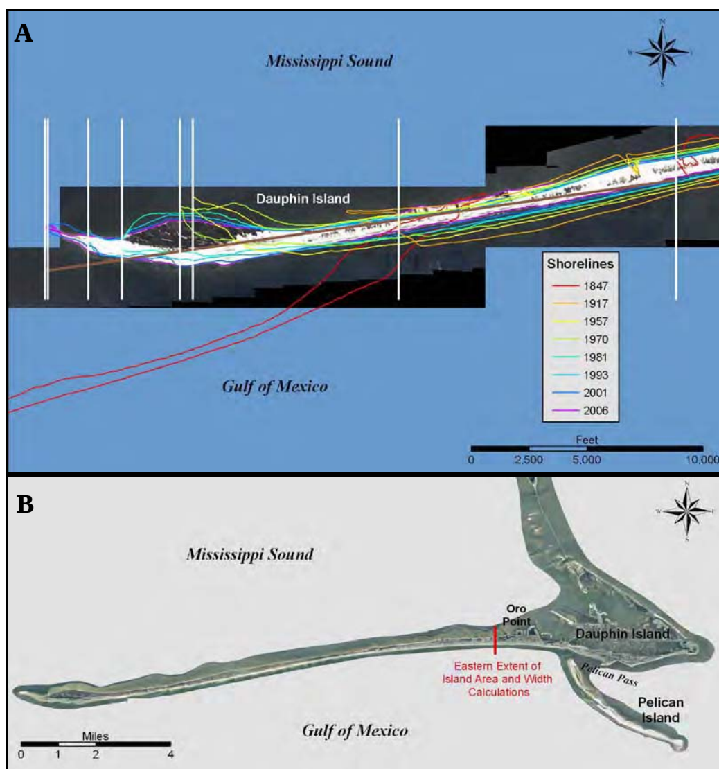
Figure 2-16. Measurement boundaries for quantifying island dimension changes relative to 2006 (A) and 2002 (B) orthophotography: A) lateral island growth calculations, and B) island width and area calculations.
