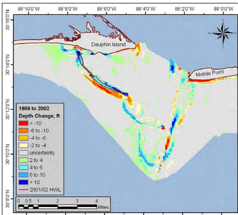
Figure 4-10. Bathymetric changes on the Mobile ebb-tidal delta, 1986 to 2002.
