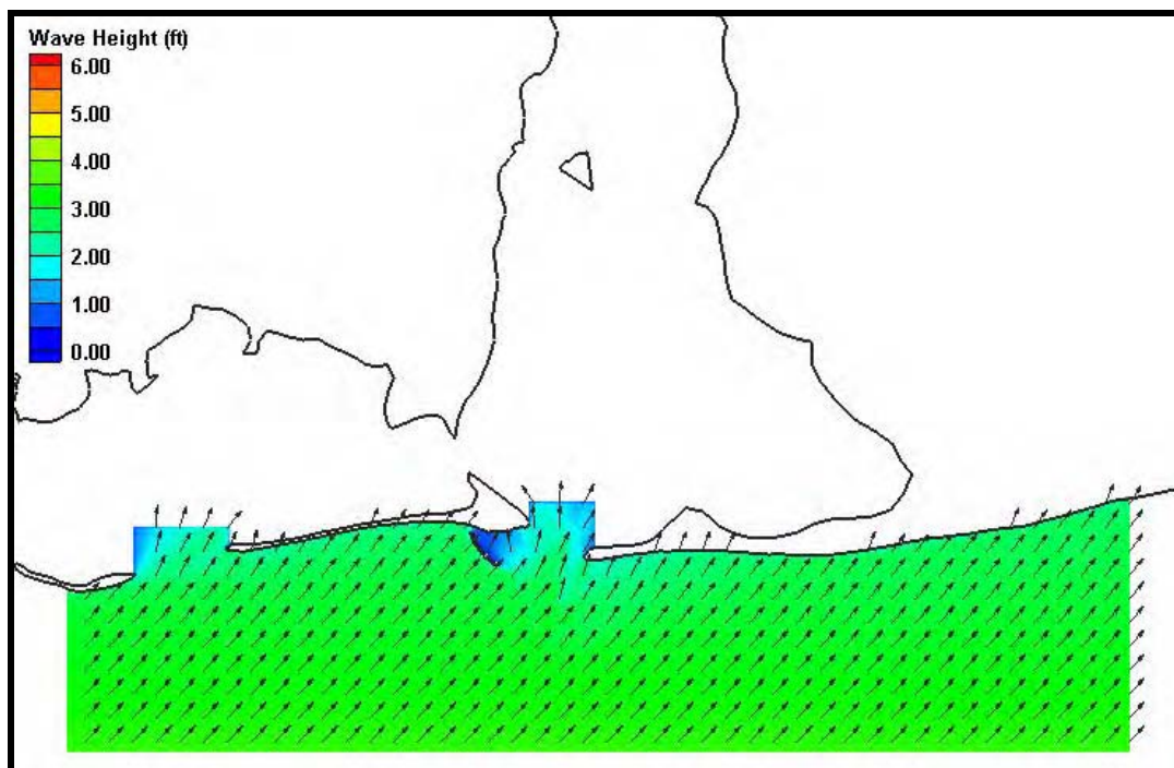
Figure H9. Coarse grid (200m x 200m) wave results for Case 9. Wave heights are shown by color while wave direction is indicated by the arrow direction.
