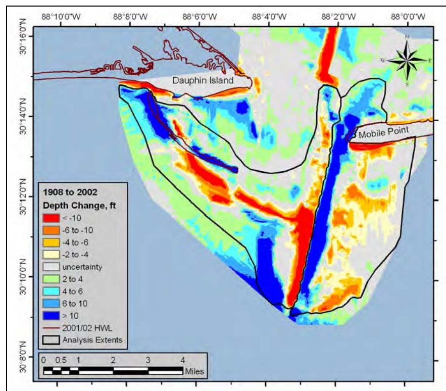
Figure G10. Analysis extent for calculating sand volume change – 1908 to 2002.
