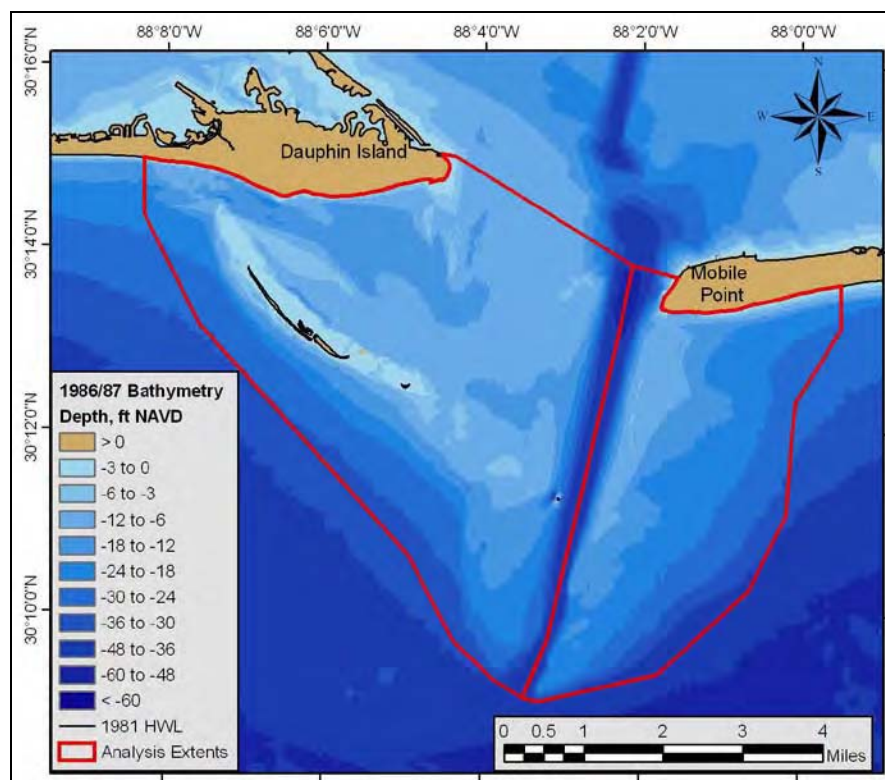
Figure F6. Analysis extent for calculating sand volume above 30-ft depth contour – 1986/87.
