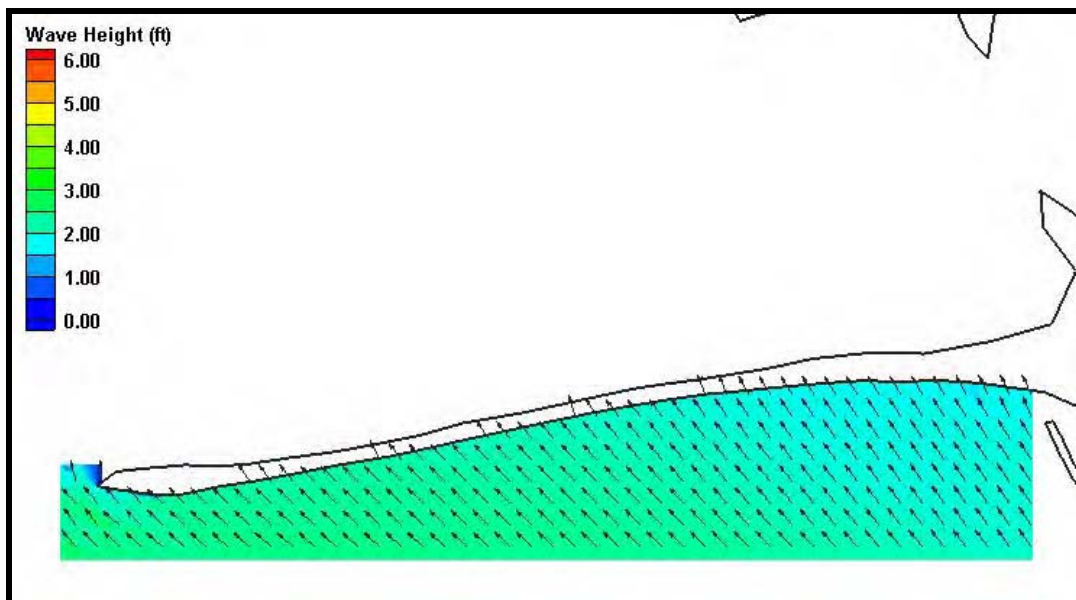
Figure H11. Fine grid (25m x 25m) wave results for Case 1, Dauphin Island. Wave heights are shown by color while wave direction is indicated by the arrow direction.
