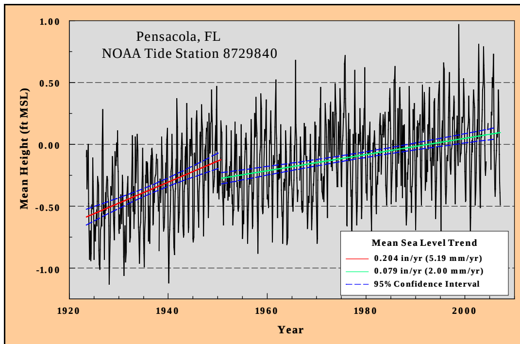
Figure 2-39. Monthly mean water level measurements and sea-level rise trends at Pensacola, FL gauge 8729840, 1923 to 1950 and 1951 to 2007.
