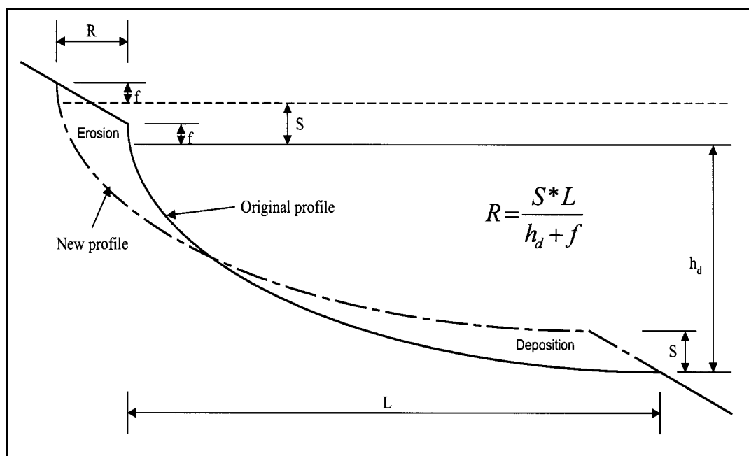
Figure 2-35. Translation of a beach profile under rising sea level in a two-dimensional closed material balance system (after Bruun, 1962).
