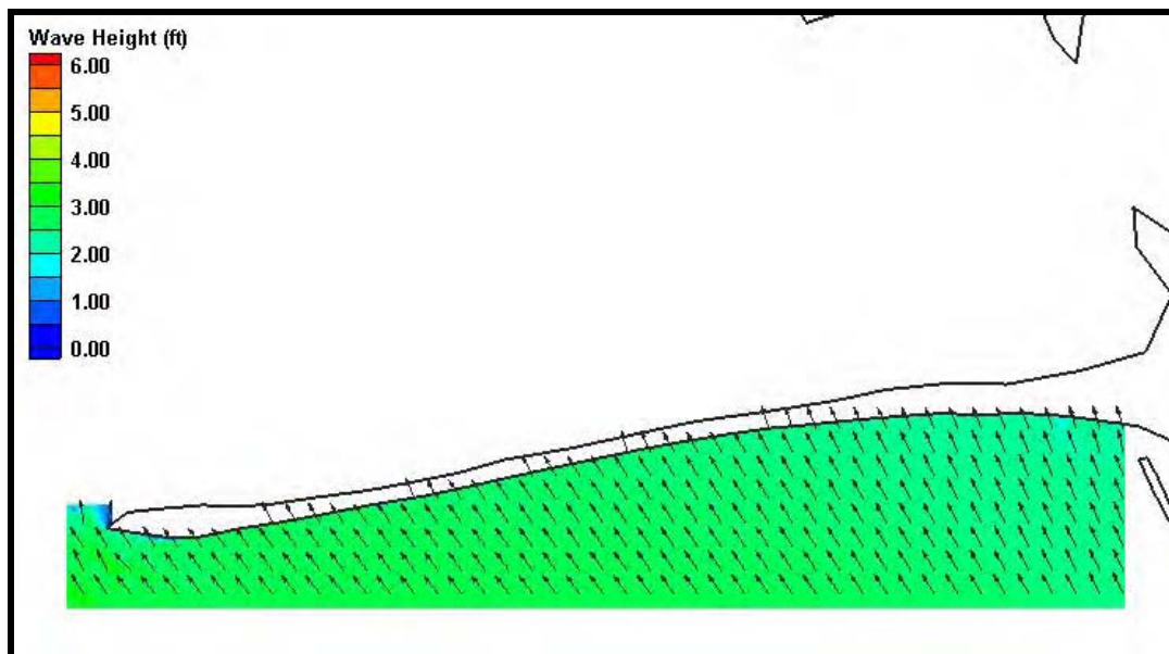
Figure H12. Fine grid (25m x 25m) wave results for Case 2, Dauphin Island. Wave heights are shown by color while wave direction is indicated by the arrow direction.
