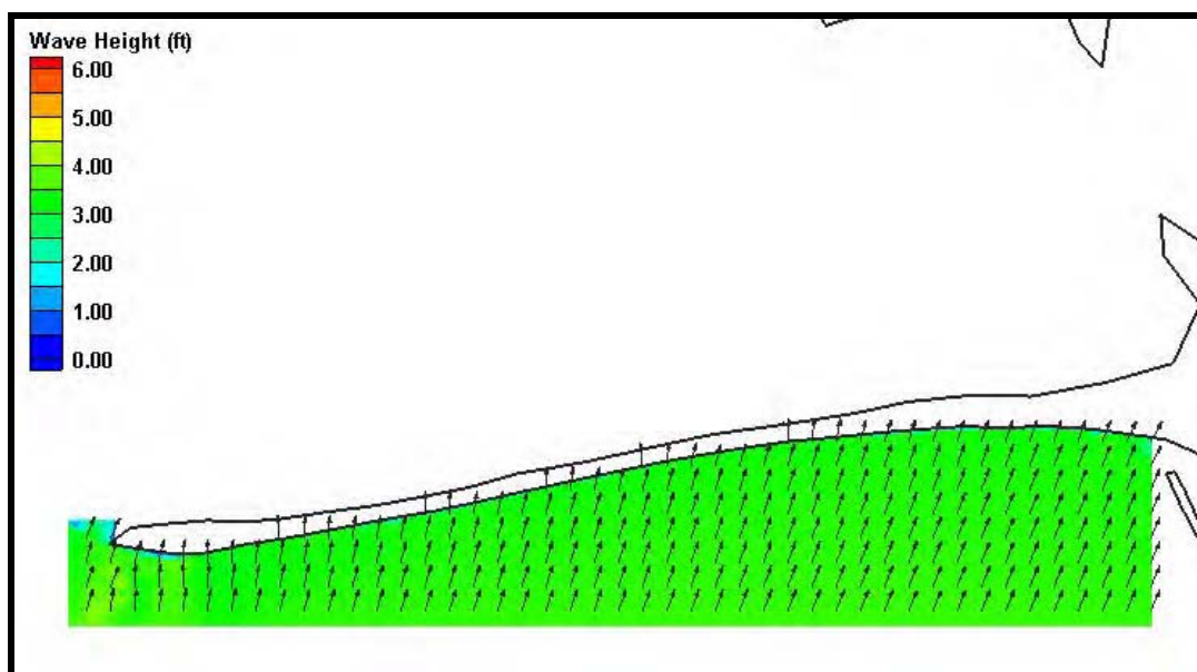
Figure H17. Fine grid (25m x 25m) wave results for Case 7, Dauphin Island. Wave heights are shown by color while wave direction is indicated by the arrow direction.
