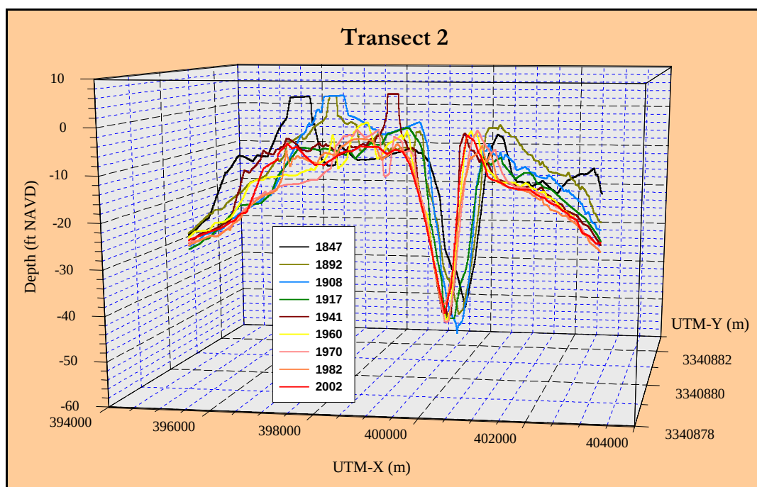
Figure 3-21. Elevation changes along Transect 2, 1847 to 2002.
