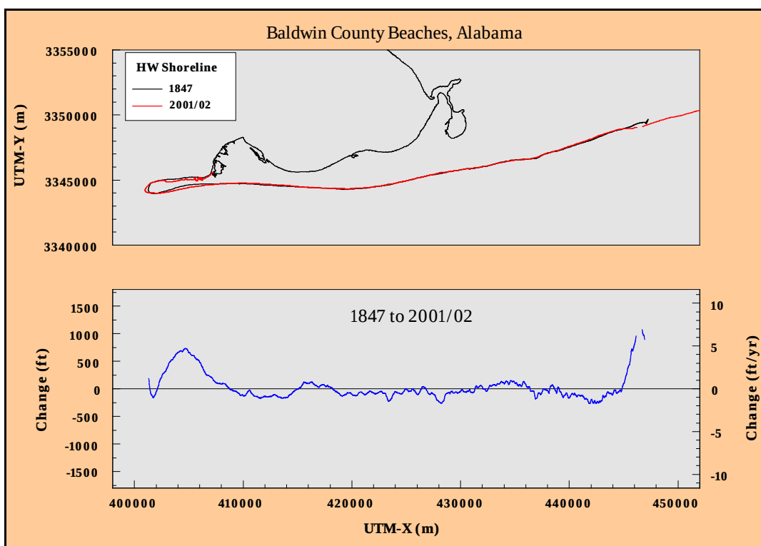
Figure D9. Historical shoreline position change, Perdido Pass to Mobile Point, Alabama: 1847 to 2001/02.
