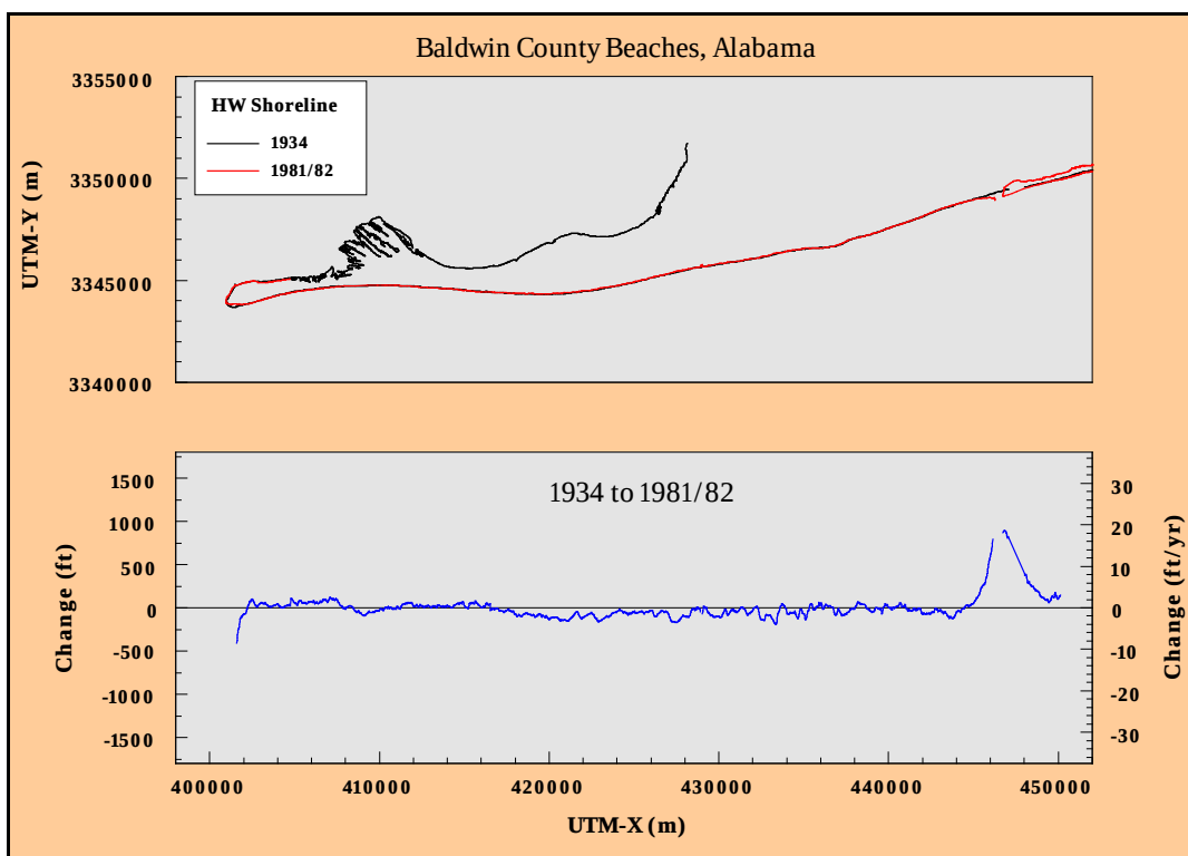
Figure D6. Historical shoreline position change, Perdido Pass to Mobile Point, Alabama: 1934 to 1981/82.
