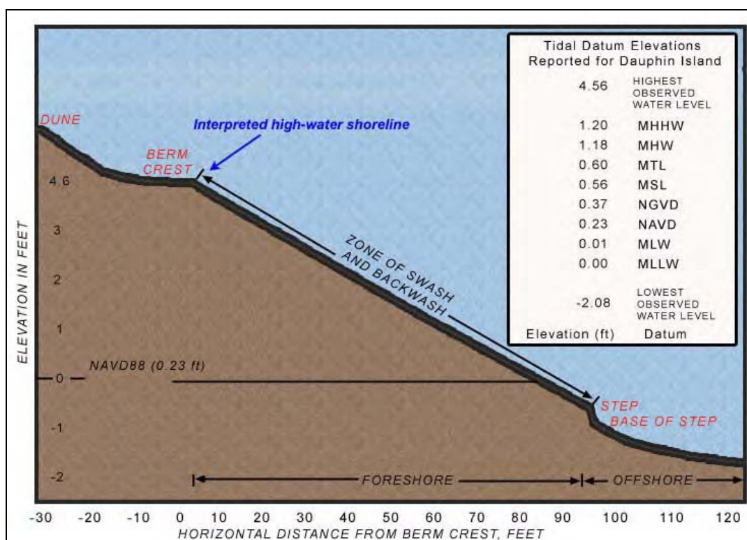
Figure 2-4. High-water shoreline position classification referenced to the beach berm crest.
