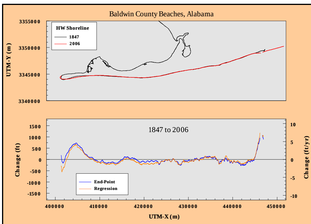
Figure 2-34. Net shoreline change between 1847 and 2006 for beaches between Perdido Pass and Mobile Point, Alabama.
