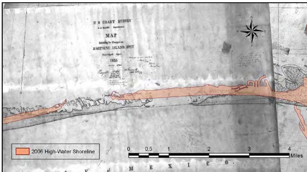
Figure 2-25. 2006 shoreline overlying the breached area in 1853, illustrating the same general location for storm breach vulnerability in 2006 as in 1853.
