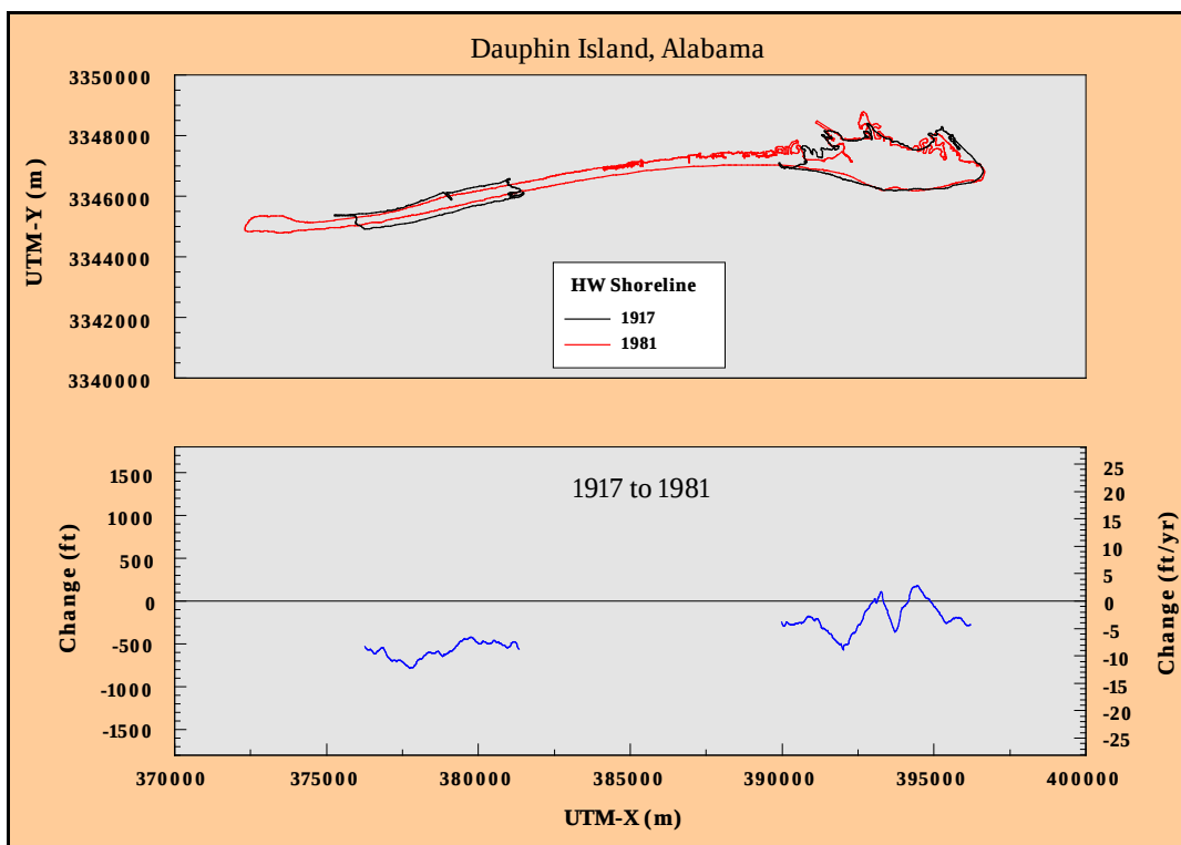
Figure C11. Historical shoreline position change, Dauphin Island, Alabama: 1917 to 1981.
