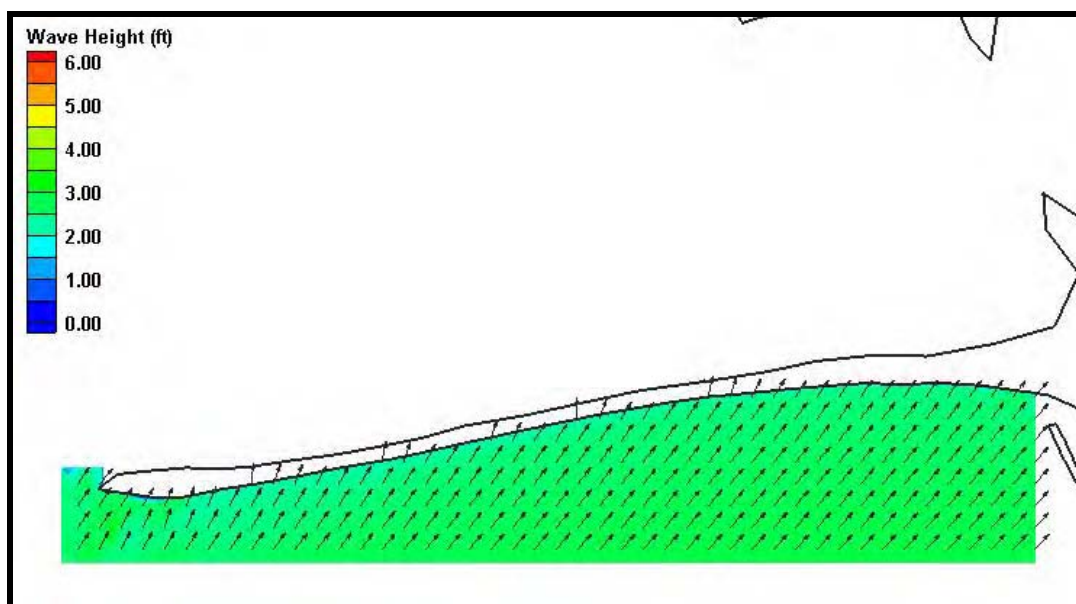
Figure H19. Fine grid (25m x 25m) wave results for Case 9, Dauphin Island. Wave heights are shown by color while wave direction is indicated by the arrow direction.
