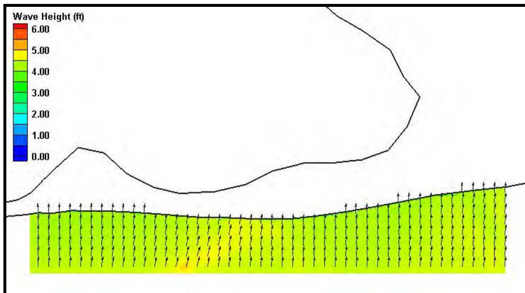
Figure H36. Fine grid (25m x 25m) wave results for Case 6, Morgan Peninsula. Wave heights are shown by color while wave direction is indicated by the arrow direction.
