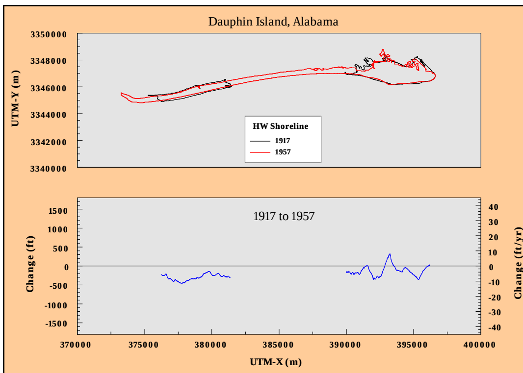
Figure C5. Historical shoreline position change, Dauphin Island, Alabama: 1917 to 1957.
