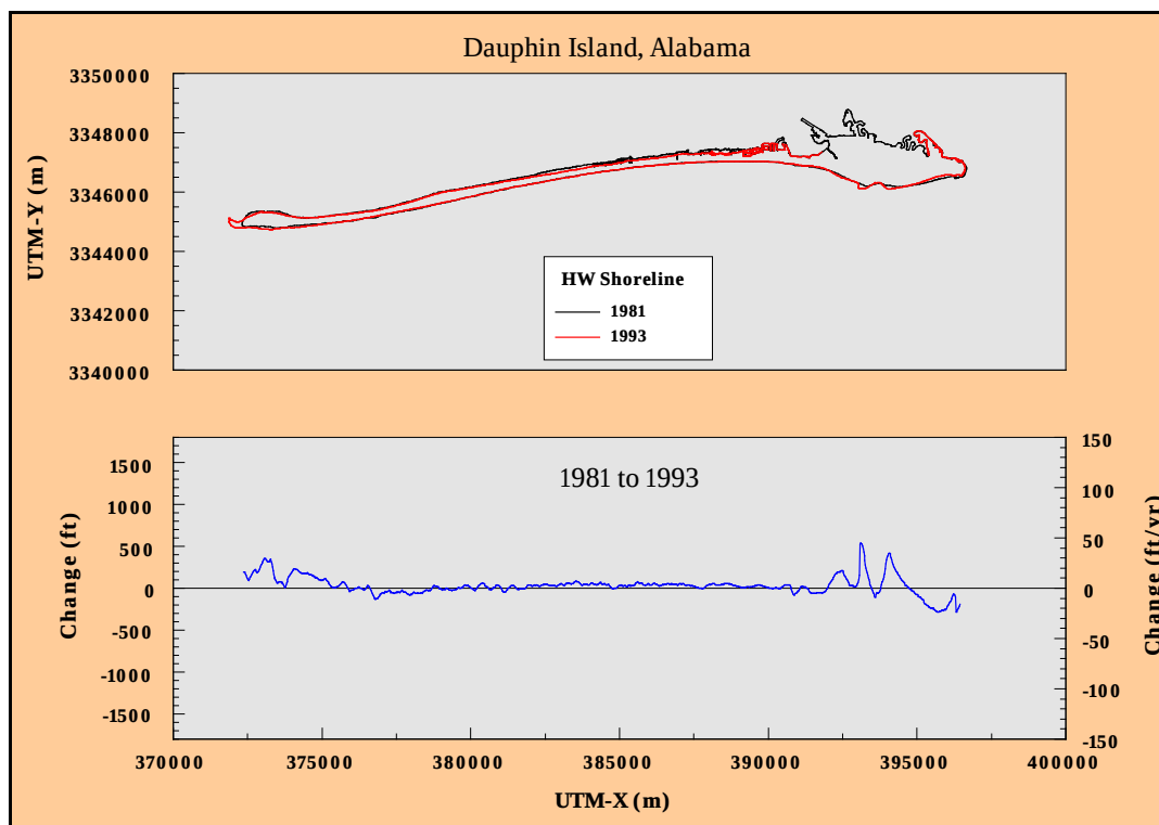
Figure C13. Historical shoreline position change, Dauphin Island, Alabama: 1981 to 1993.
