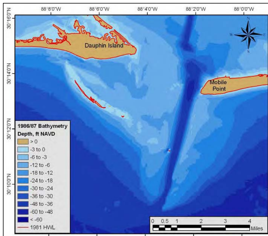
Figure 3-13. Bathymetric surface for Mobile Pass ebb-tidal delta and adjacent shores, 1986/87.
