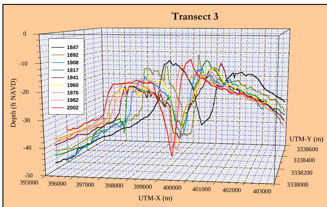
Figure 3-22. Elevation changes along Transect 3, 1847 to 2002.
