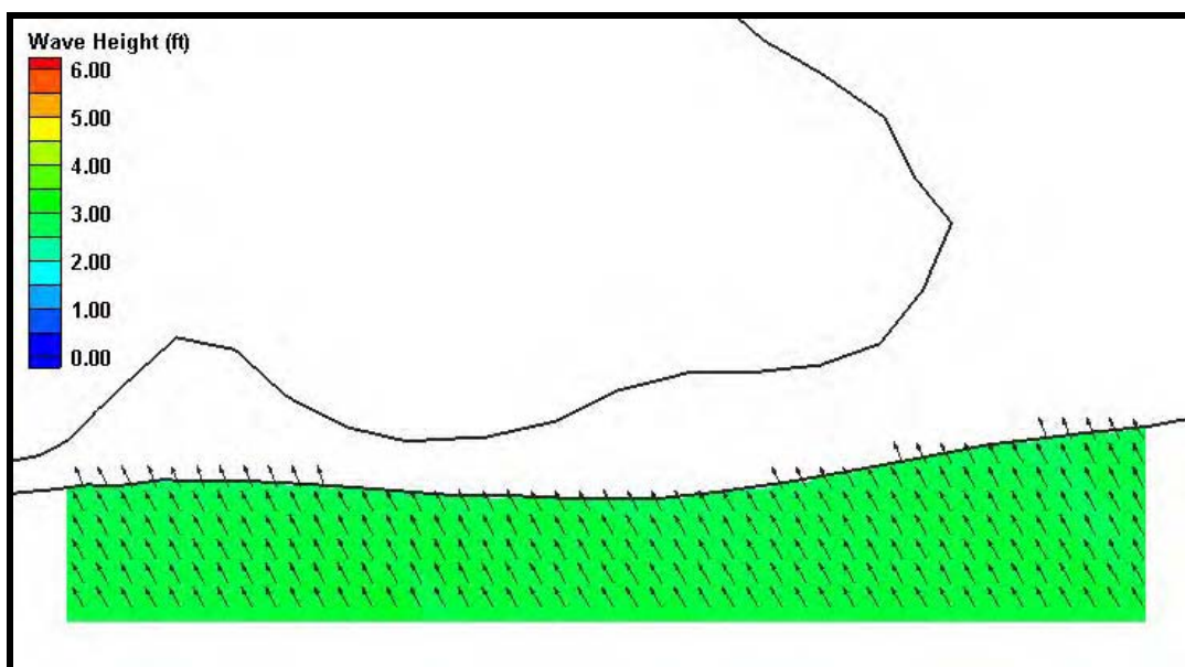
Figure H33. Fine grid (25m x 25m) wave results for Case 3, Morgan Peninsula. Wave heights are shown by color while wave direction is indicated by the arrow direction.
