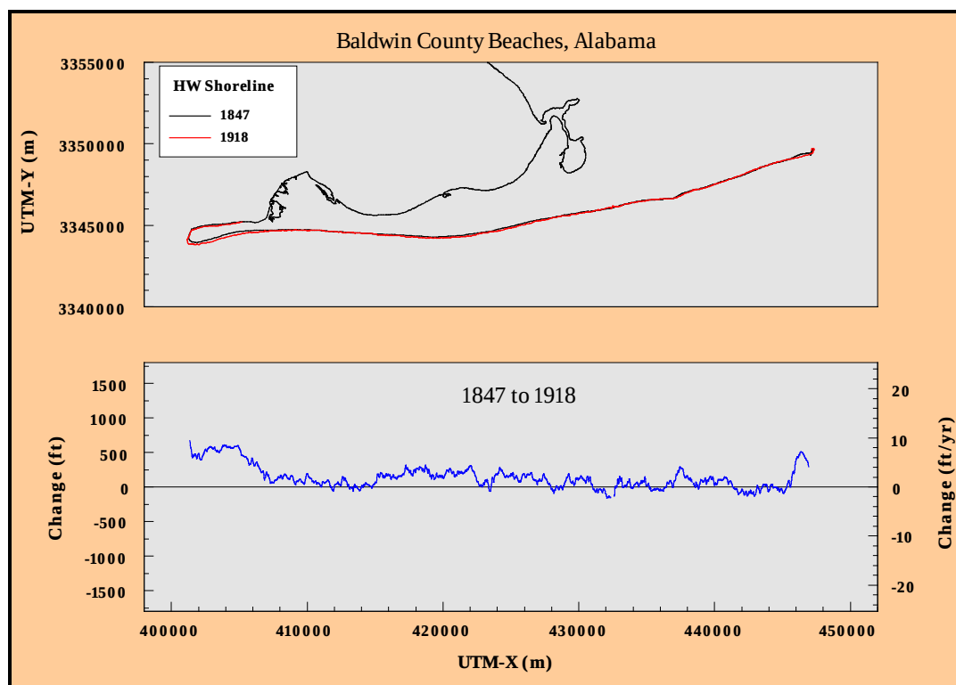
Figure D1. Historical shoreline position change, Perdido Pass to Mobile Point, Alabama: 1847 to 1918.
