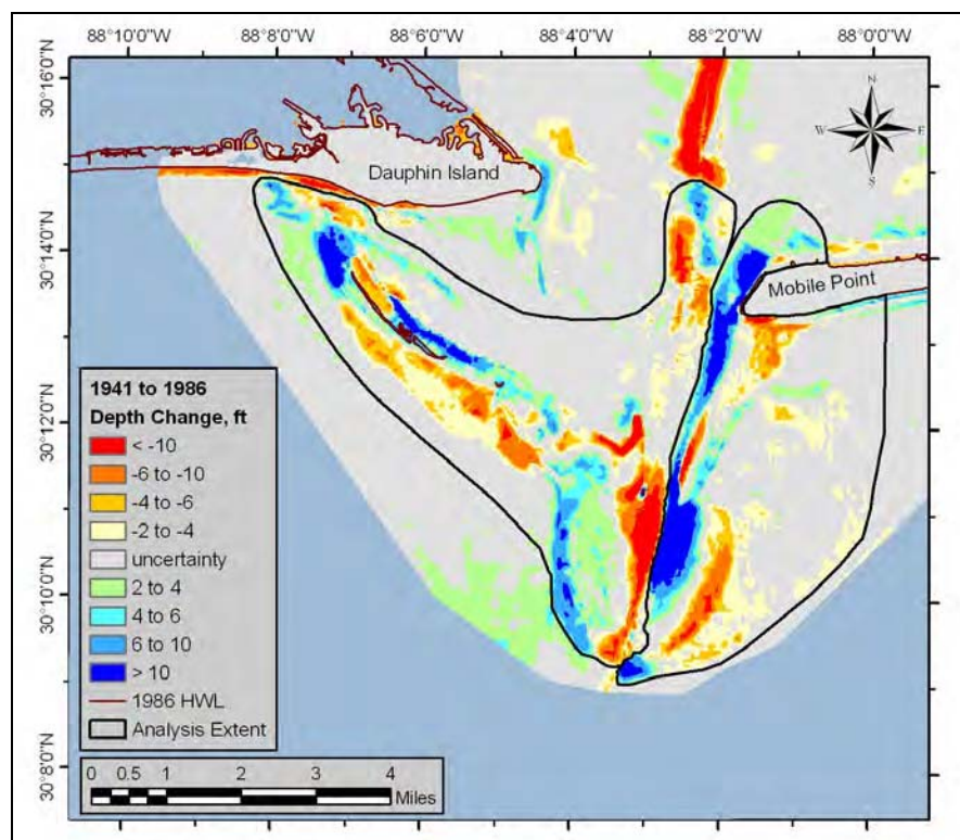
Figure G6. Analysis extent for calculating sand volume change – 1941 to 1986.
