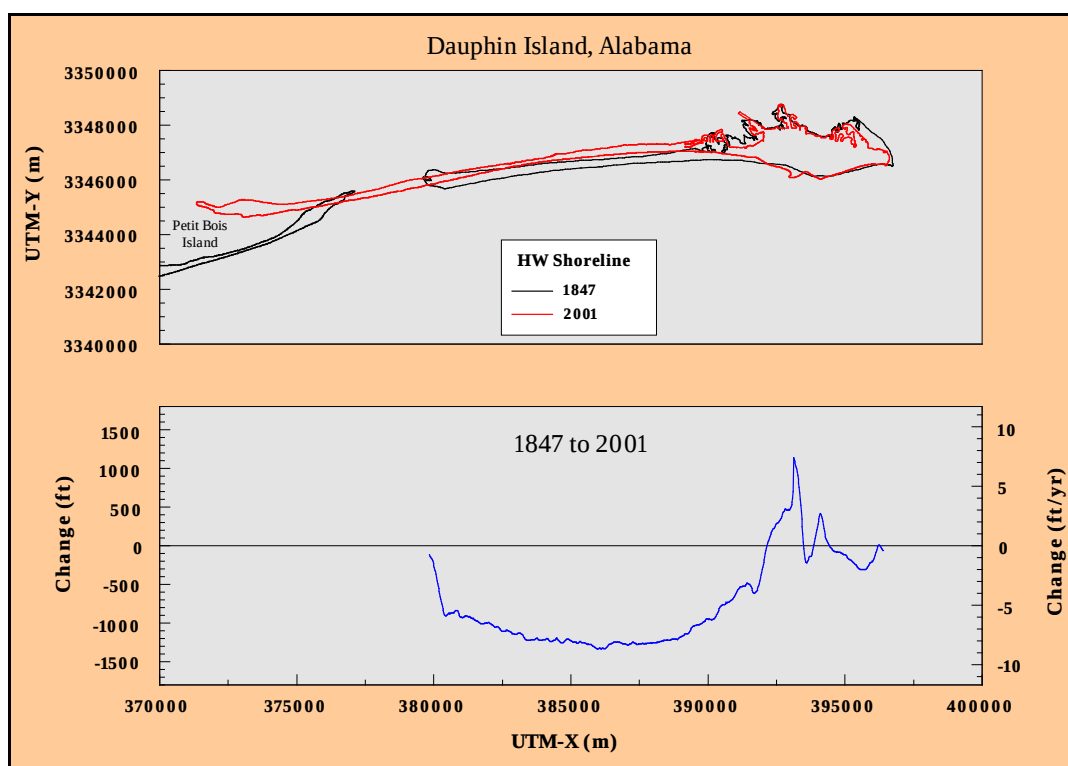
Figure C18. Historical shoreline position change, Dauphin Island, Alabama: 1847 to 2001.
