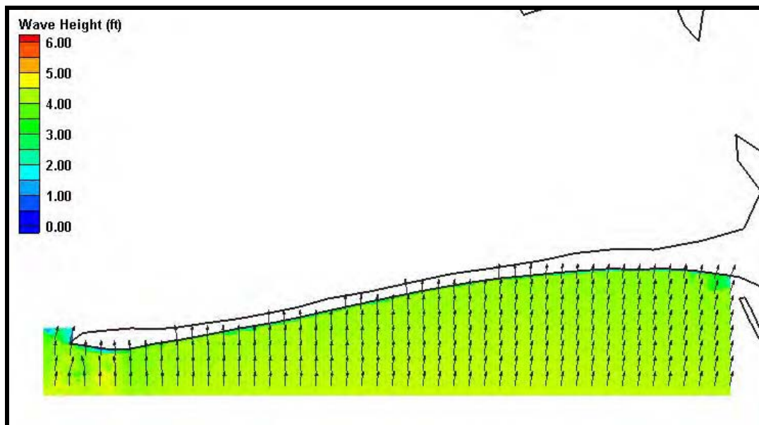
Figure H16. Fine grid (25m x 25m) wave results for Case 6, Dauphin Island. Wave heights are shown by color while wave direction is indicated by the arrow direction.
