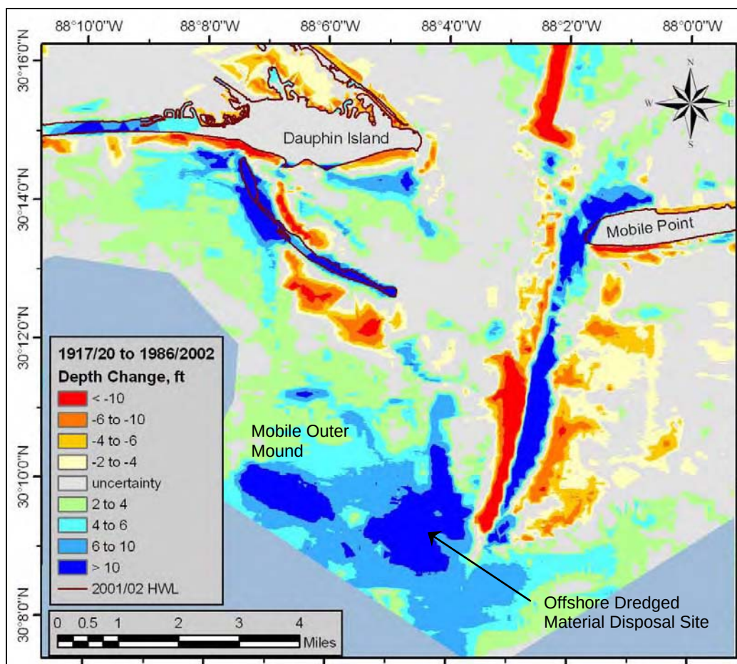
Figure 6-1. Location of offshore dredged material disposal site and the Mobile Outer Mound relative to deposition on the ebb-tidal delta.
