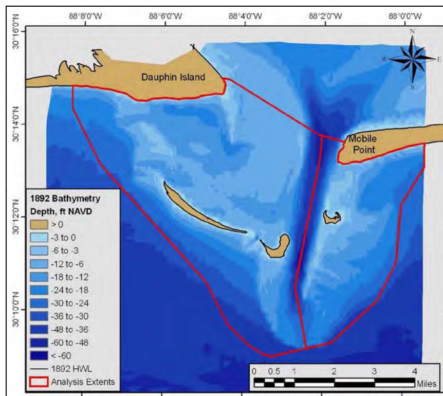
Figure F2. Analysis extent for calculating sand volume above 30-ft depth contour – 1892.
