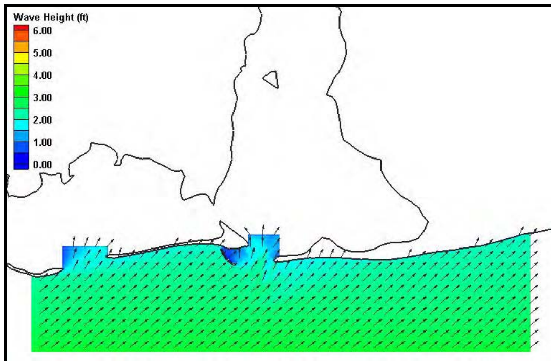
Figure H10. Coarse grid (200m x 200m) wave results for Case 10. Wave heights are shown by color while wave direction is indicated by the arrow direction.
