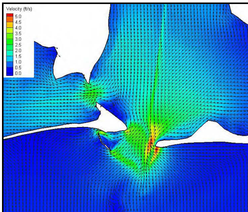
Figure 5-25. Velocity contours and vectors for maximum flooding tide at Mobile Pass February 26, 2007.
