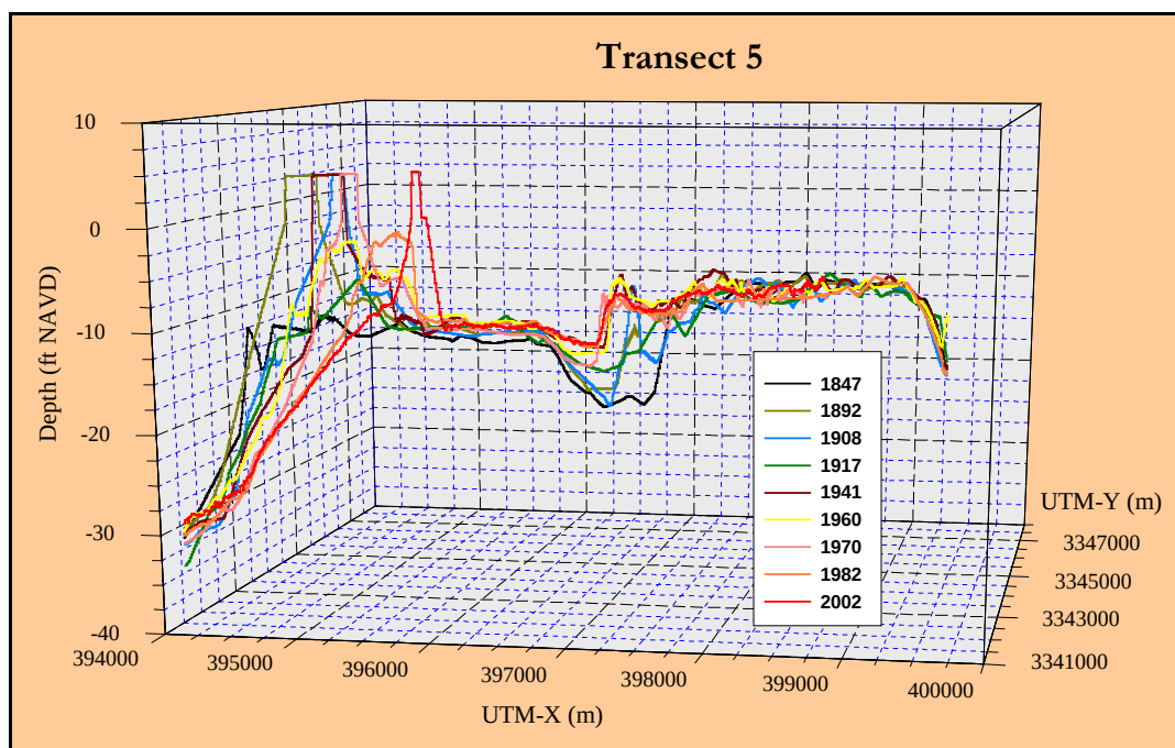
Figure 3-24. Elevation changes along Transect 5, 1847 to 2002.
