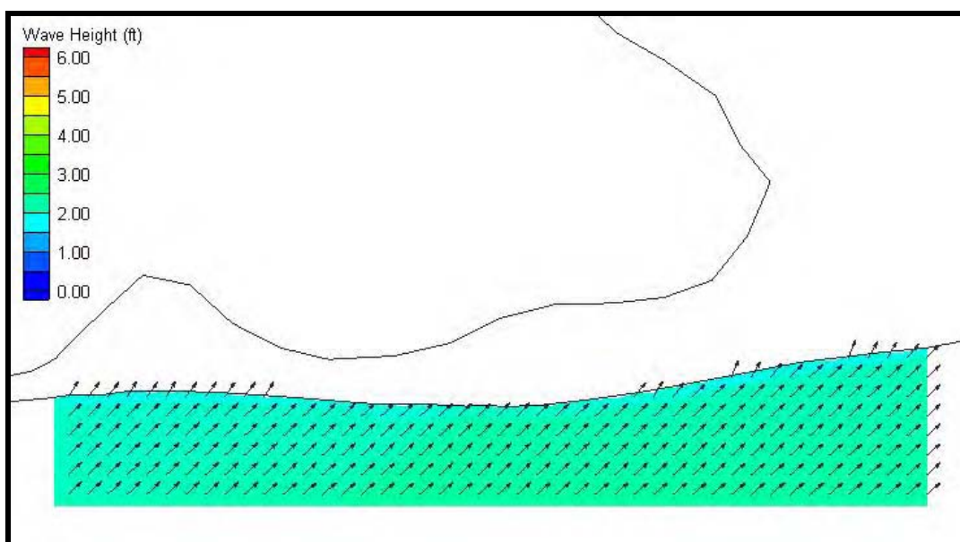
Figure 5-14. Fine grid (25 m x 25 m) wave results for Case 10, Morgan Peninsula. Wave heights are shown by color while wave direction is indicated by the arrow direction.
