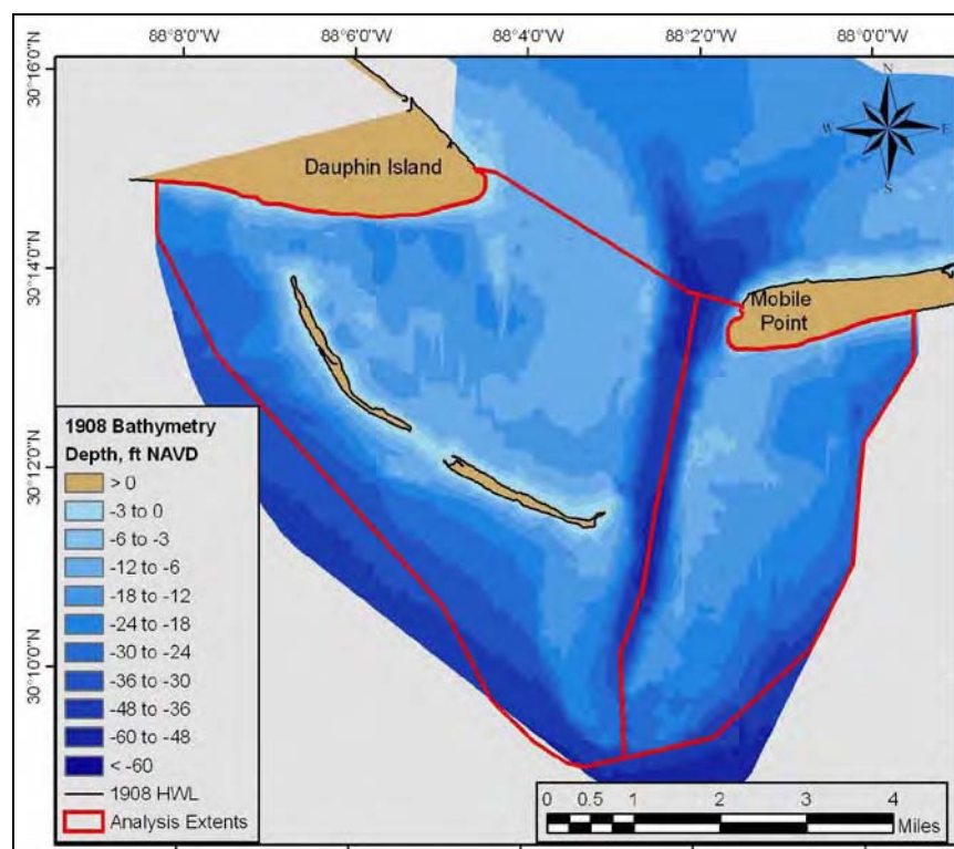
Figure F3. Analysis extent for calculating sand volume above 30-ft depth contour – 1908.
