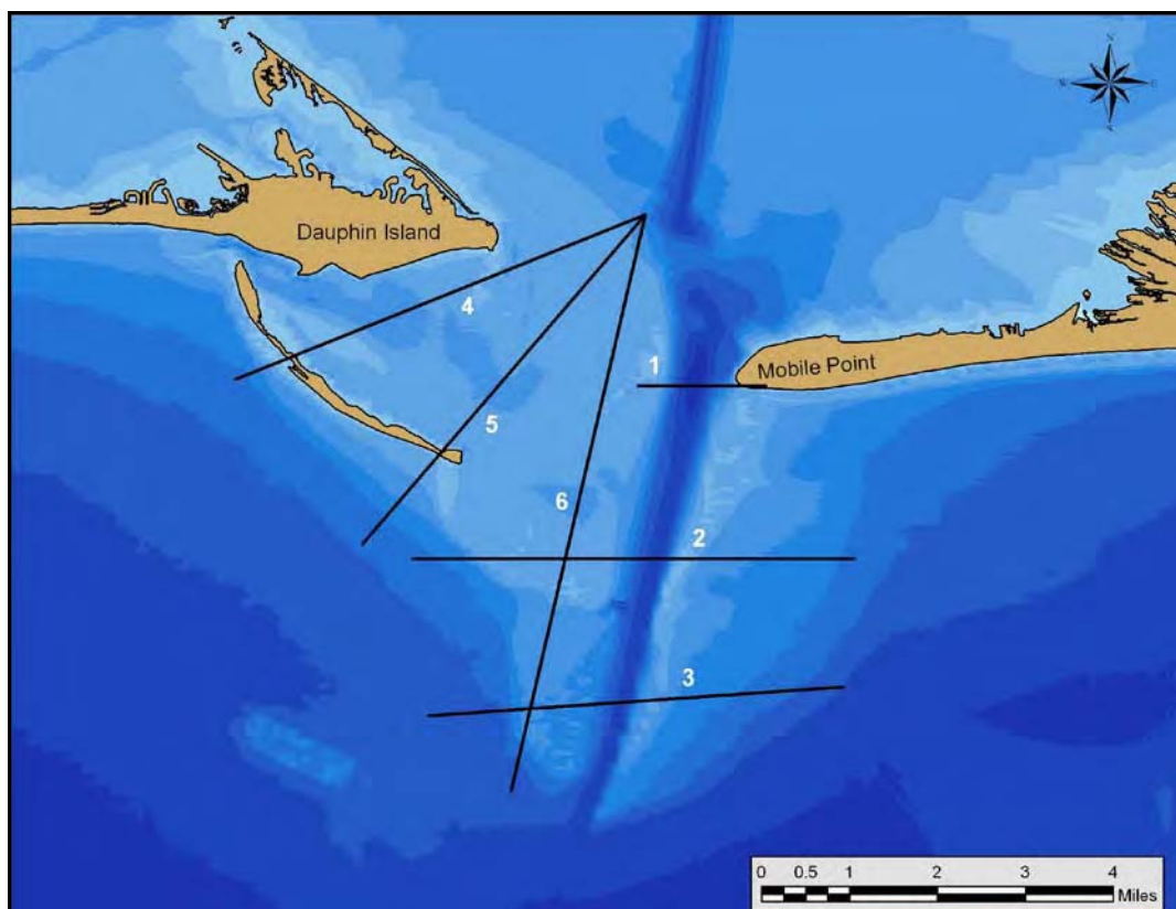
Figure 3-19. Transect locations on the Mobile ebb-tidal delta.
