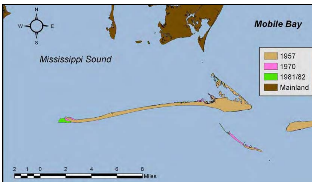
Figure 2-13. 1957 shoreline superimposed on 1970 and 1981/82 shorelines illustrating island movement on the ebb shoal to the northwest and lateral growth on western Dauphin Island.
