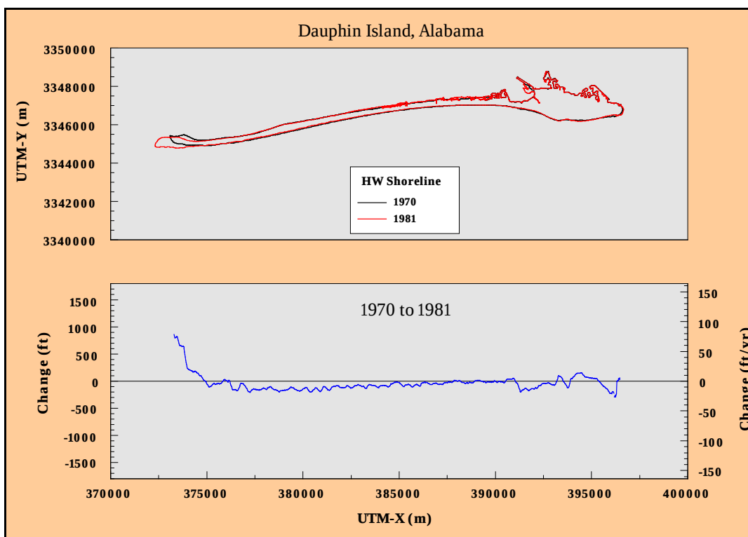
Figure C10. Historical shoreline position change, Dauphin Island, Alabama: 1970 to 1981.
