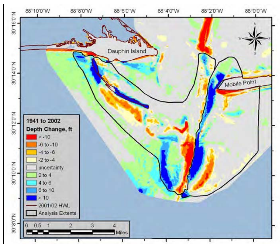
Figure G9. Analysis extent for calculating sand volume change – 1941 to 2002.
