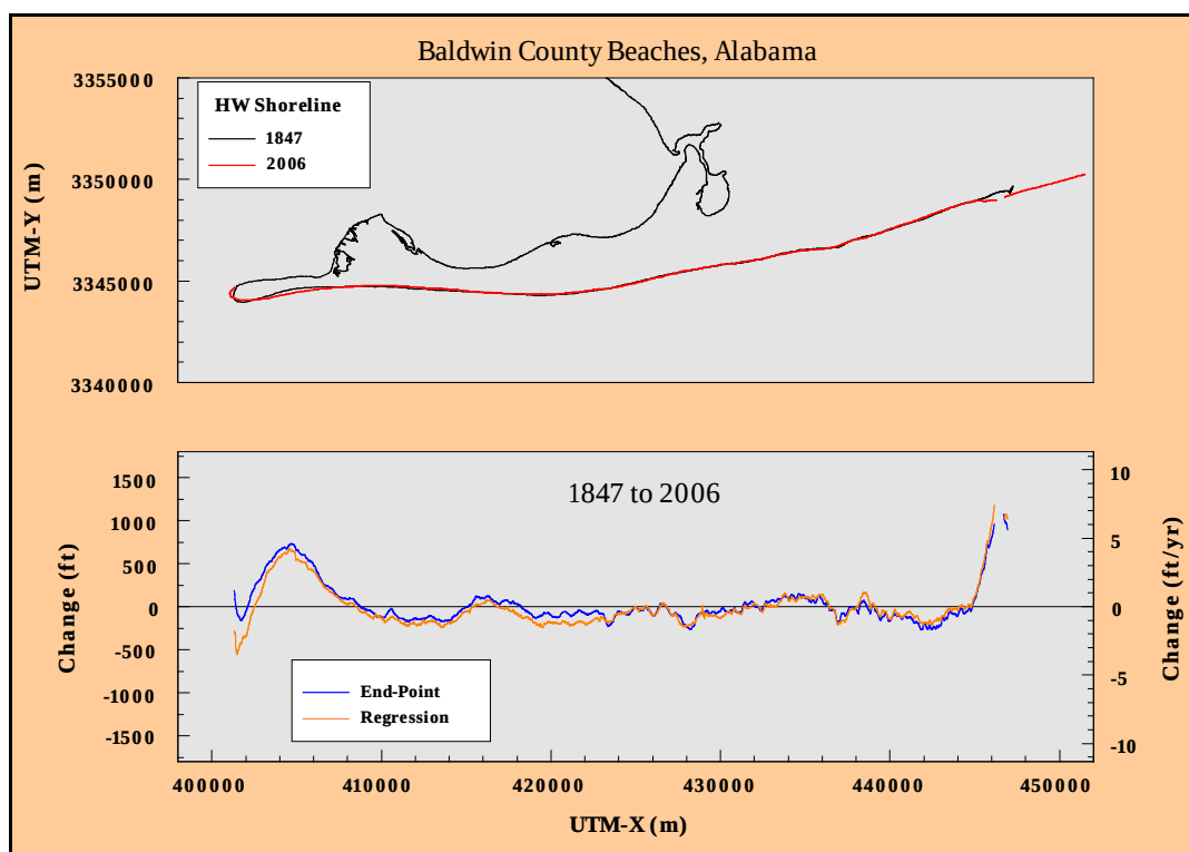
Figure D11. Historical shoreline position change, Perdido Pass to Mobile Point, Alabama: 1847 to 2006.
