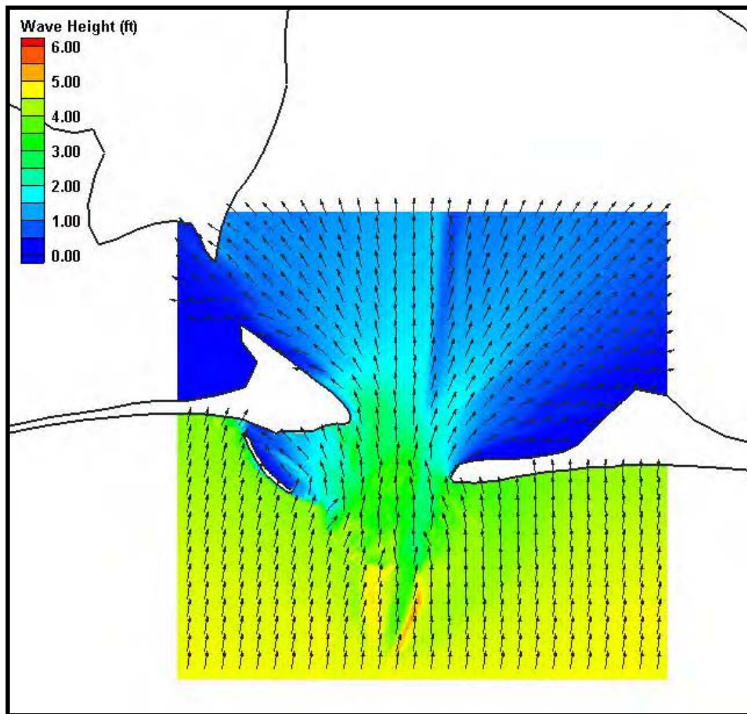
Figure H26. Fine grid (50m x 50m) wave results for Case 6, Mobile Pass. Wave heights are shown by color while wave direction is indicated by the arrow direction.
