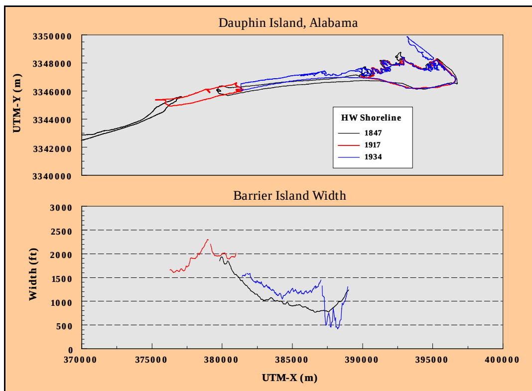
Figure 2-17. Changes in barrier island width between 1847 and 1934, Dauphin Island, AL.
