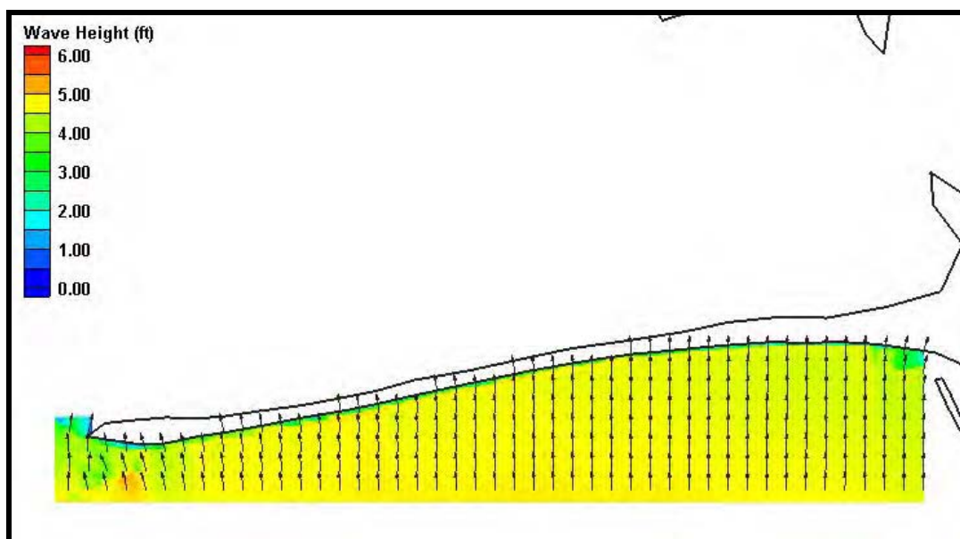
Figure H15. Fine grid (25m x 25m) wave results for Case 5, Dauphin Island. Wave heights are shown by color while wave direction is indicated by the arrow direction.
