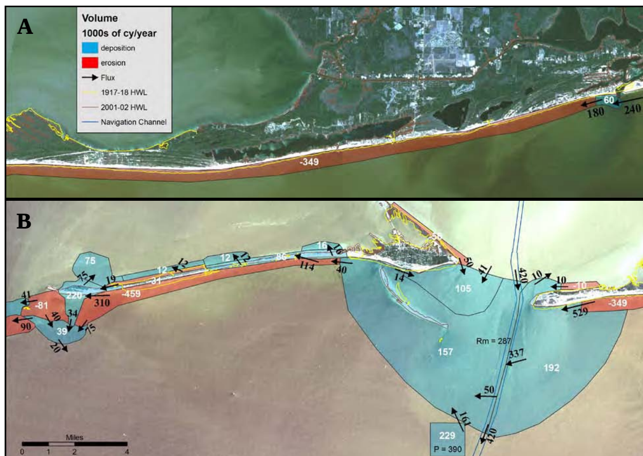
Figure 6-2. Sediment budget for the Alabama outer coast, 1917/20 to 1986/2002. A: Alabama coast between Perdido Pass in the east and western Morgan Peninsula; B – Alabama coast between western Morgan Peninsula and eastern Petit Bois Island, MS. White numbers indicate quantities eroded or deposited in thousands of cubic yards on an annual basis within defined polygons, and black numbers associated with black arrows are sediment fluxes in thousands of cubic yards per year.
