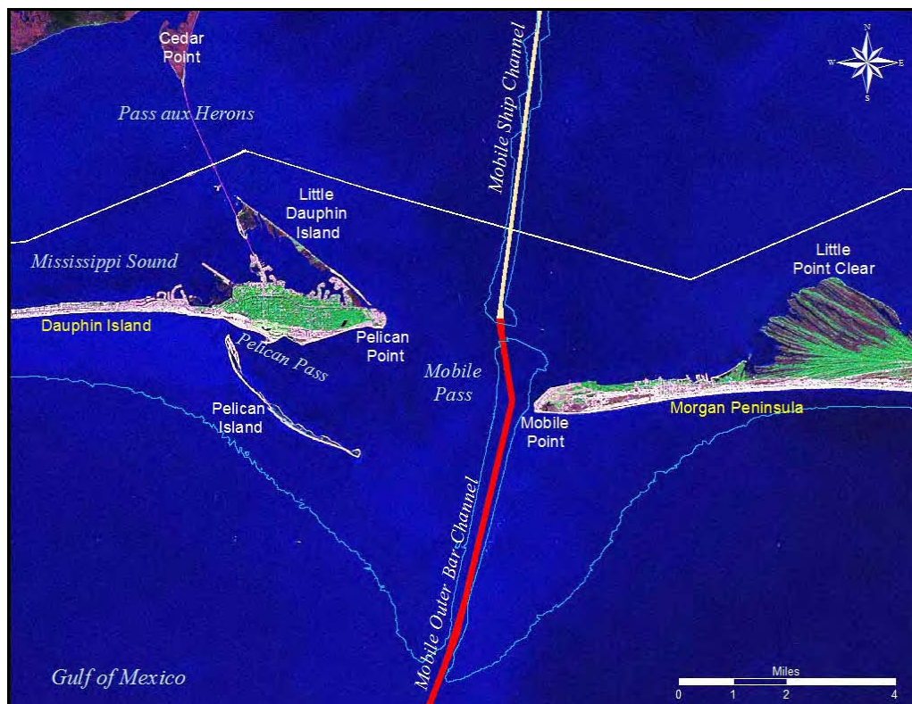
Figure 1-3. Mobile Pass and adjacent environments, including Mobile Outer Bar Channel and the 30-ft depth contour defining the seaward extent of the ebb-tidal delta and the Mobil Outer Mound disposal site.
