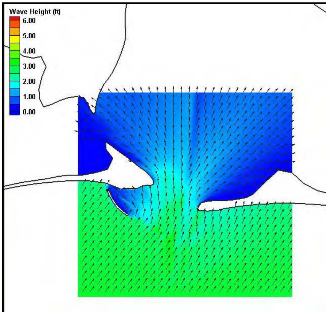
Figure H28. Fine grid (50m x 50m) wave results for Case 8, Mobile Pass. Wave heights are shown by color while wave direction is indicated by the arrow direction.
