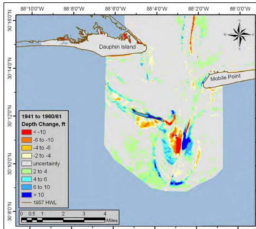
Figure 4-7. Bathymetric changes on the Mobile ebb-tidal delta, 1941 to 1960/61.
