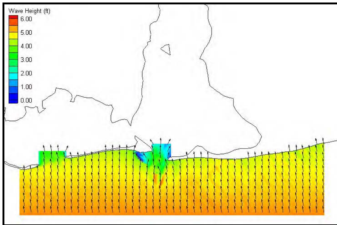
Figure 5-7. Coarse grid (200 m x 200 m) wave results for Case 5. Wave heights are shown by color while wave direction is indicated by the arrow direction.
