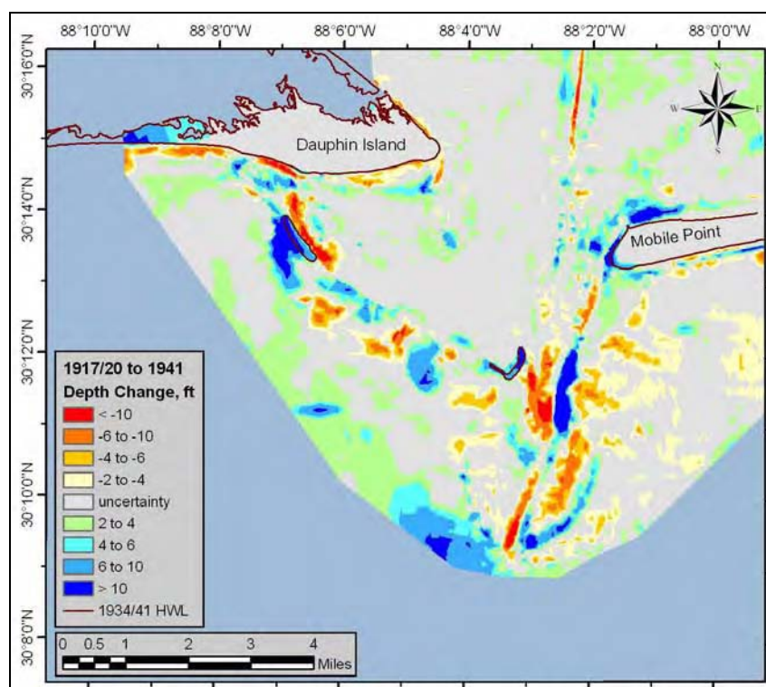
Figure 4-6. Bathymetric change after the July 1916 hurricane illustrating deposition along the eastern margin of the channel, minor island and shoal formation to the west of the channel, and deposition west of the outer mouth bar channel illustrating the offshore dredged material disposal site.
