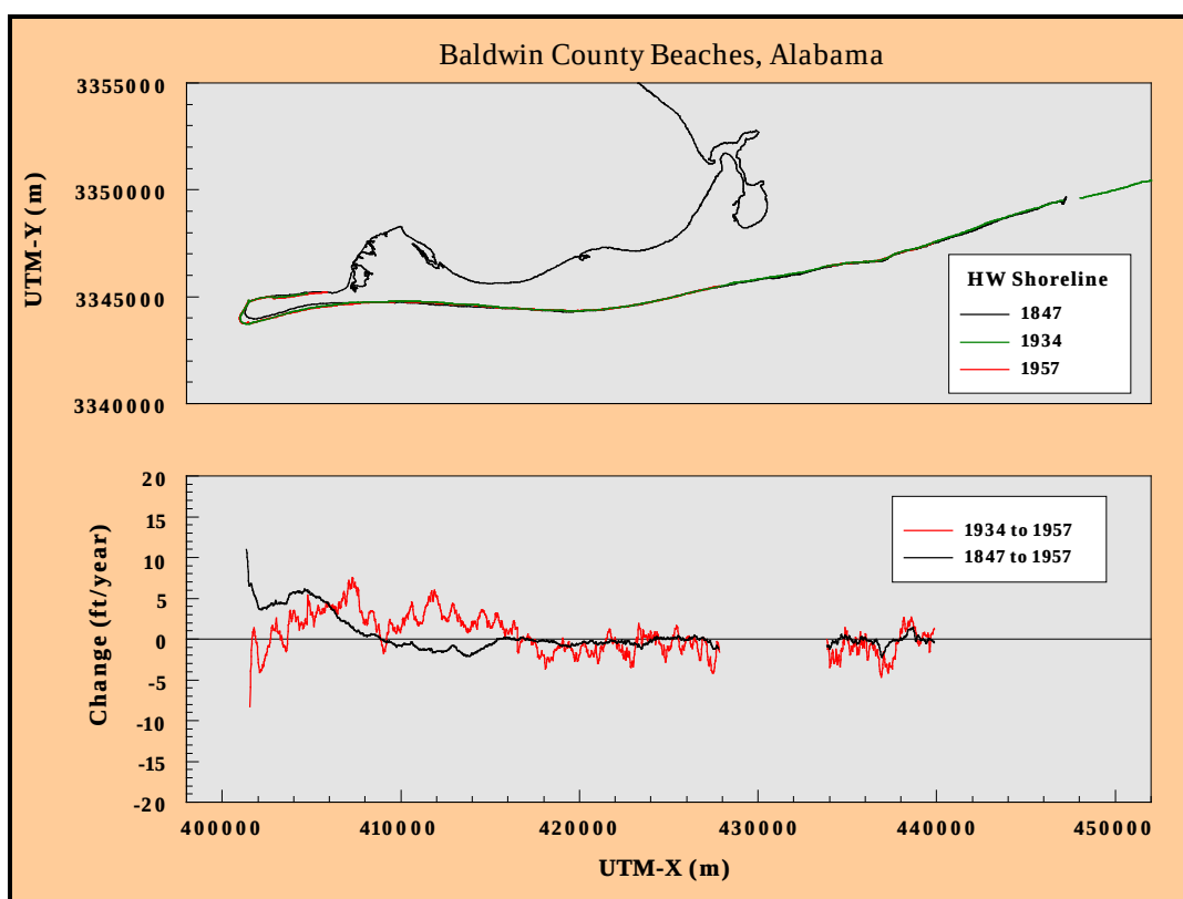
Figure 2-32. Gulf shoreline change between 1934 and 1957 relative to long-term trends between Perdido Pass and Mobile Point, Alabama.
