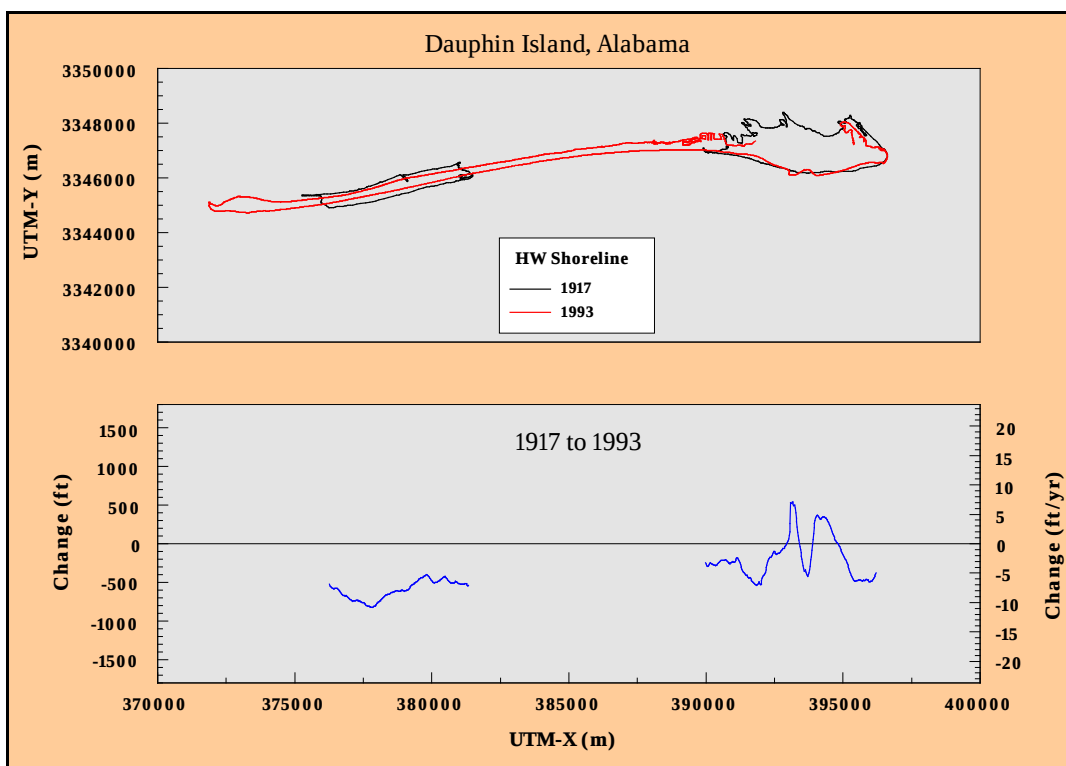
Figure C14. Historical shoreline position change, Dauphin Island, Alabama: 1917 to 1993.
