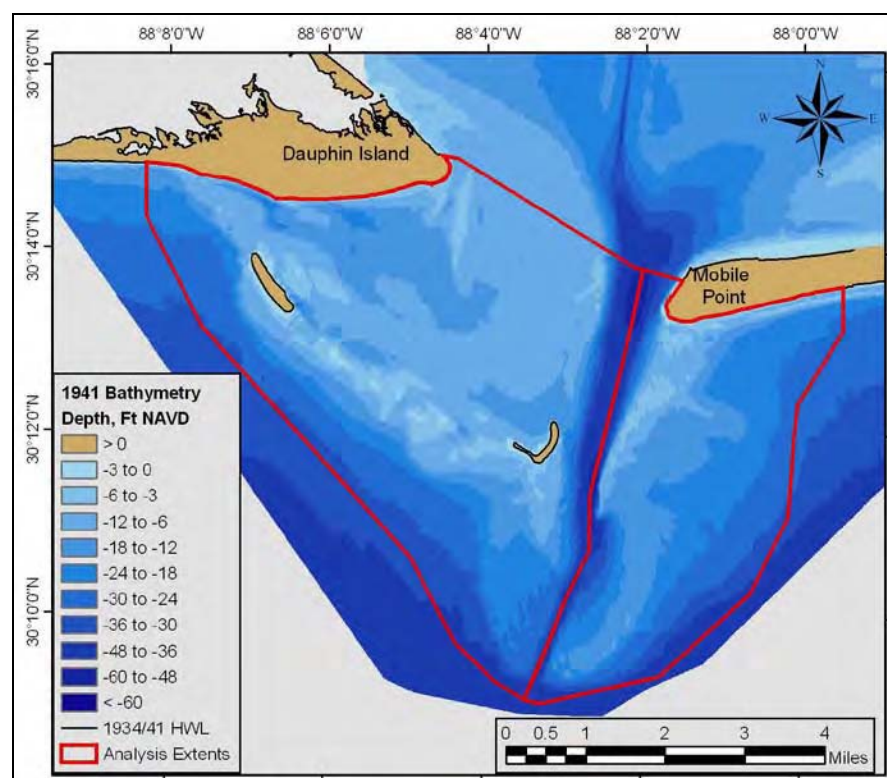
Figure F5. Analysis extent for calculating sand volume above 30-ft depth contour – 1941.
