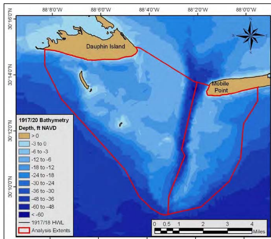
Figure F4. Analysis extent for calculating sand volume above 30-ft depth contour – 1917/20.
