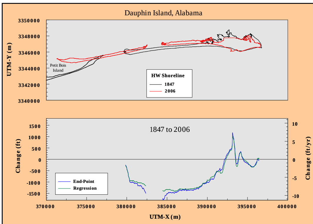
Figure C21. Historical shoreline position change, Dauphin Island, Alabama: 1847 to 2006.
