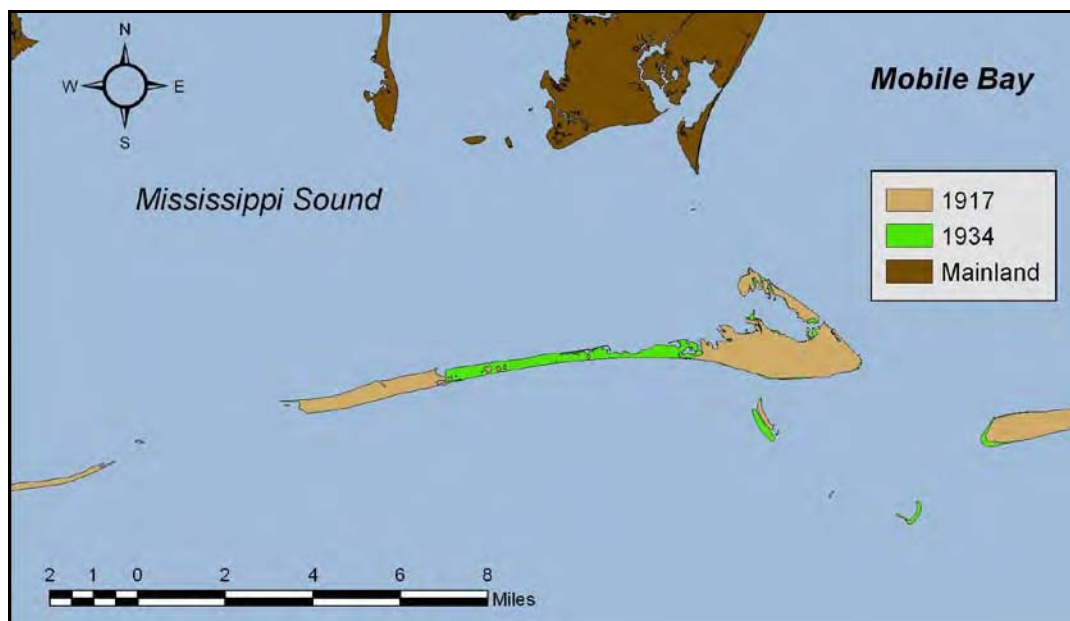
Figure 2-10. 1917 shoreline superimposed on 1934 shoreline illustrating complete infilling of the hurricane breach formed in 1916. Partial recovery of subaerial deposits on the ebb shoal is illustrated by the re-emergence of Sand Island by 1934.
