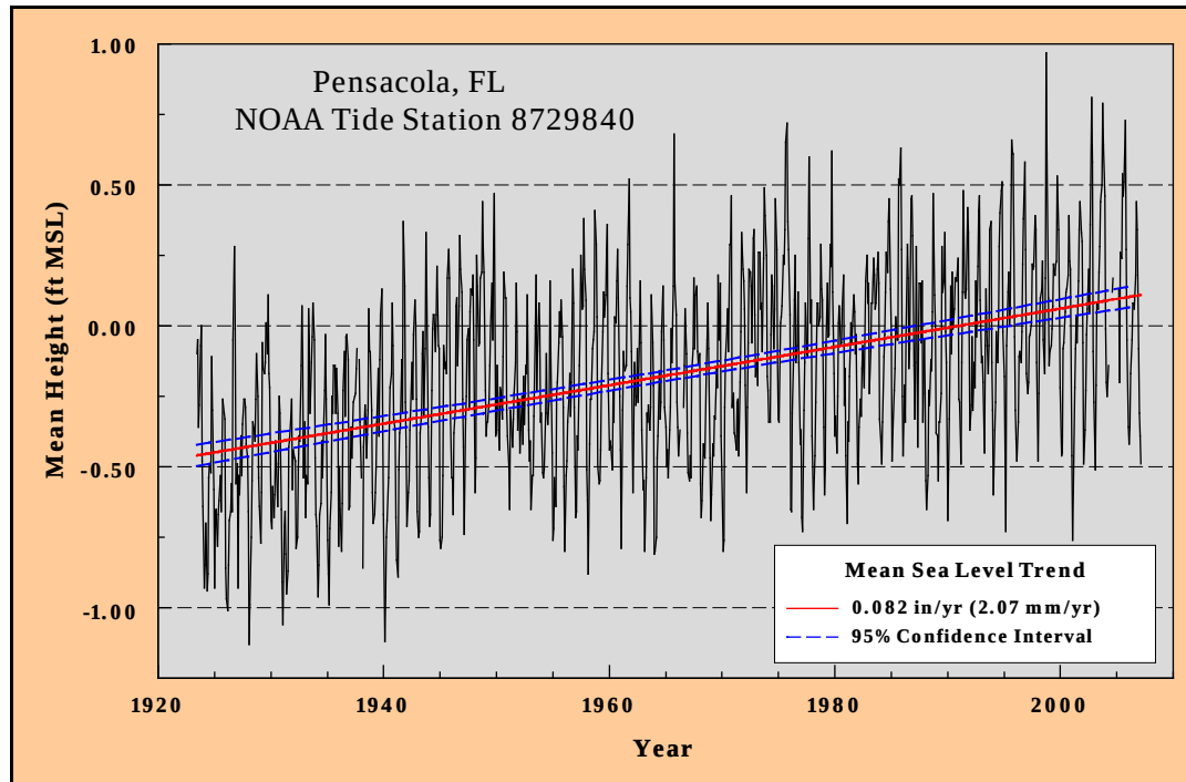
Figure 2-40. Monthly mean water level measurements at Pensacola, FL gauge 8729840, 1923 to 2007.
