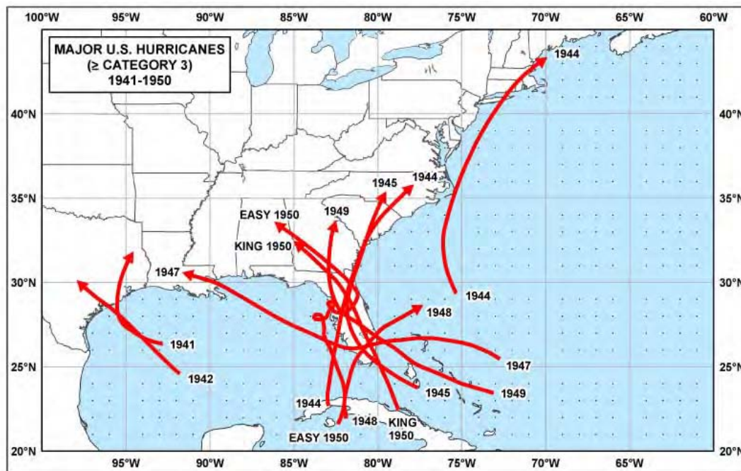
Figure A10. Hurricanes stronger than or equal to category 3 for the Gulf and Atlantic coasts – 1941 to 1950 (Blake et al. 2005).
