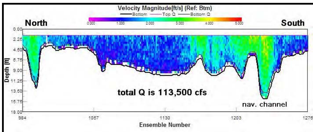
Figure 5-19. Color contour plot of velocities in Pass aux herons during maximum flood tide conditions.
