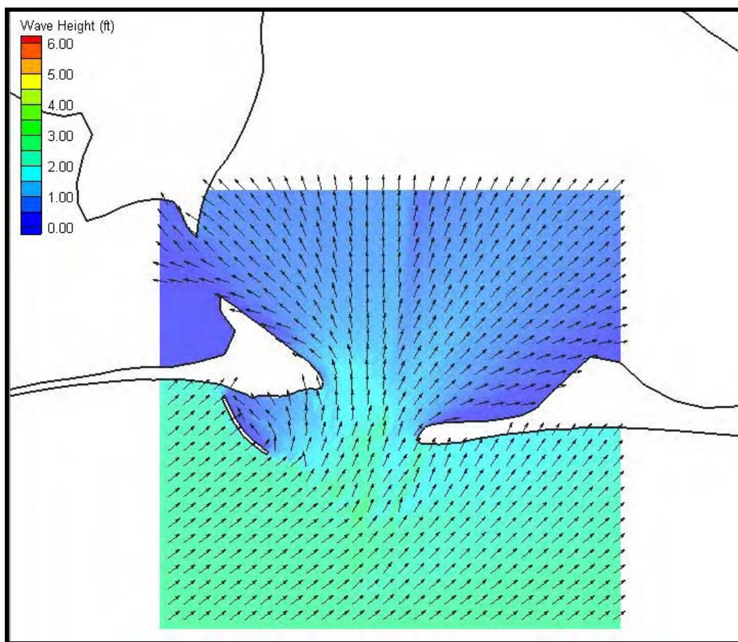
Figure 5-12. Fine grid (50 m x 50 m) wave results for Case 10, Mobile Pass. Wave heights are shown by color while wave direction is indicated by the arrow direction.
