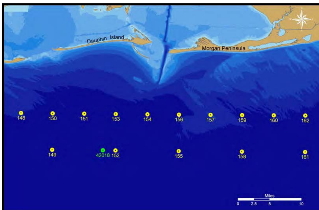
Figure 5-1. WIS stations in the study region are shown with yellow markers. NDBC Buoy 42018 is shown in green.
