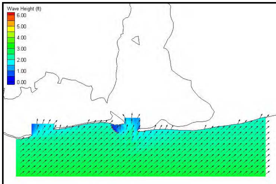
Figure 5-8. Coarse grid (200 m x 200 m) wave results for Case 10. Wave heights are shown by color while wave direction is indicated by the arrow direction.
