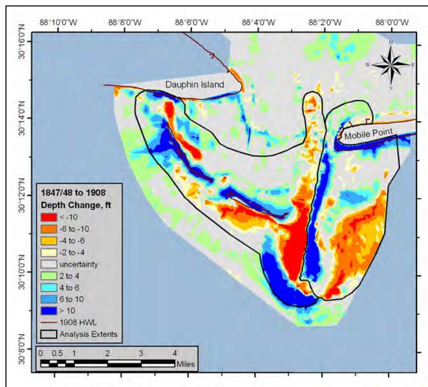
Figure G2. Analysis extent for calculating sand volume change – 1847/48 to 1908.
