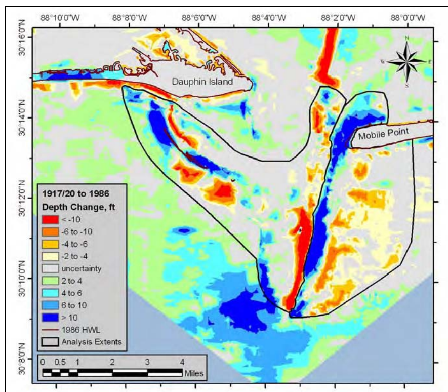
Figure G7. Analysis extent for calculating sand volume change – 1917/20 to 1986.
