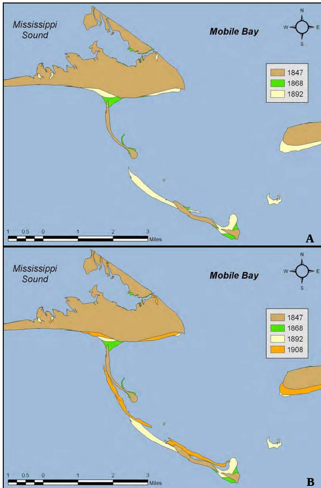
Figure 2-7. Shoreline and shoal evolution at and adjacent to eastern Dauphin Island and the west lobe of the ebb-tidal delta from 1847 to 1908.
