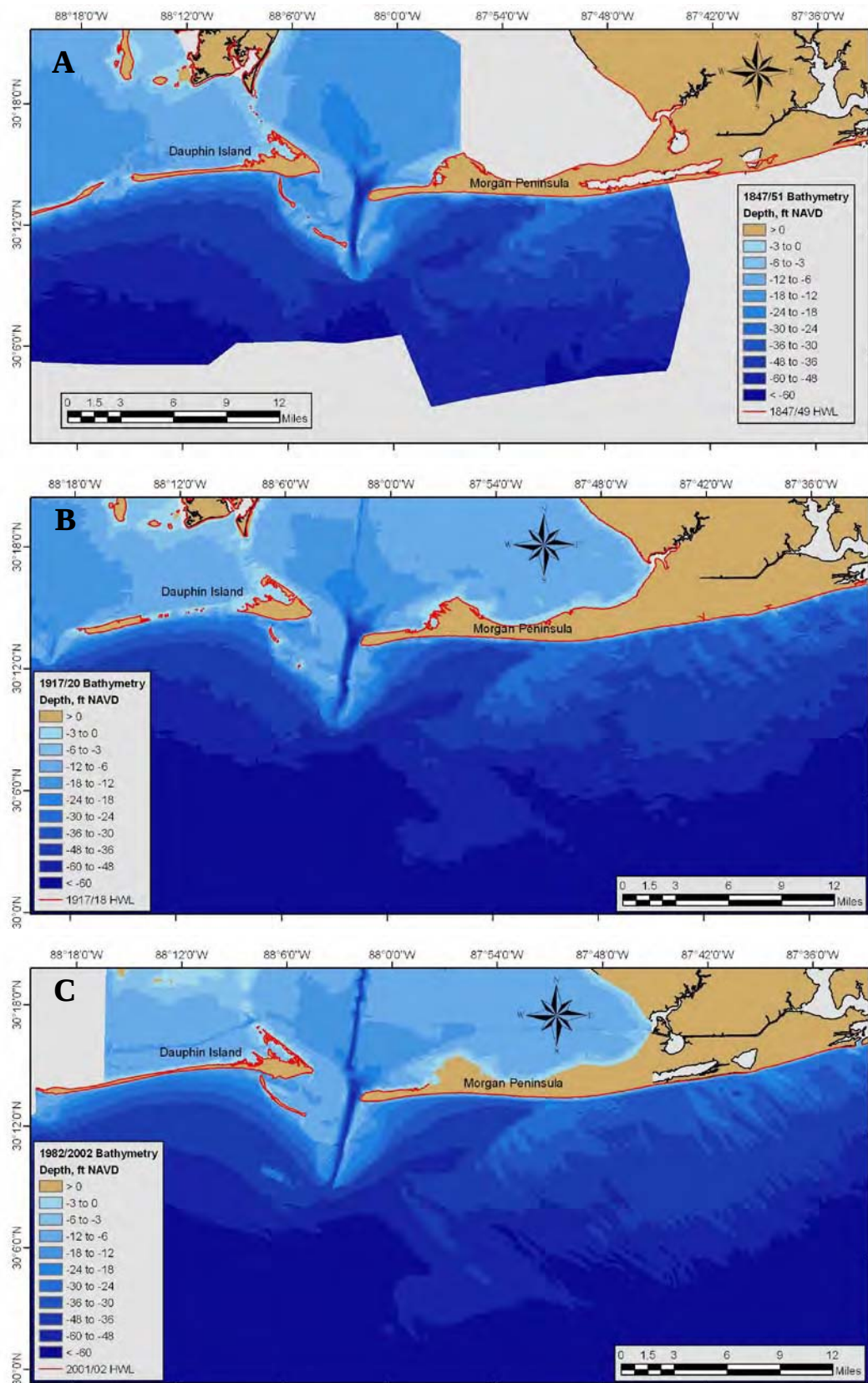
Figure 3-5. Regional bathymetric surfaces: A) 1847/51, B) 1917/20, C) 1982/2002.
