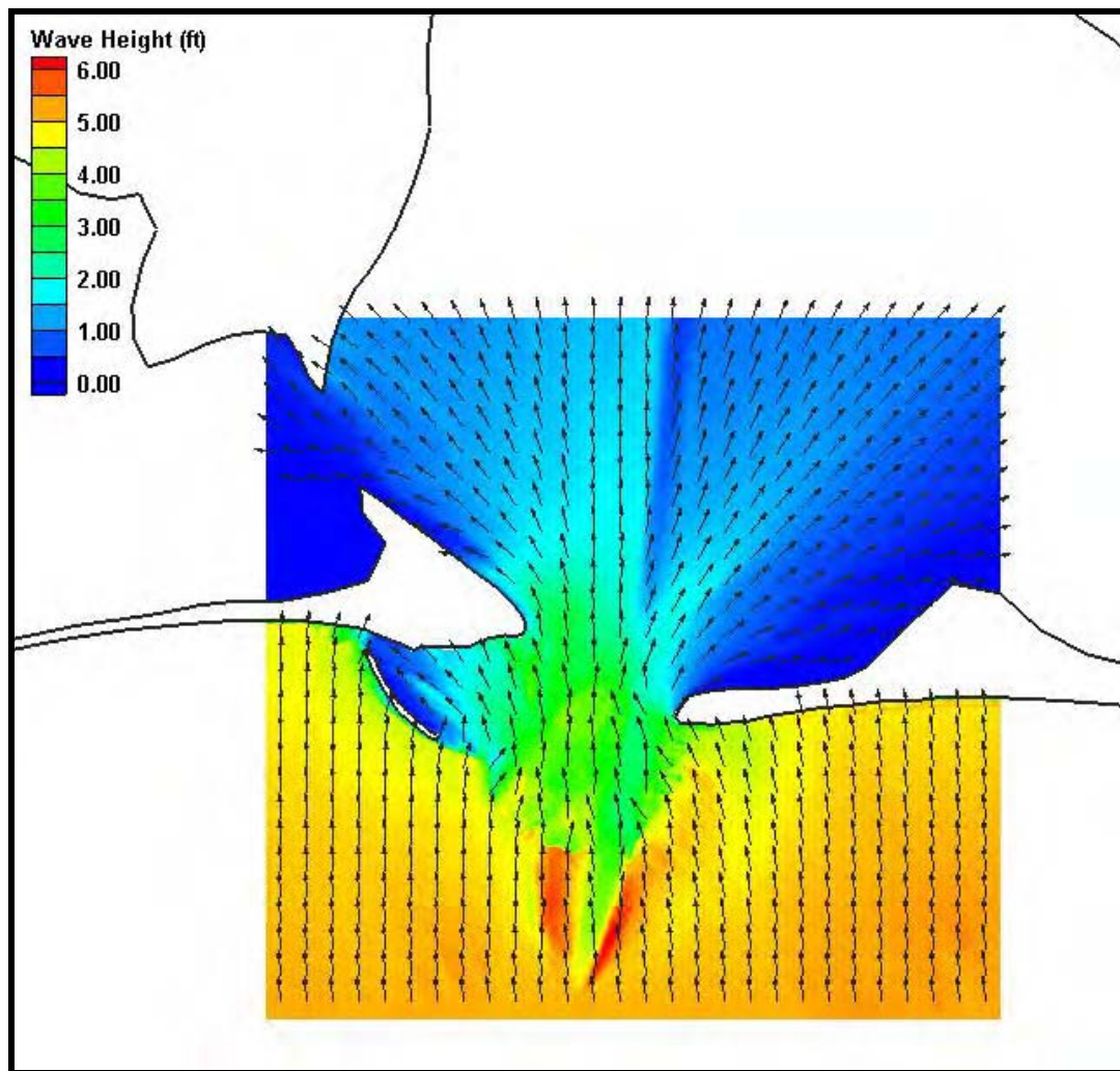
Figure H25. Fine grid (50m x 50m) wave results for Case 5, Mobile Pass. Wave heights are shown by color while wave direction is indicated by the arrow direction.
