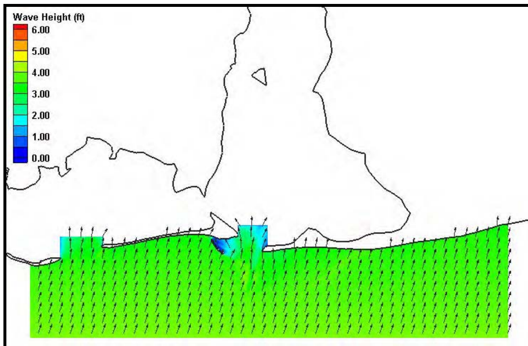
Figure H7. Coarse grid (200m x 200m) wave results for Case 7. Wave heights are shown by color while wave direction is indicated by the arrow direction.
