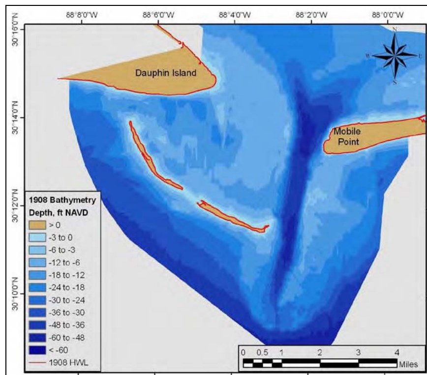
Figure 3-8. Bathymetric surface for Mobile Pass ebb-tidal delta and adjacent shores, 1908.
