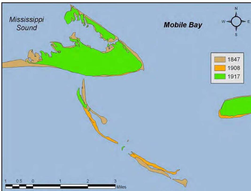
Figure 2-9. 1917 shoreline superimposed on 1847 and 1908 shorelines illustrating impact of the July 1916 hurricane on island evolution. Near-complete removal of subaerial sand from Pelican and Sand Islands and the eastern extent of island breaching are well documented.
