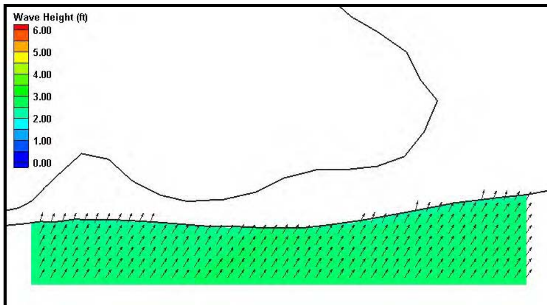
Figure H38. Fine grid (25m x 25m) wave results for Case 8, Morgan Peninsula. Wave heights are shown by color while wave direction is indicated by the arrow direction.
