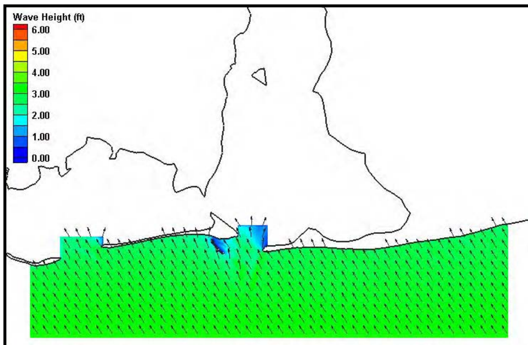
Figure H3. Coarse grid (200m x 200m) wave results for Case 3. Wave heights are shown by color while wave direction is indicated by the arrow direction.
