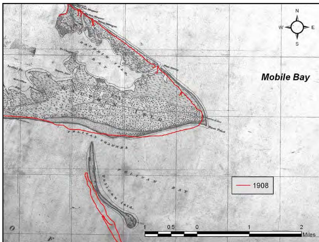
Figure 2-8. 1908 shoreline superimposed on T-sheet 240 (1847) illustrating shoreline erosion on the northeast-facing bay beaches of Dauphin Island and deposition along the south-facing beaches north of Pelican Island.
