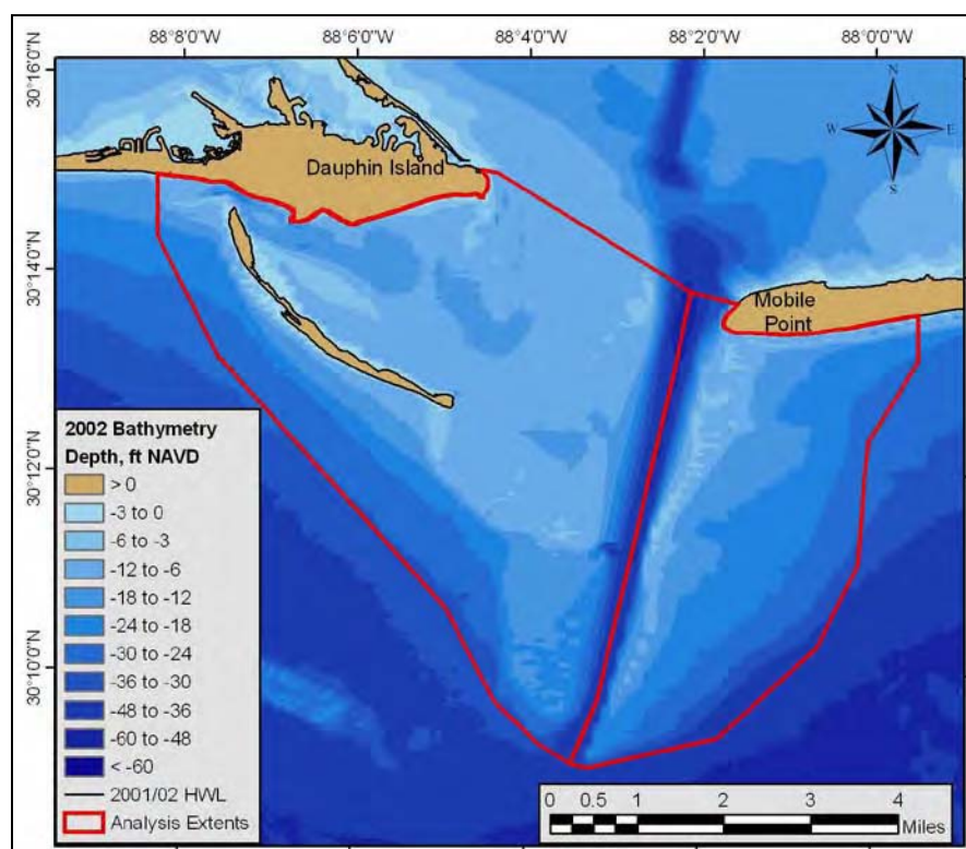
Figure F7. Analysis extent for calculating sand volume above 30-ft depth contour – 2002.
