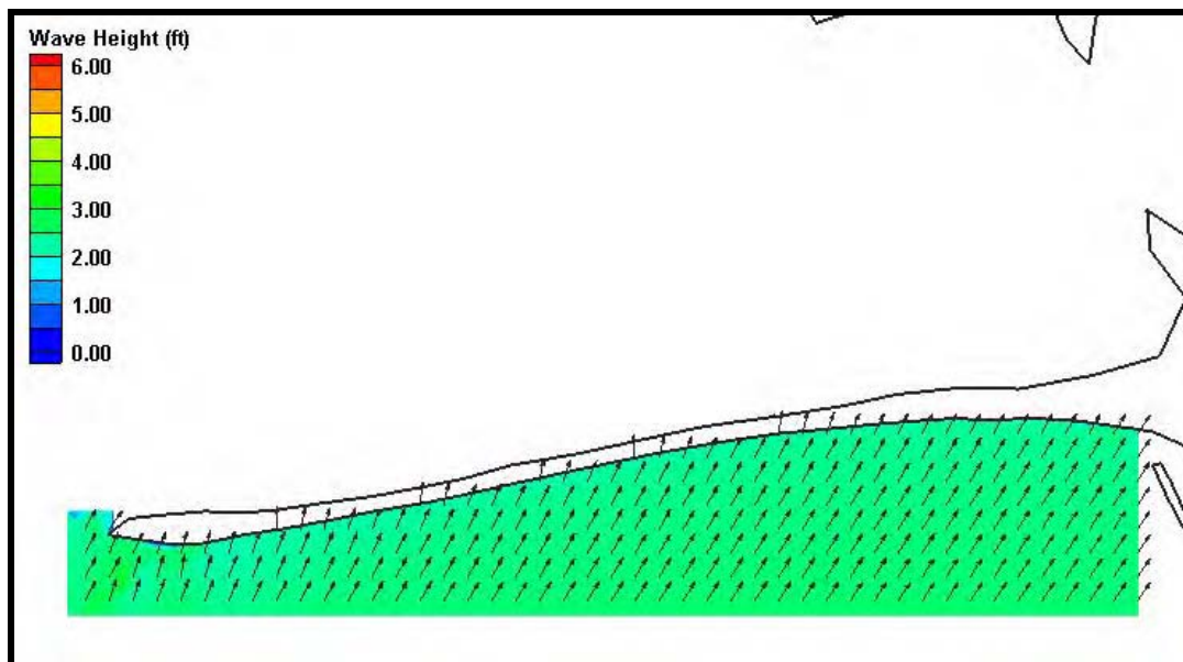
Figure H18. Fine grid (25m x 25m) wave results for Case 8, Dauphin Island. Wave heights are shown by color while wave direction is indicated by the arrow direction.
