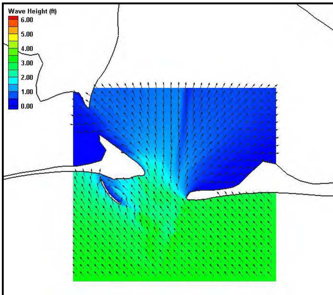
Figure H22. Fine grid (50m x 50m) wave results for Case 2, Mobile Pass. Wave heights are shown by color while wave direction is indicated by the arrow direction.
