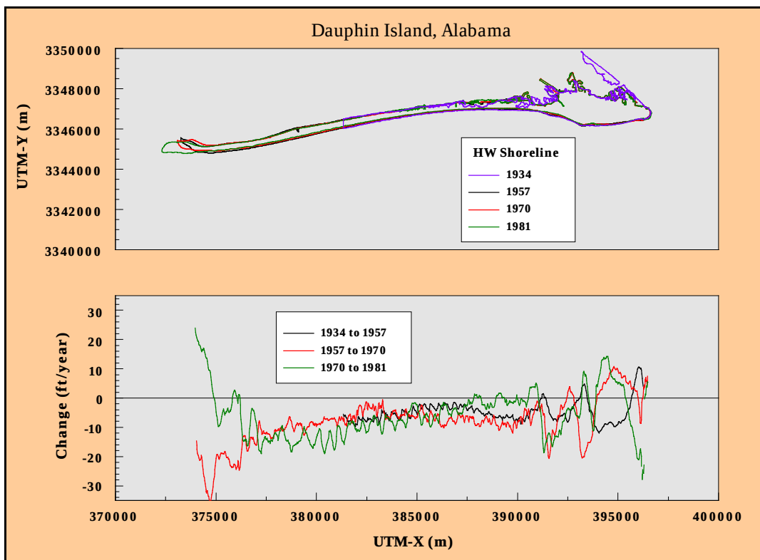
Figure 2-29. Gulf shoreline change between 1934 and 1981 illustrating net recession along the central portion of the island most vulnerable to overtopping during storms.
