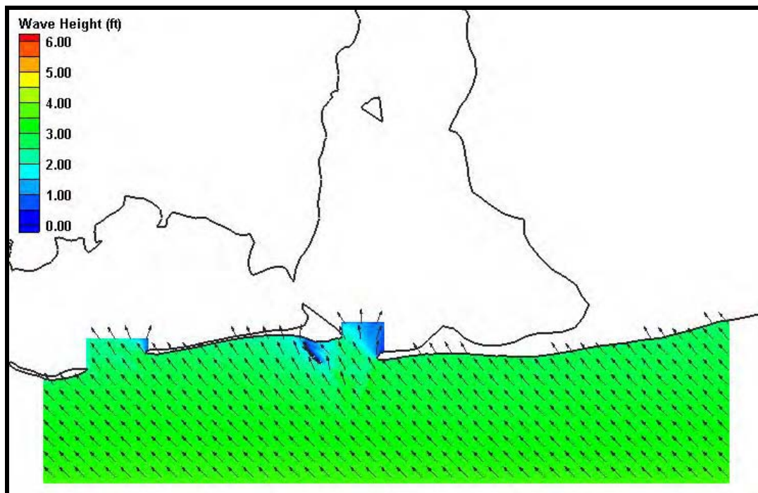
Figure H2. Coarse grid (200m x 200m) wave results for Case 2. Wave heights are shown by color while wave direction is indicated by the arrow direction.
