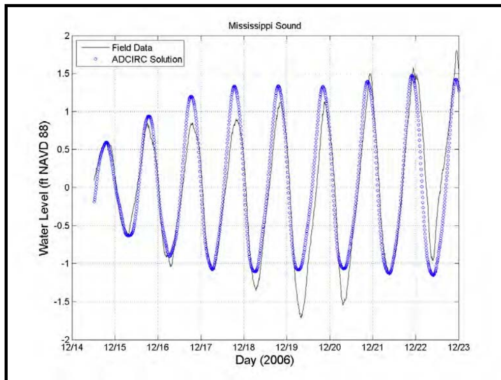
Figure 5-23. Comparison of modeled water levels with measured data for Mississippi Sound, December 15, 2006 to December 23, 2006.
