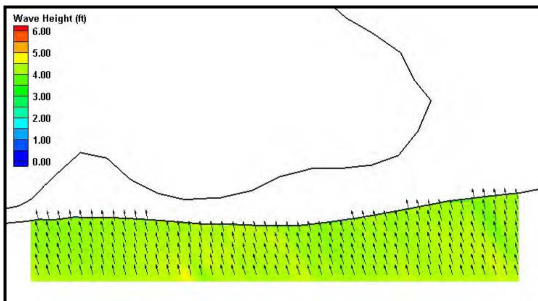
Figure H34. Fine grid (25m x 25m) wave results for Case 4, Morgan Peninsula. Wave heights are shown by color while wave direction is indicated by the arrow direction.
