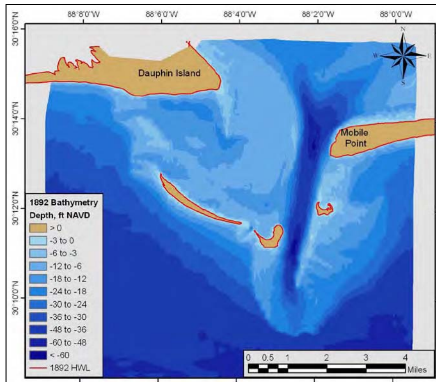
Figure 3-7. Bathymetric surface for Mobile Pass ebb-tidal delta and adjacent shores, 1892.
