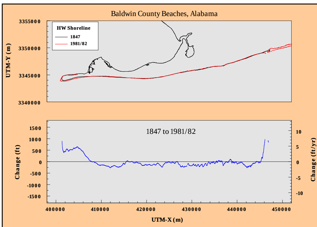
Figure D7. Historical shoreline position change, Perdido Pass to Mobile Point, Alabama: 1847 to 1981/82.
