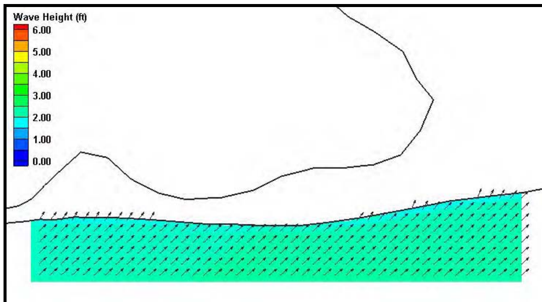
Figure H40. Fine grid (25m x 25m) wave results for Case 10, Morgan Peninsula. Wave heights are shown by color while wave direction is indicated by the arrow direction.
