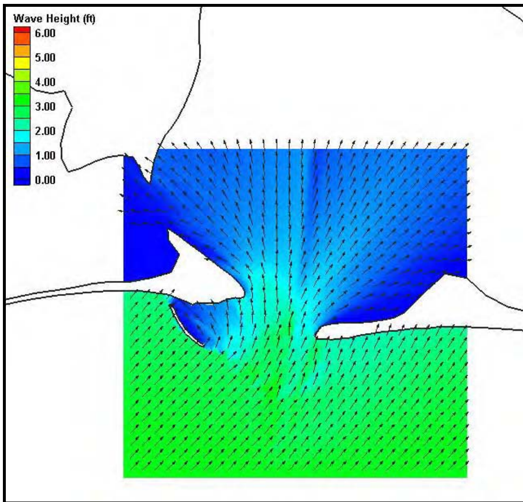
Figure H29. Fine grid (50m x 50m) wave results for Case 9, Mobile Pass. Wave heights are shown by color while wave direction is indicated by the arrow direction.
