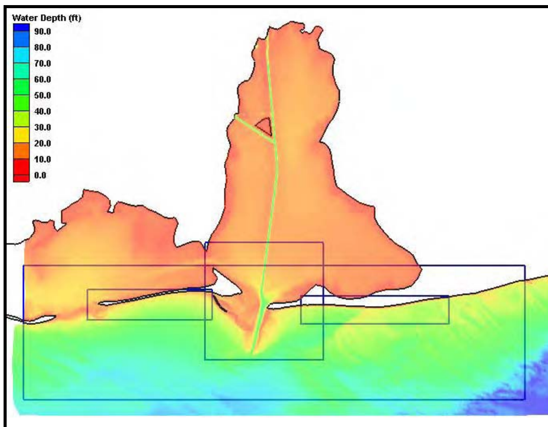
Figure 5-5. STWAVE bathymetry and model grid domains.
