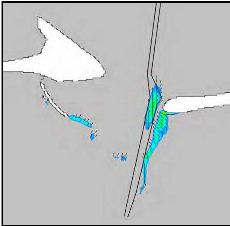
Figure 5-30. CMS-M2D average transport vectors for Case 2 during flood tide.
