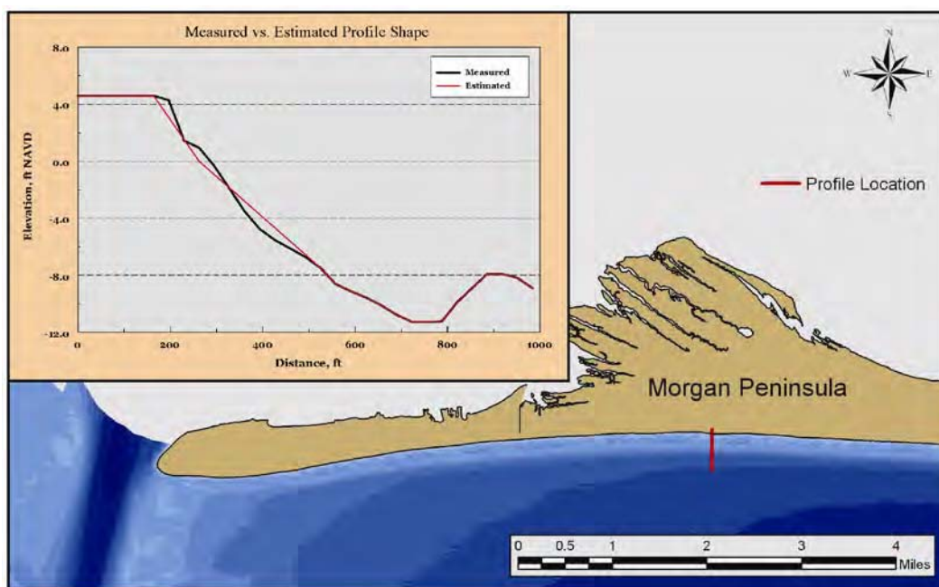
Figure 3-4. Comparison of measured profile elevations versus estimated profile shape using HWL to NAVD distance relationship derived from lidar and beach profile data.
