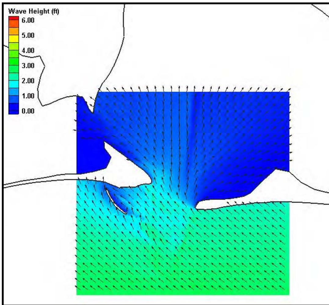
Figure H21. Fine grid (50m x 50m) wave results for Case 1, Mobile Pass. Wave heights are shown by color while wave direction is indicated by the arrow direction.
