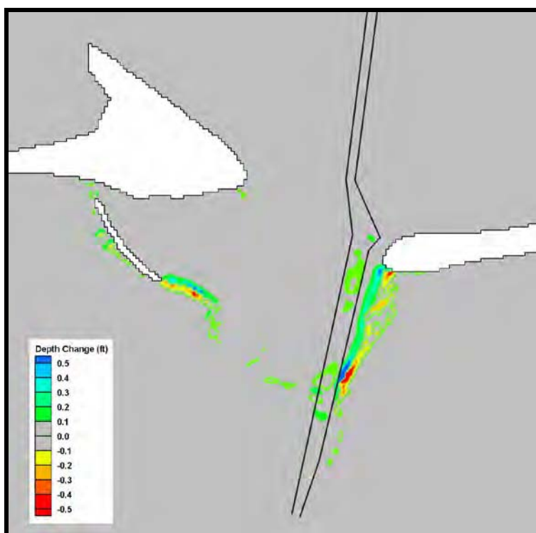
Figure 5-29. CMS-M2D bottom change results for 3 days of average tidal conditions under normal waves. Erosion is in yellow/red and accretion is in blue/green.
