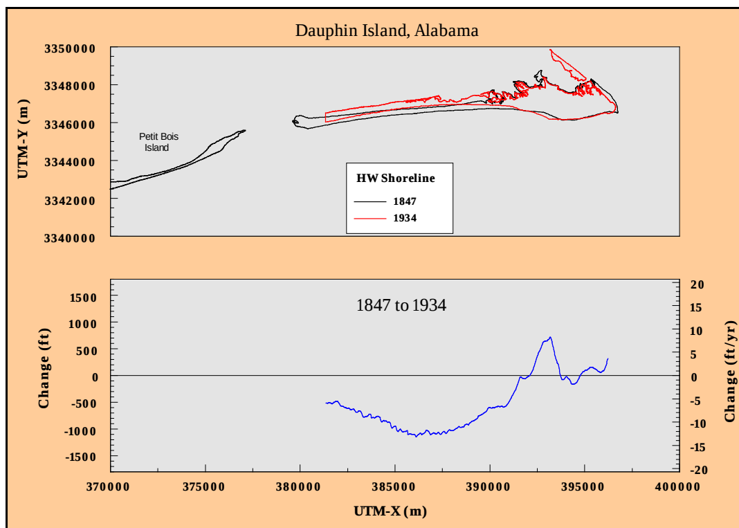
Figure C3. Historical shoreline position change, Dauphin Island, Alabama: 1847 to 1934.
