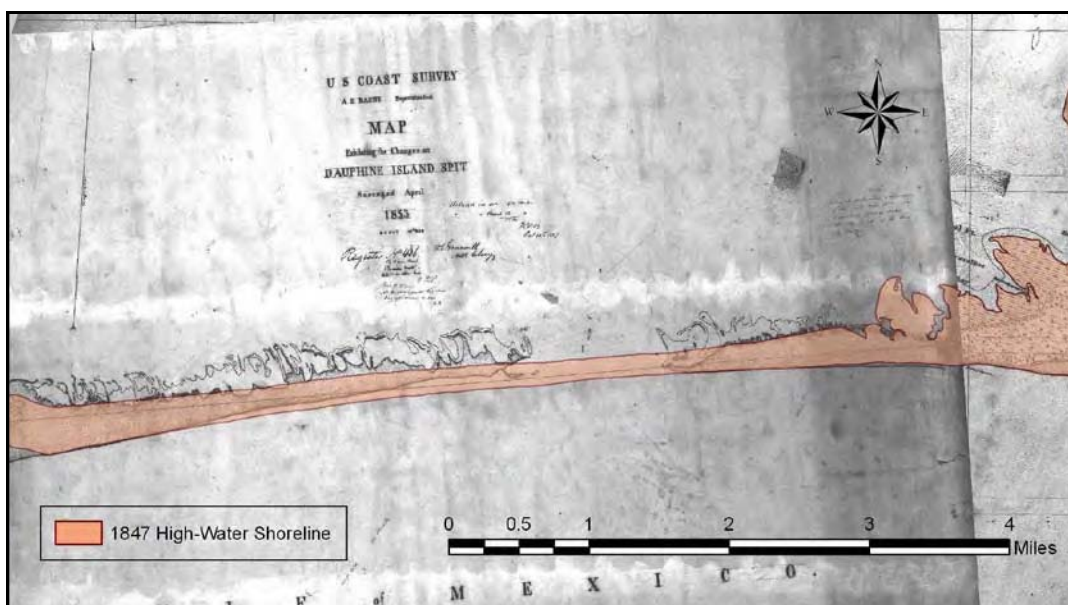
Figure 2-22. First-recorded breaching along the central portion of western Dauphin Island in response to the hurricane of 1852.
