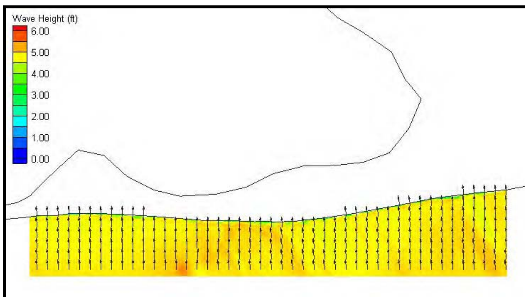
Figure 5-13. Fine grid (25 m x 25 m) wave results for Case 5, Morgan Peninsula. Wave heights are shown by color while wave direction is indicated by the arrow direction.
