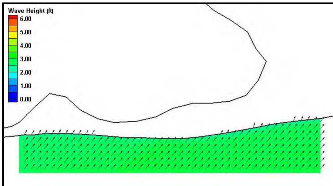
Figure H39. Fine grid (25m x 25m) wave results for Case 9, Morgan Peninsula. Wave heights are shown by color while wave direction is indicated by the arrow direction.
