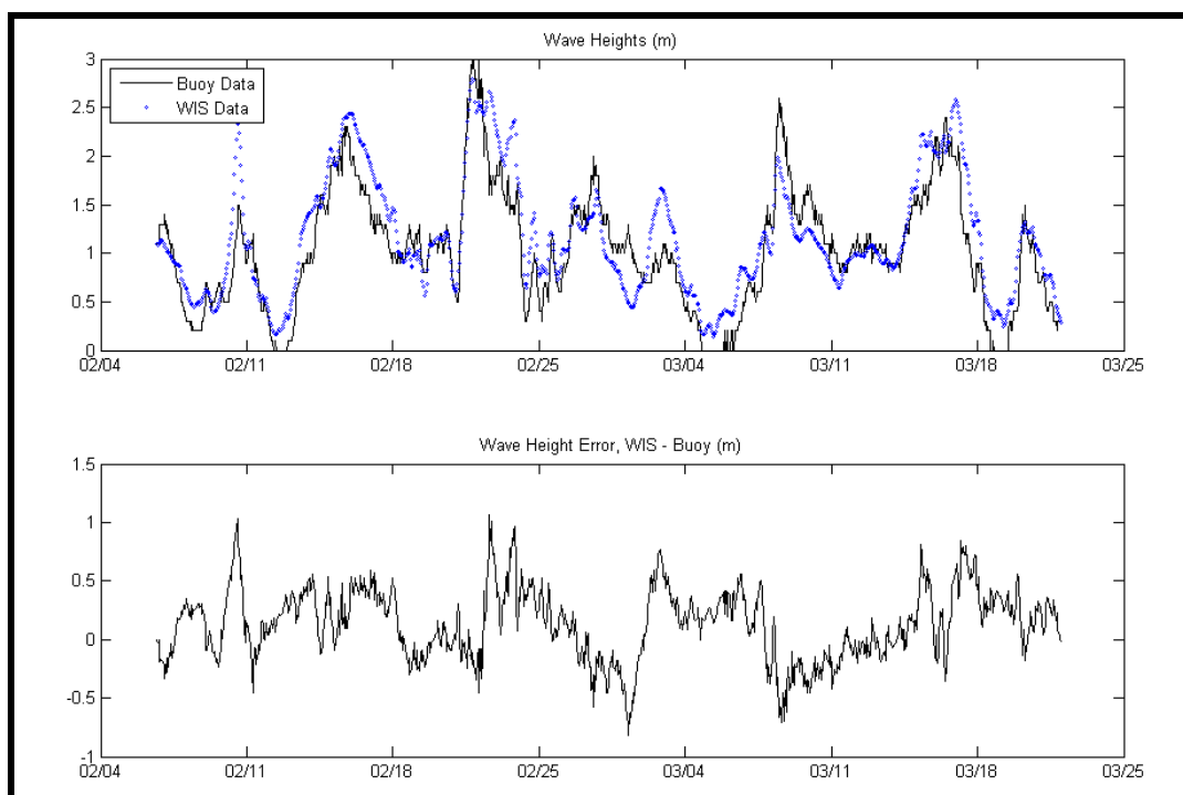
Figure 5-3. Wave height comparison between WIS Station 152 and NDBC Station 41018. The top panel illustrates WIS and NDBC wave height time series, and the bottom panel shows the error in WIS data reported as WIS prediction - Buoy measurement.
