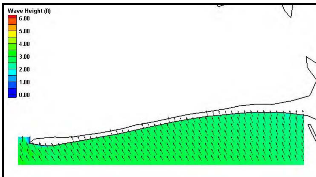
Figure H13. Fine grid (25m x 25m) wave results for Case 3, Dauphin Island. Wave heights are shown by color while wave direction is indicated by the arrow direction.
