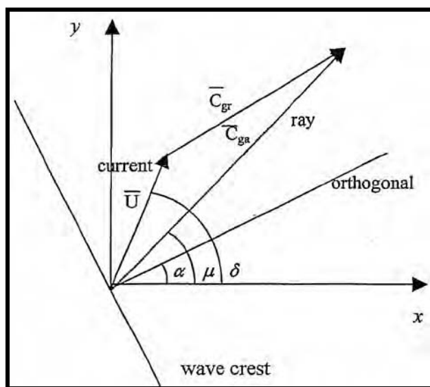
Figure 5-4. Wave and current vectors used in STWAVE.
