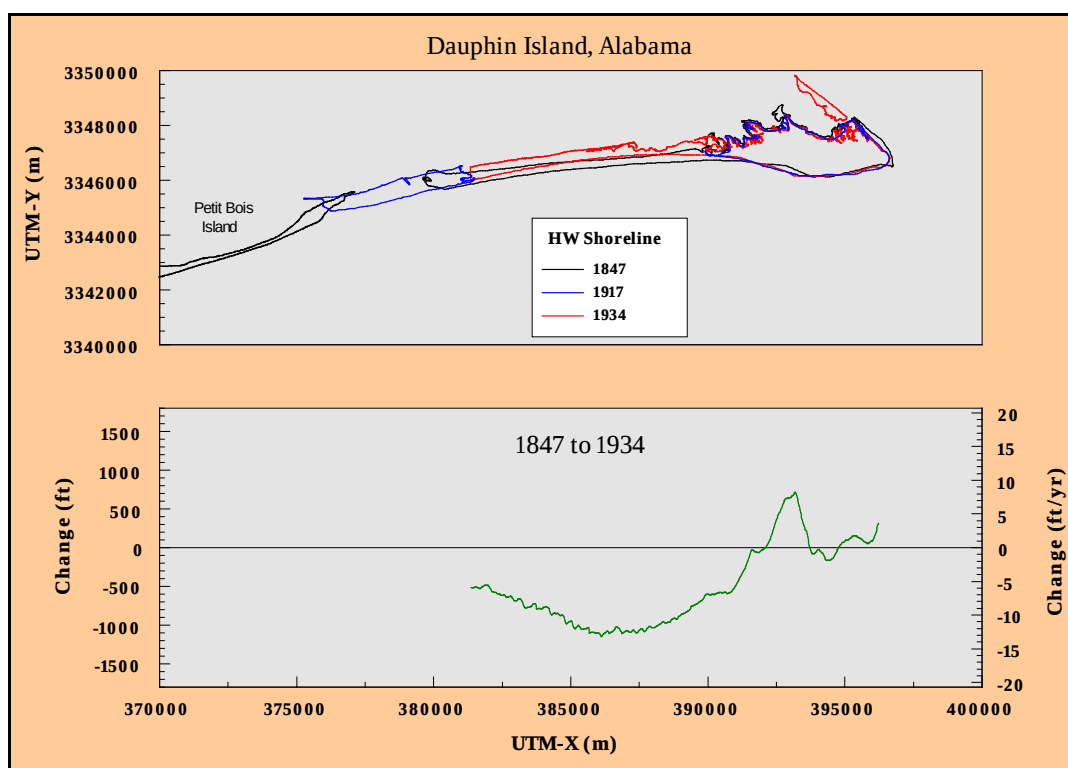
Figure 2-28. Breach infilling by 1934 created a continuous island that was displaced landward by about 1,100 ft of its position in 1847.
