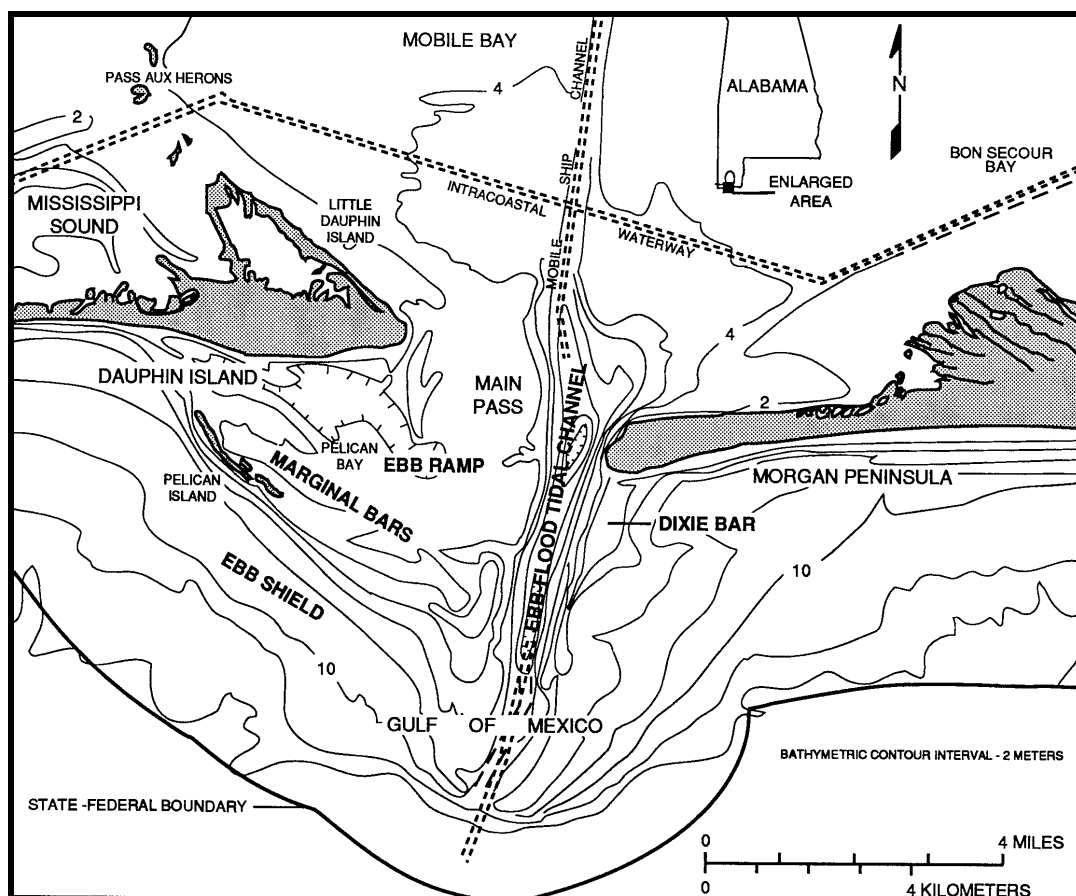
Figure 1-6. Geomorphology of the ebb-tidal delta seaward of Mobile Bay entrance (from Hummell, 1996).
