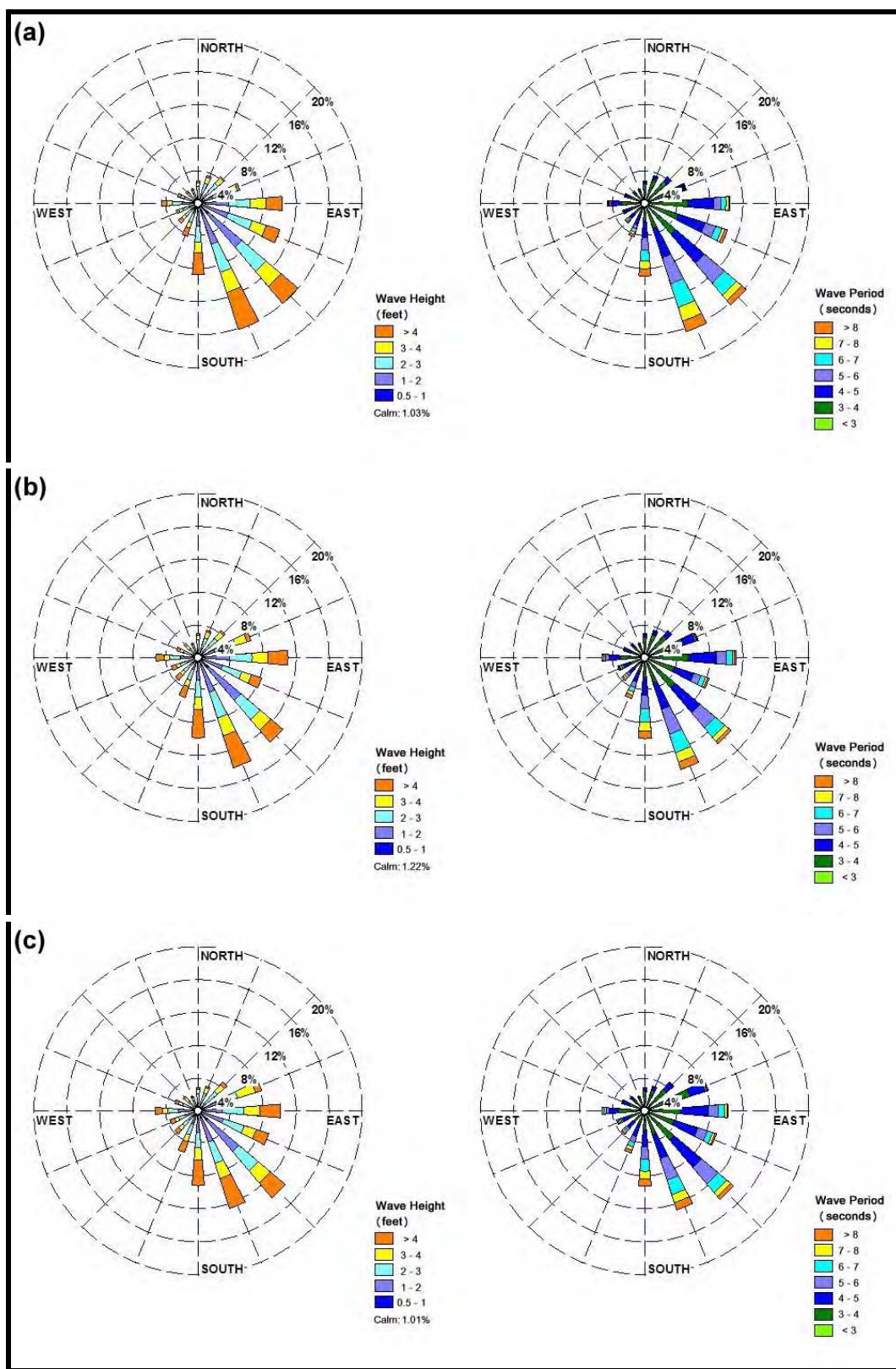
Figure 5-2. Wave height and period roses for (a) WIS station 148, (b) WIS station 156, and (c) WIS station 162.
