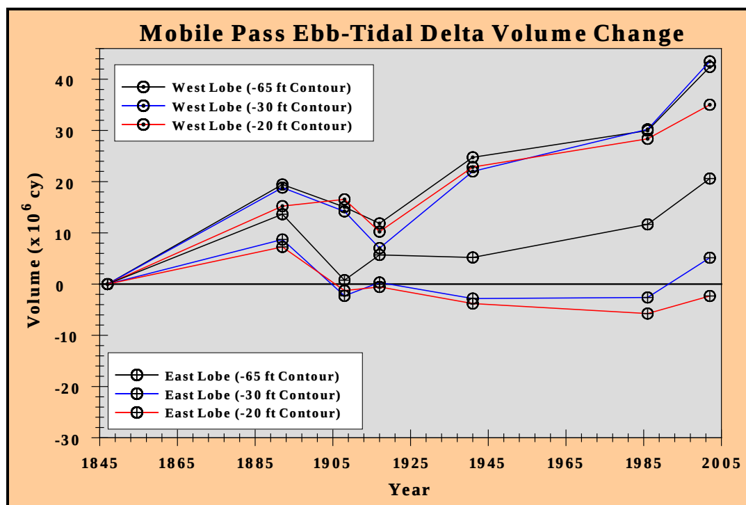
Figure 3-27. Plot of sediment volume change east and west of the channel for the Mobile Pass ebb-tidal delta, 1847/48 to 2002.
