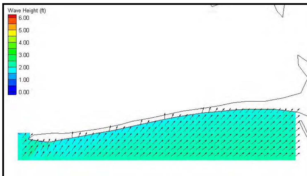
Figure 5-10. Fine grid (25 m x 25 m) wave results for Case 10, Dauphin Island. Wave heights are shown by color while wave direction is indicated by arrow direction.
