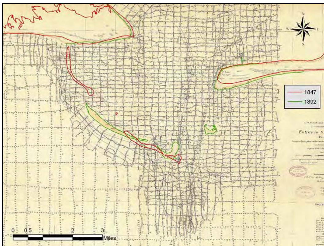
Figure 3-1. USC&GS bathymetry data coverage for the 1892 survey with overlays of the 1847 and 1892 high-water shorelines.
