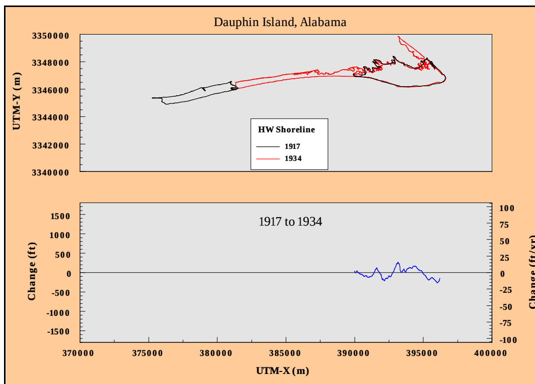
Figure C2. Historical shoreline position change, Dauphin Island, Alabama: 1917 to 1934.
