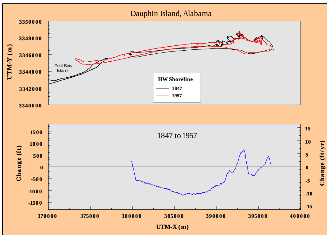
Figure C6. Historical shoreline position change, Dauphin Island, Alabama: 1847 to 1957.
