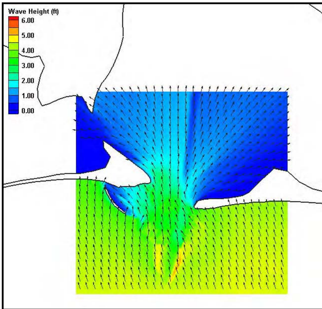
Figure H24. Fine grid (50m x 50m) wave results for Case 4, Mobile Pass. Wave heights are shown by color while wave direction is indicated by the arrow direction.
