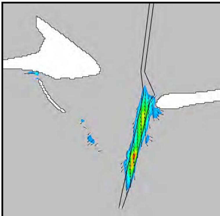
Figure 5-31. CMS-M2D average transport vectors for Case 2 during ebb tide.
