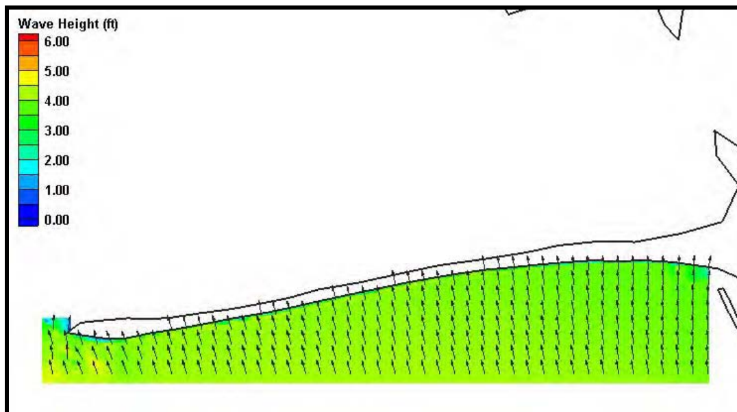
Figure H14. Fine grid (25m x 25m) wave results for Case 4, Dauphin Island. Wave heights are shown by color while wave direction is indicated by the arrow direction.
