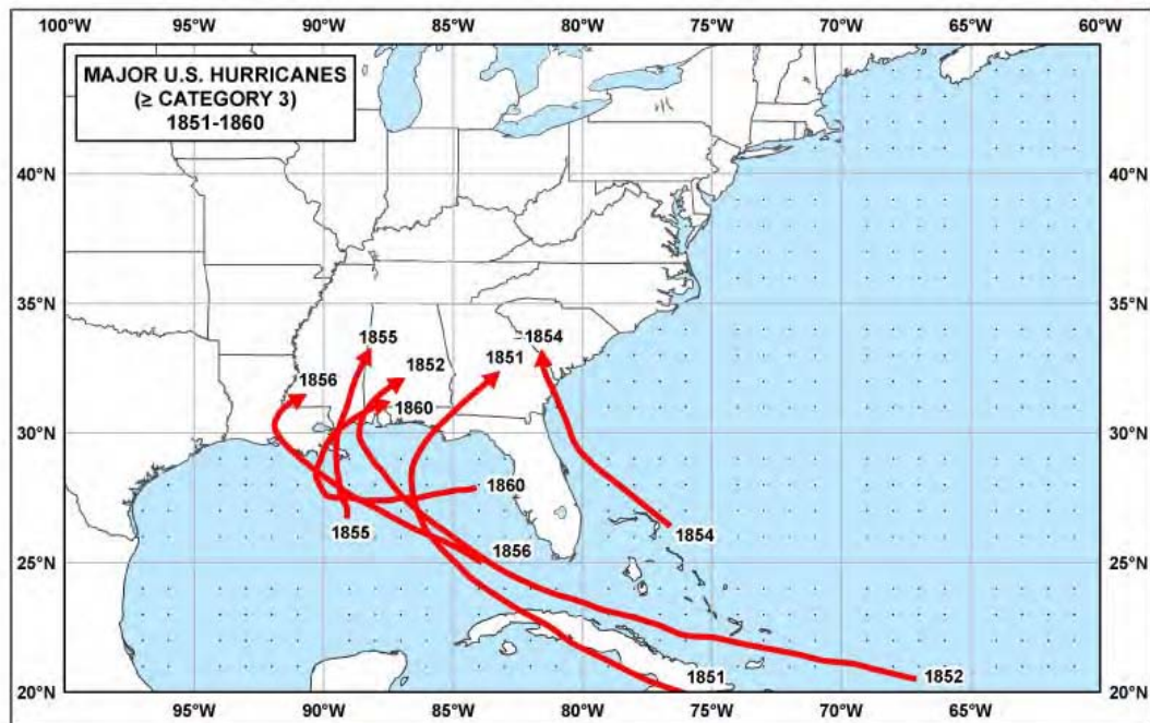
Figure A1. Hurricanes stronger than or equal to category 3 for the Gulf and Atlantic coasts – 1851 to 1860 (Blake et al. 2005).
