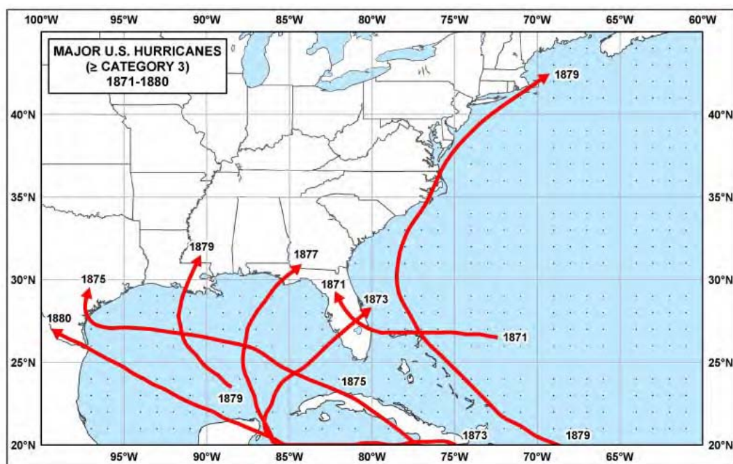
Figure A3. Hurricanes stronger than or equal to category 3 for the Gulf and Atlantic coasts – 1871 to 1880 (Blake et al. 2005).
