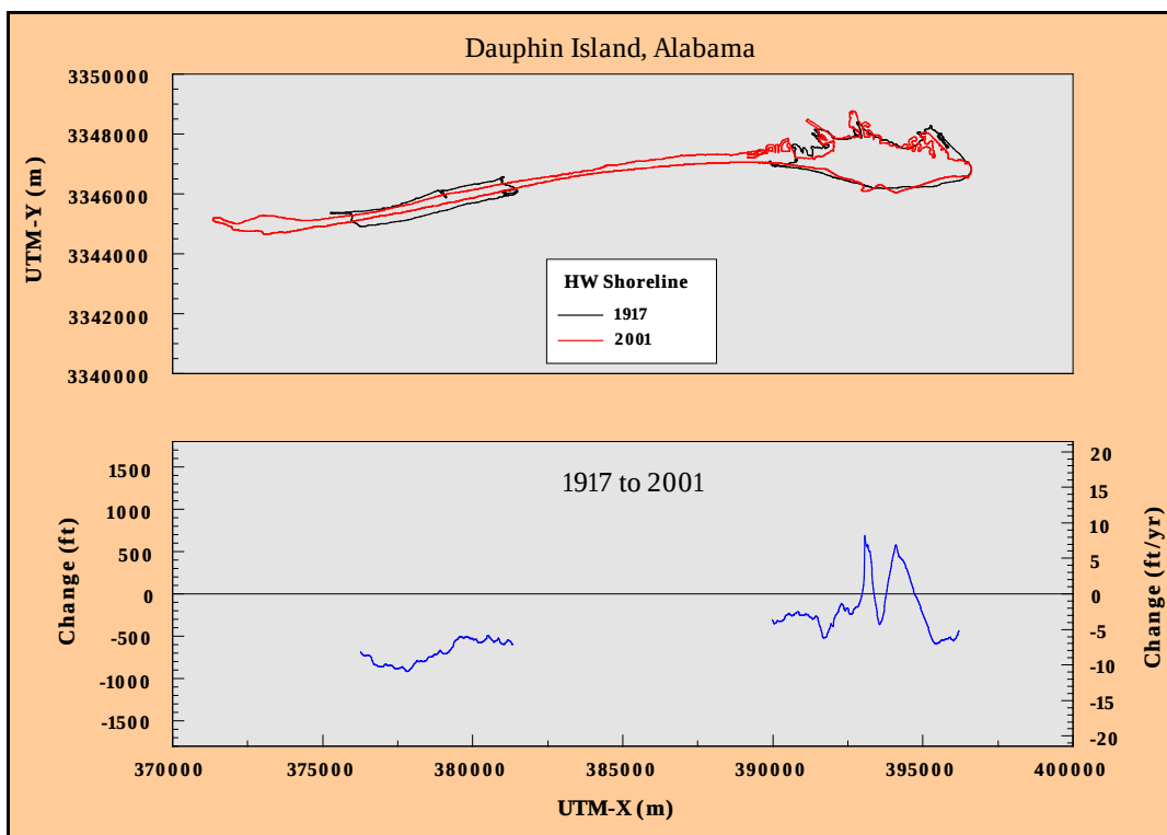
Figure C17. Historical shoreline position change, Dauphin Island, Alabama: 1917 to 2001.
