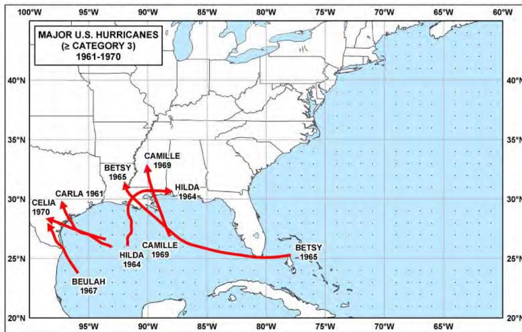
Figure A12. Hurricanes stronger than or equal to category 3 for the Gulf and Atlantic coasts – 1961 to 1970 (Blake et al. 2005).
