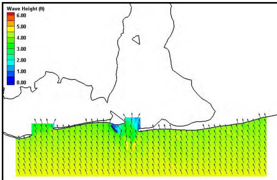
Figure H4. Coarse grid (200m x 200m) wave results for Case 4. Wave heights are shown by color while wave direction is indicated by the arrow direction.
