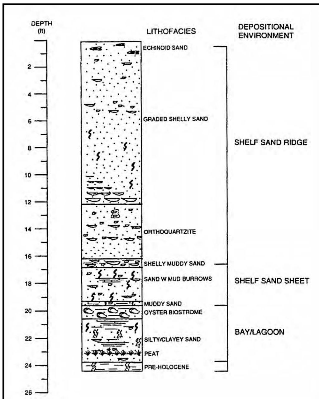
Figure 1-10. Generalized stratigraphic sequence for the Alabama EEZ study area (from Parker et al. 1997).
