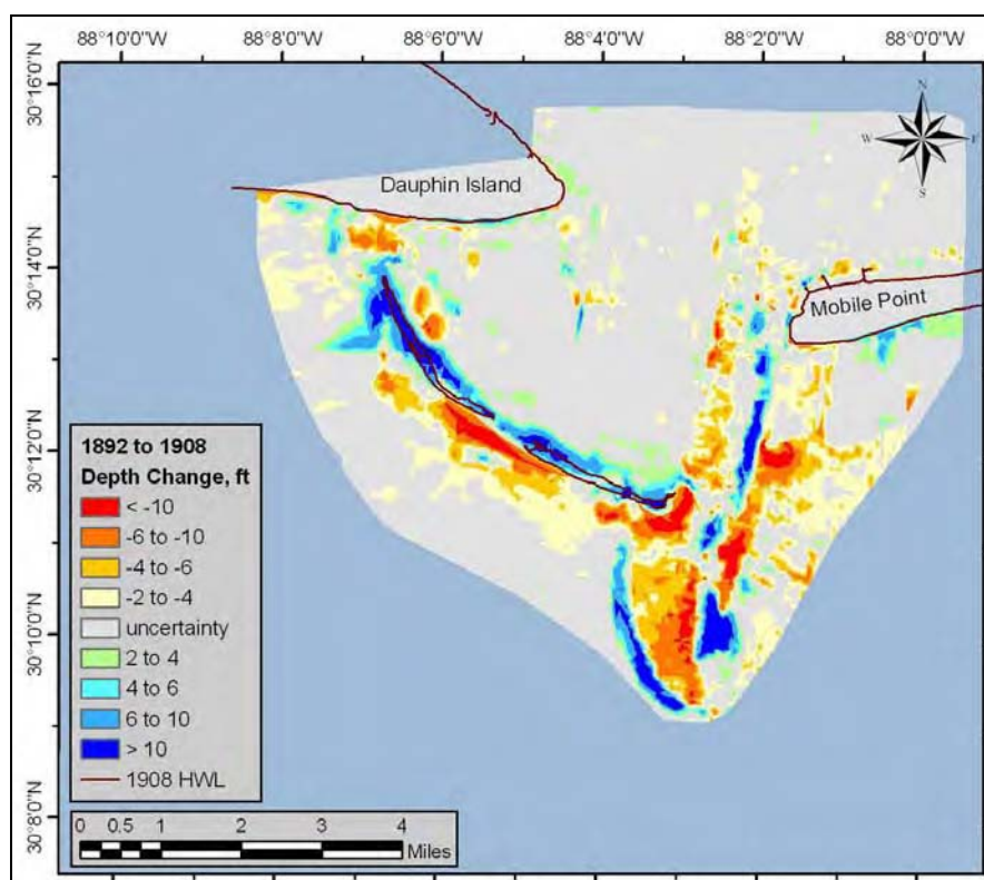
Figure 4-4. Bathymetric changes recorded on the Mobile Pass ebb tidal delta for the period 1892 to 1908.
