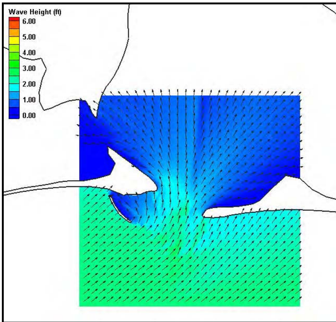
Figure H30. Fine grid (50m x 50m) wave results for Case 10, Mobile Pass. Wave heights are shown by color while wave direction is indicated by the arrow direction.
