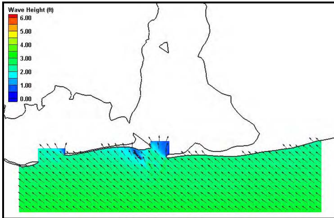
Figure H1. Coarse grid (200m x 200m) wave results for Case 1. Wave heights are shown by color while wave direction is indicated by the arrow direction.
