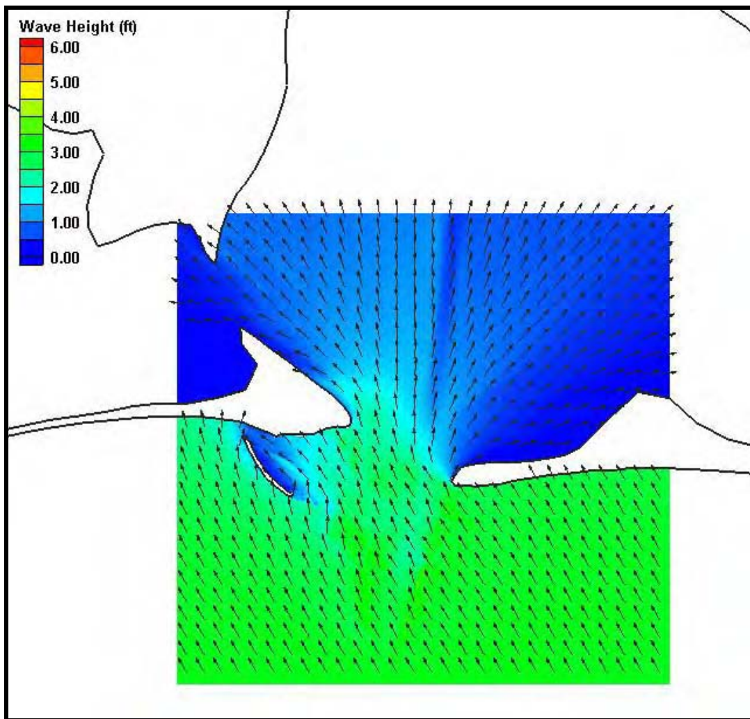
Figure H23. Fine grid (50m x 50m) wave results for Case 3, Mobile Pass. Wave heights are shown by color while wave direction is indicated by the arrow direction.
