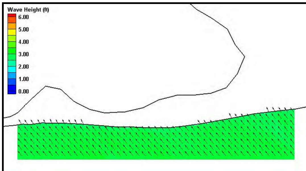
Figure H32. Fine grid (25m x 25m) wave results for Case 2, Morgan Peninsula. Wave heights are shown by color while wave direction is indicated by the arrow direction.
