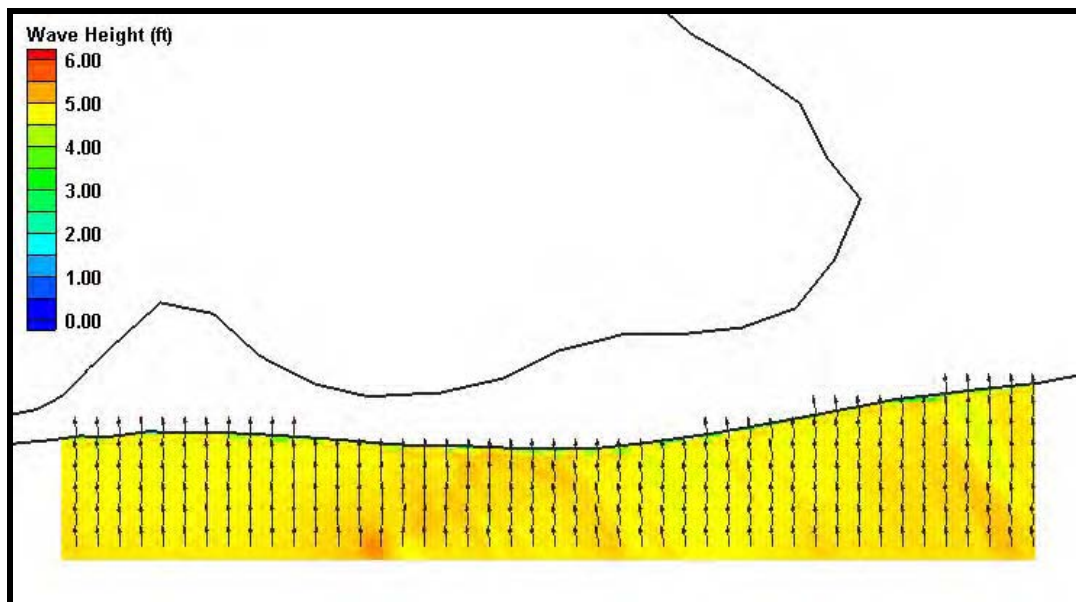
Figure H35. Fine grid (25m x 25m) wave results for Case 5, Morgan Peninsula. Wave heights are shown by color while wave direction is indicated by the arrow direction.
