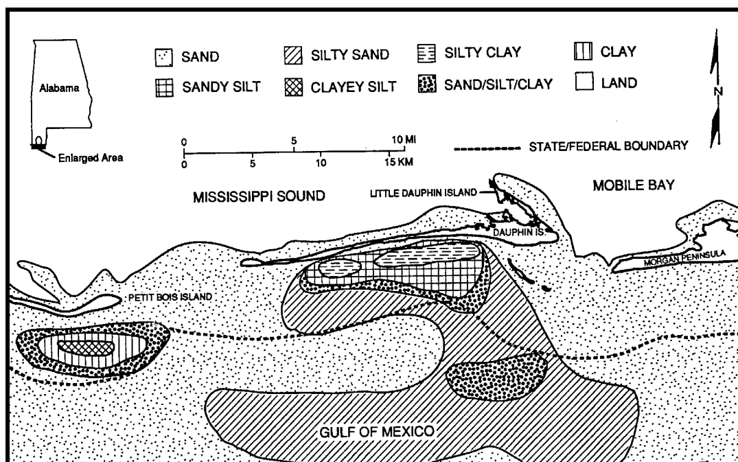
Figure 1-9. Surface sediment distribution in the west Alabama inner continental shelf (from Hummell, 1996).
