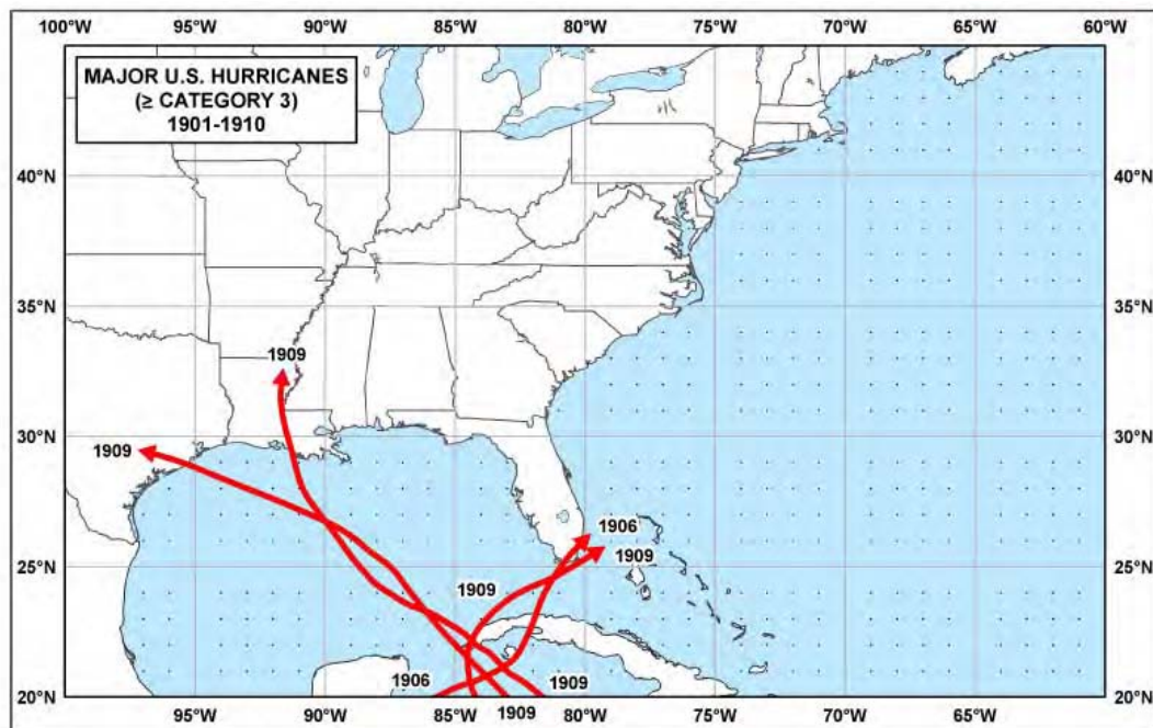
Figure A6. Hurricanes stronger than or equal to category 3 for the Gulf and Atlantic coasts – 1901 to 1910 (Blake et al. 2005).
