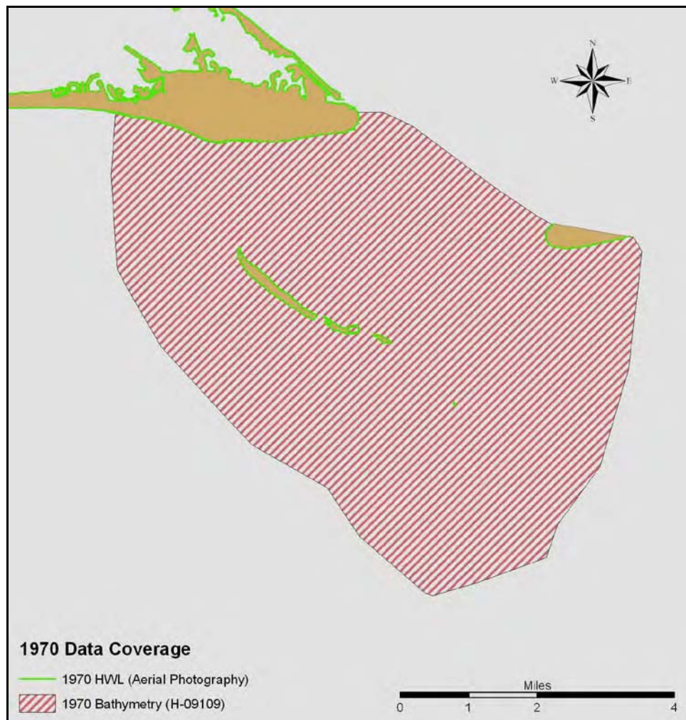
Figure E7. Bathymetry and high-water shoreline data coverage – 1970.
