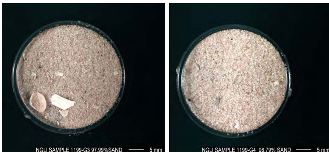
Figure 1-8. Shelf sediment texture east of Mobile Pass (from Sawyer et al. 2001).
