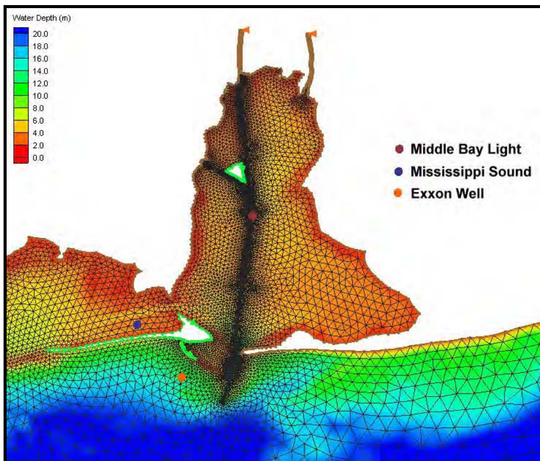
Figure 5-21. Detail of the ADCIRC domain focused on Mobile Bay and Mississippi Sound. Bathymetry contours are shown in color along with the model mesh for this region. Mobile and Tensaw River inflow portions of the mesh can be seen at the north end of Mobile Bay. Three tidal recording stations used to calibrate the model are also shown.
