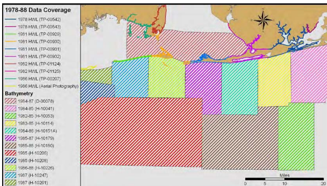
Figure E8. Bathymetry and high-water shoreline data coverage – 1978/88.
