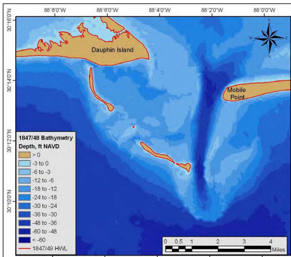
Figure 3-6. Bathymetric surface for Mobile Pass ebb-tidal delta and adjacent shores, 1847/48.
