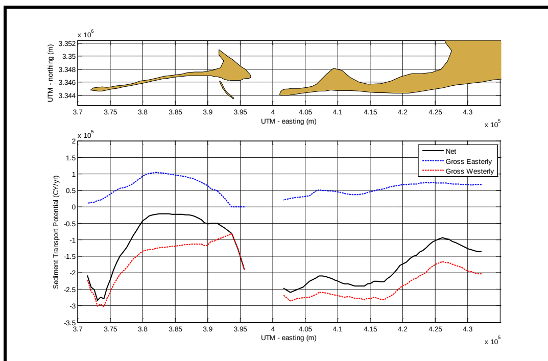
Figure 5-15. Longshore sediment transport potential along Dauphin Island and Morgan Peninsula. Net transport is indicated by a solid black line. Easterly transport is shown as dashed blue, and westerly transport is shown in dashed red.
