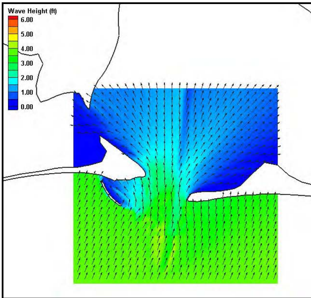
Figure H27. Fine grid (50m x 50m) wave results for Case 7, Mobile Pass. Wave heights are shown by color while wave direction is indicated by the arrow direction.
