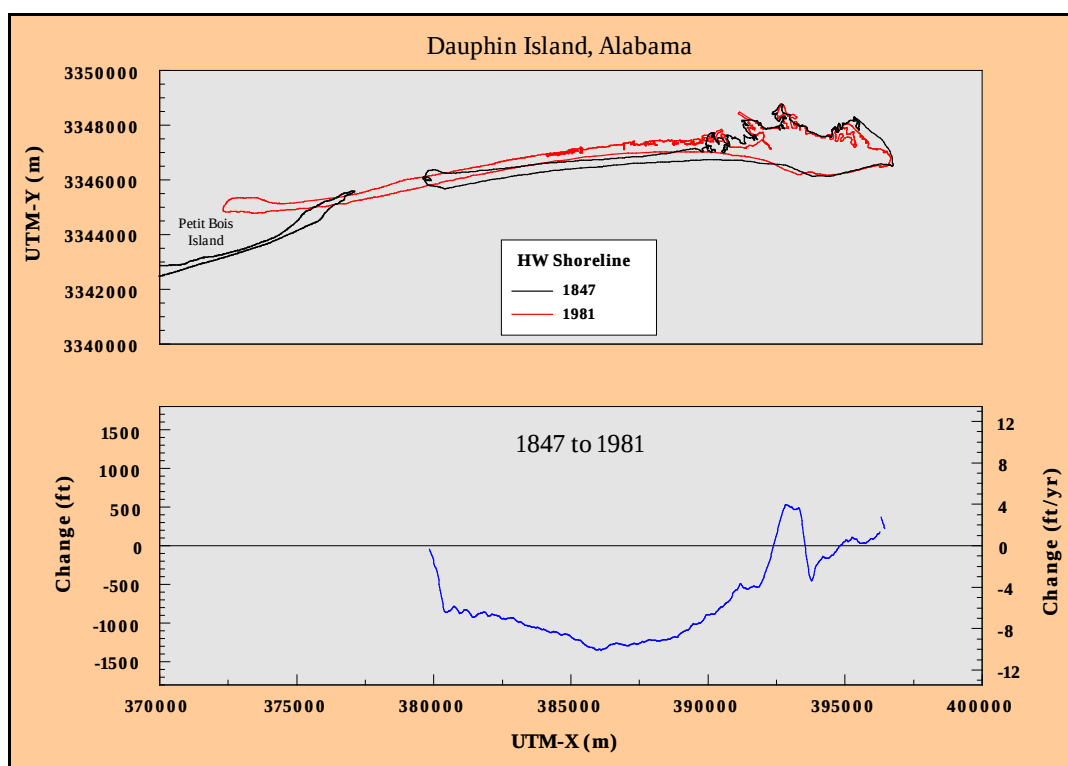
Figure C12. Historical shoreline position change, Dauphin Island, Alabama: 1847 to 1981.
