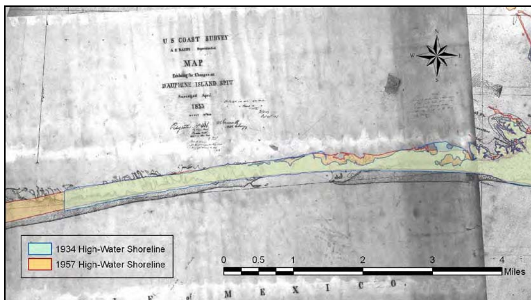
Figure 2-24. Location of the 1934 and 1957 shorelines relative to the 1853 island breach.
