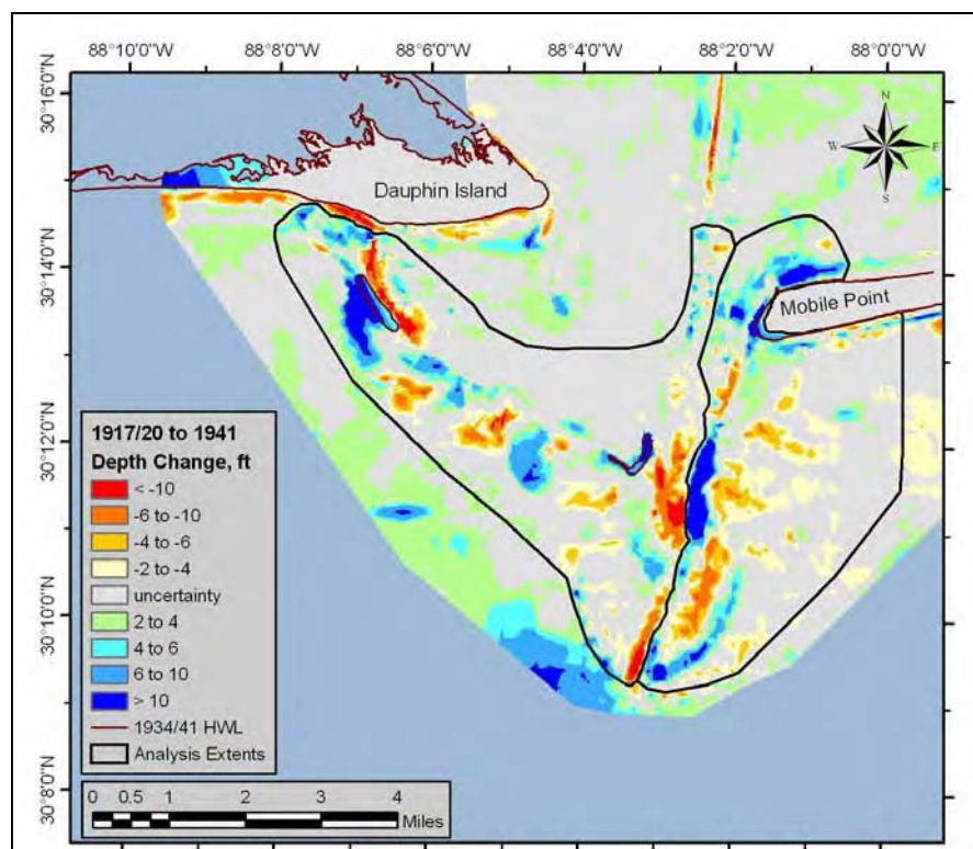
Figure G5. Analysis extent for calculating sand volume change – 1917/20 to 1941.
