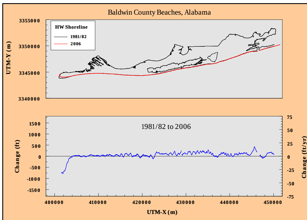
Figure D10. Historical shoreline position change, Perdido Pass to Mobile Point, Alabama: 1981/82 to 2006.
