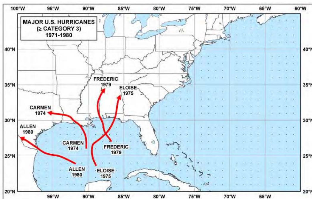
Figure A13. Hurricanes stronger than or equal to category 3 for the Gulf and Atlantic coasts – 1971 to 1980 (Blake et al. 2005).
