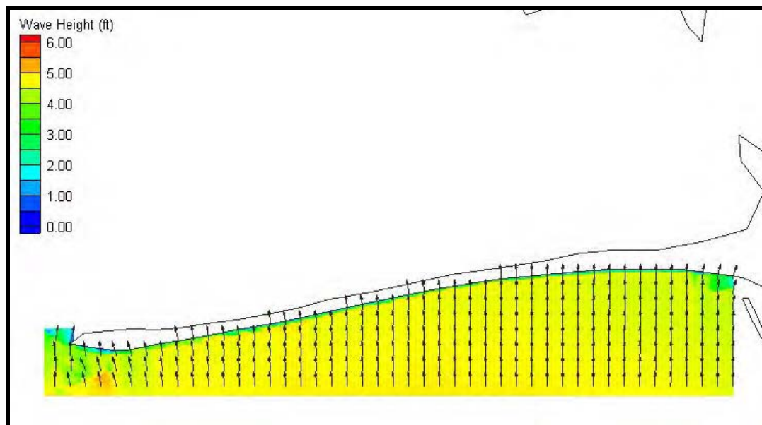
Figure 5-9. Fine grid (25 m x 25 m) wave results for Case 5, Dauphin Island. Wave heights are shown by color while wave direction is indicated by arrow direction.
