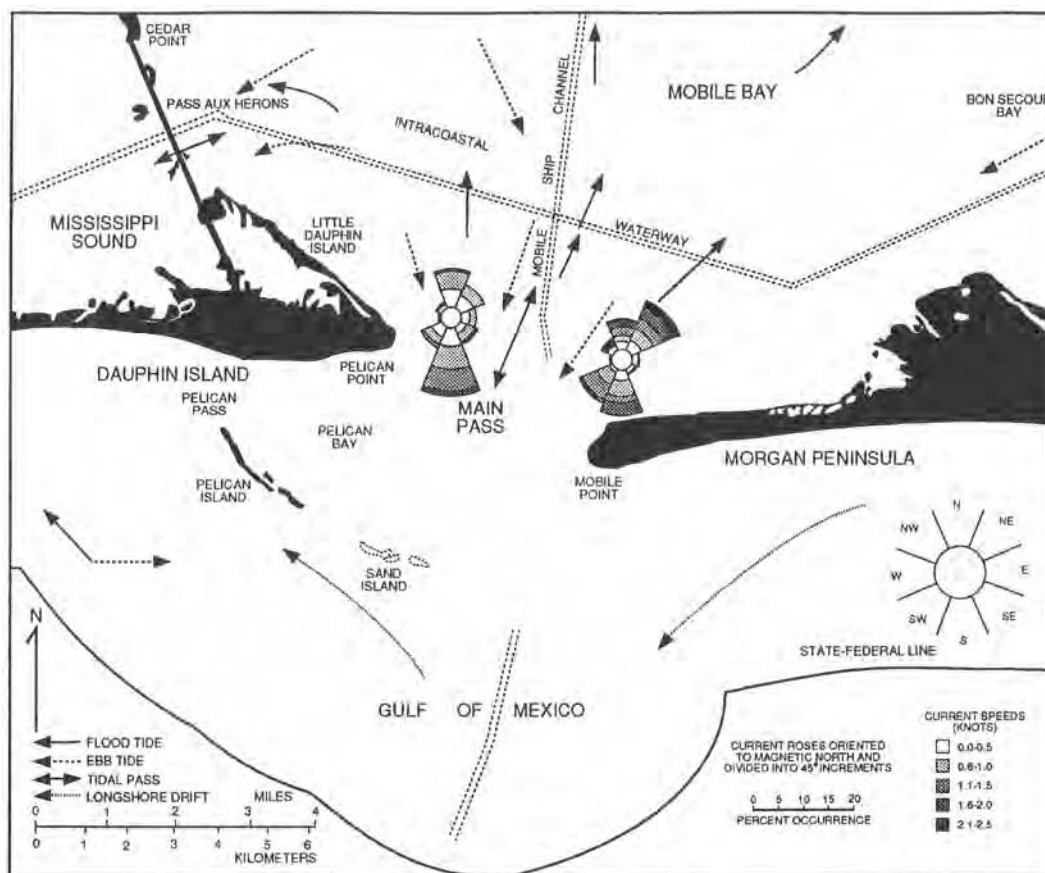
Figure 1-11. Average surface current during flood and ebb tide near Main Pass (from Hummell, 1990).
