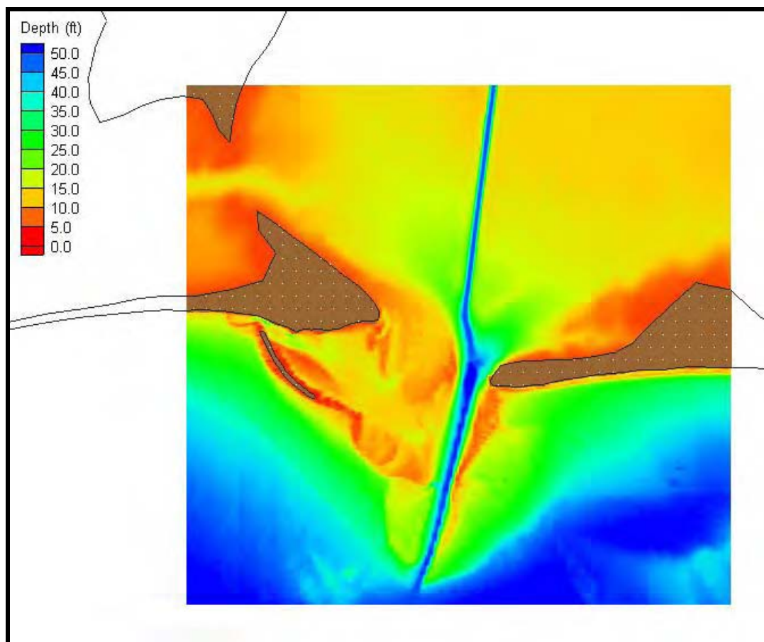
Figure 5-27. CMS-M2D model domain and bathymetry.
