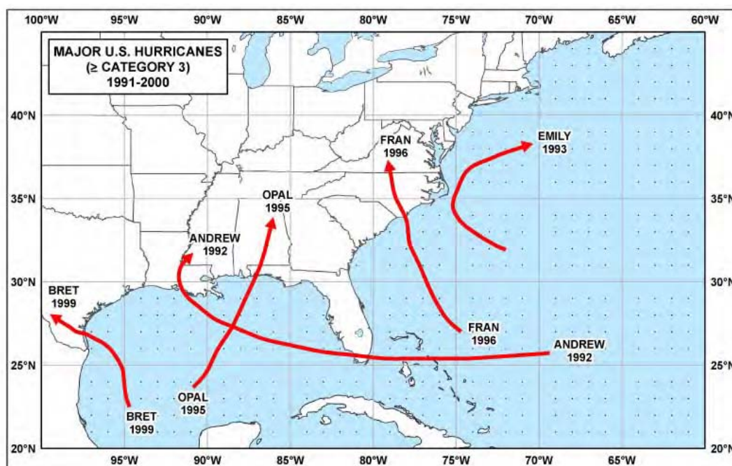
Figure A15. Hurricanes stronger than or equal to category 3 for the Gulf and Atlantic coasts – 1991 to 2000 (Blake et al. 2005).
