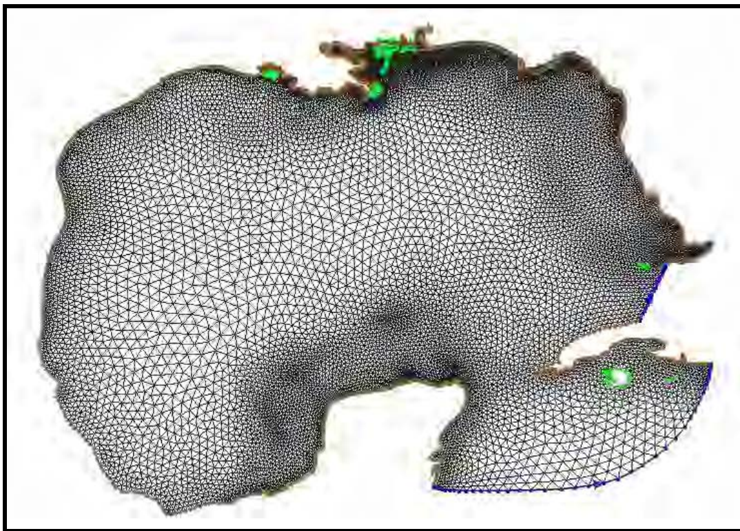
Figure 5-20. ADCIRC model domain for the Gulf of Mexico. The two open boundaries are shown in navy blue, land boundaries are in brown, and islands are in green.
