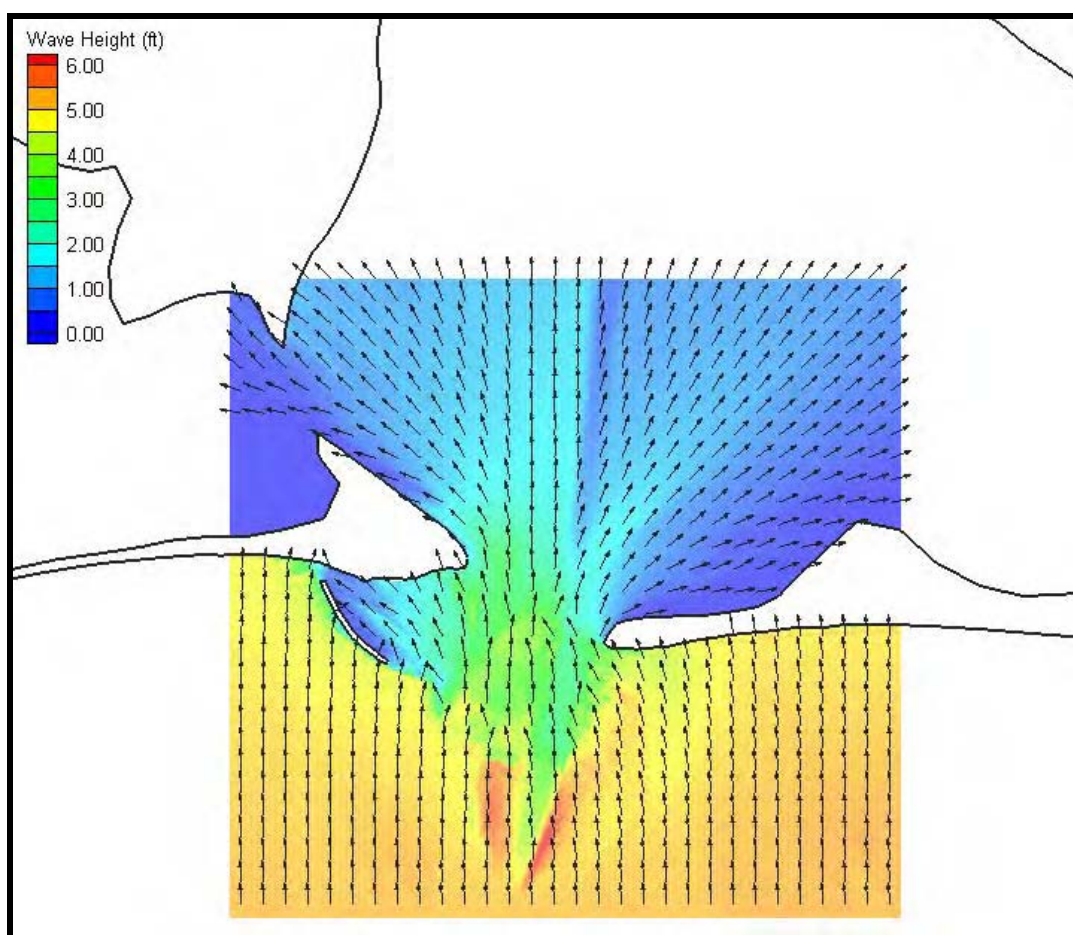
Figure 5-11. Fine grid (50 m x 50 m) wave results for Case 5, Mobile Pass. Wave heights are shown by color while wave direction is indicated by the arrow direction.
