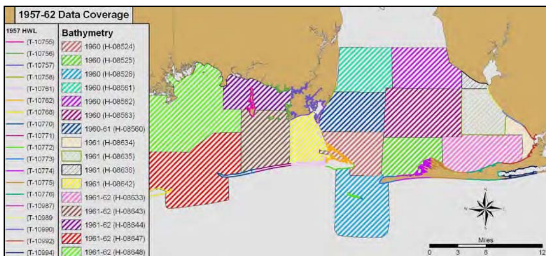
Figure E6. Bathymetry and high-water shoreline data coverage – 1957/62.
