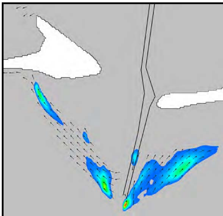
Figure 5-34. CMS-M2D average transport vectors for Case 3 during ebb tide.
