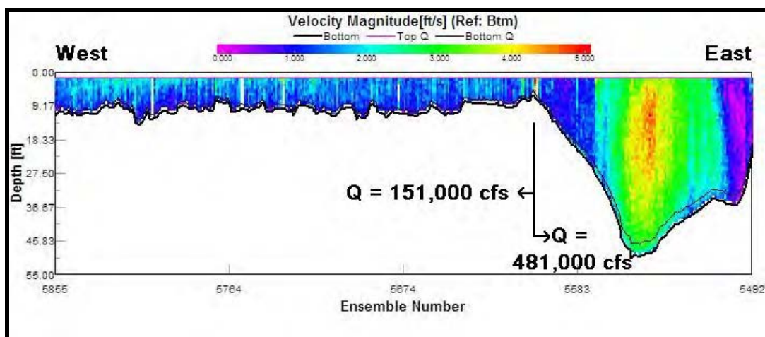
Figure 5-18. Color contour plot of velocities in Mobile Pass during maximum flood tide conditions.
