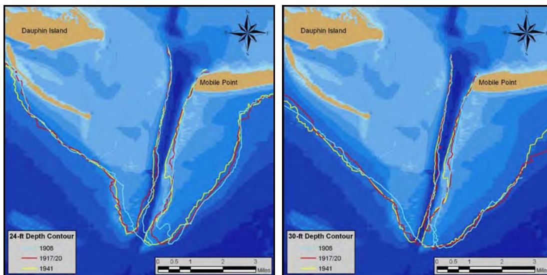
Figure 3-16. Variations in location of the 24- and 30-ft depth contours, 1908, 1917/20, and 1941.
