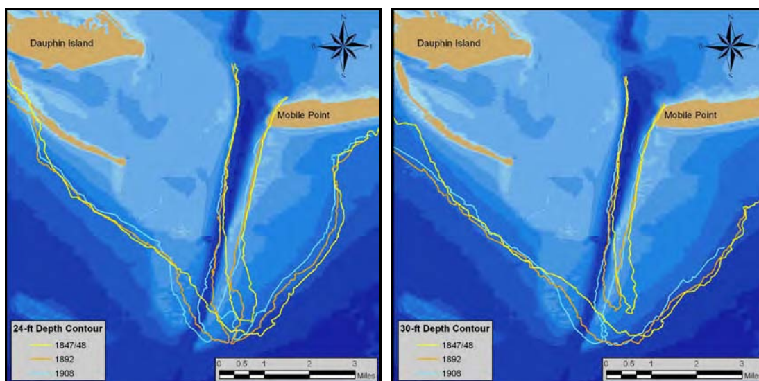
Figure 3-15. Variations in location of the 24- and 30-ft depth contours, 1847/48, 1892, and 1908.
