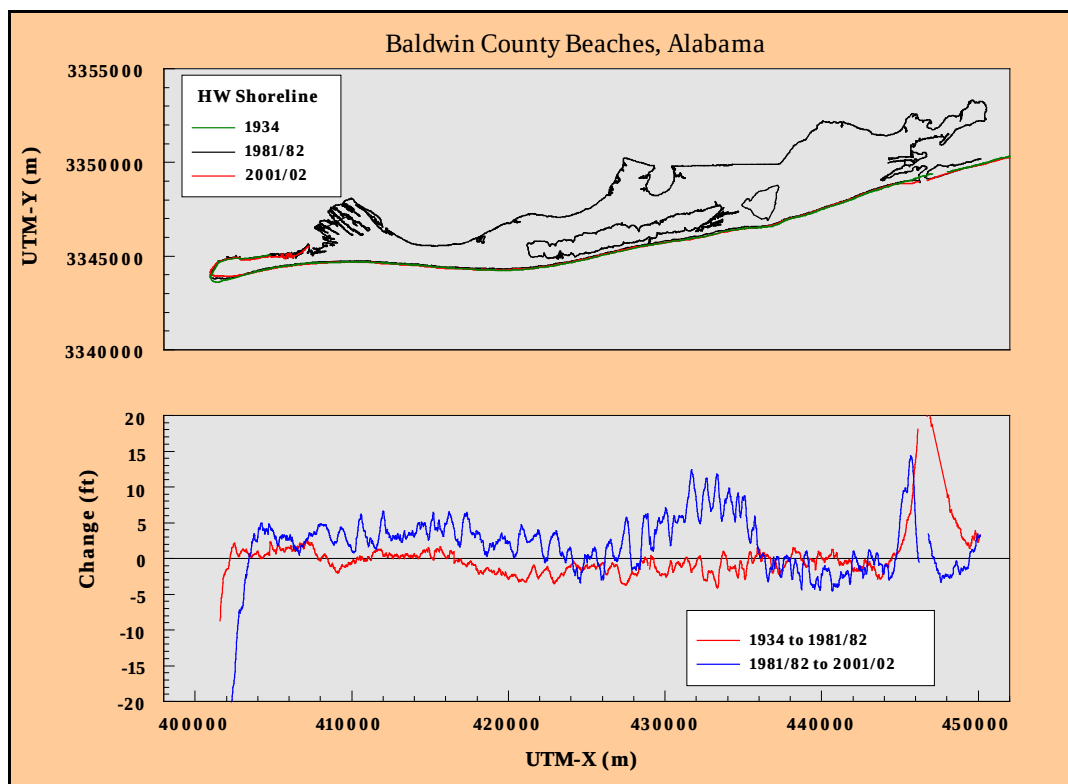
Figure 2-33. Shoreline change between 1934 and 2001/02 illustrating sand accumulation at the jetties at Perdido Pass and net shoreline advance west of this point until Mobile Point, Alabama.
