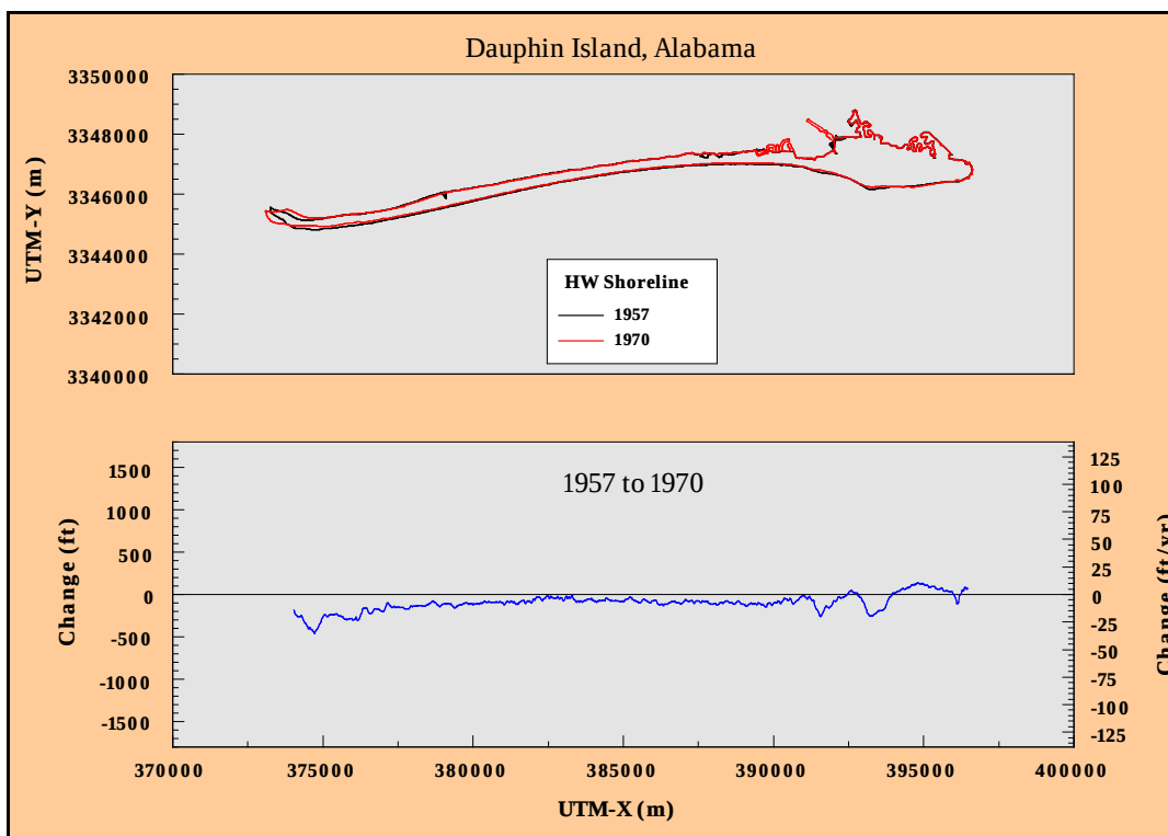
Figure C7. Historical shoreline position change, Dauphin Island, Alabama: 1957 to 1970.
