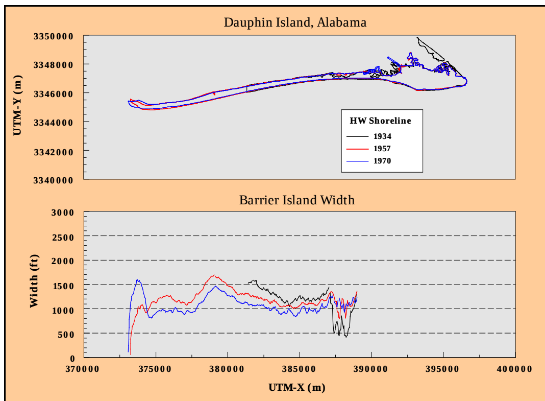
Figure 2-18. Changes in barrier island width between 1934 and 1970, Dauphin Island, AL.
