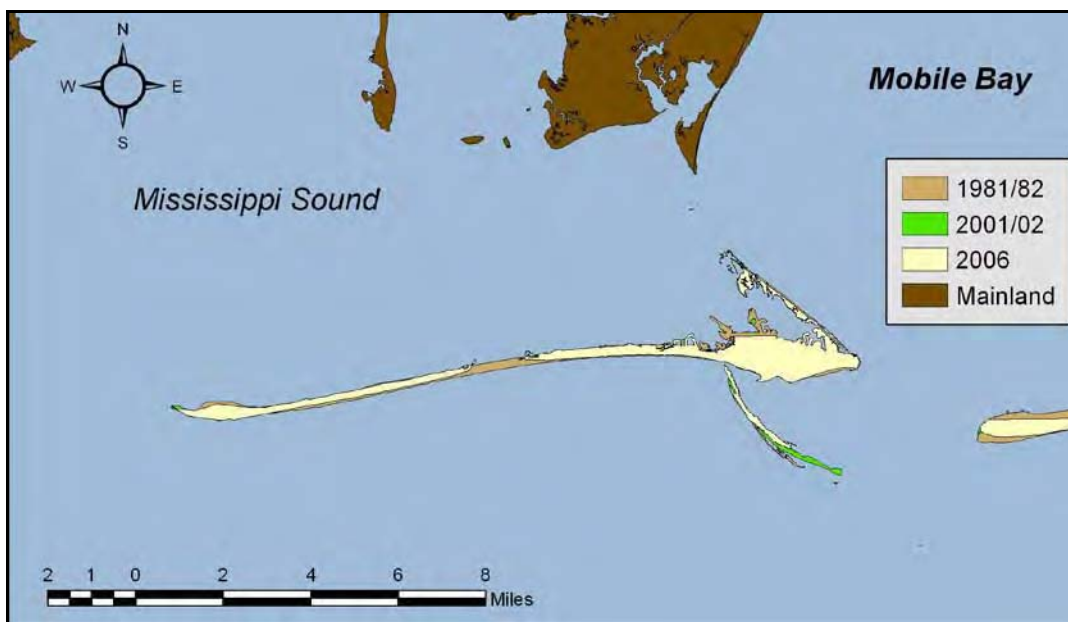
Figure 2-14. 2006 shoreline superimposed on 1981/82 and 2001/02 shorelines illustrating island growth on the ebb-tidal delta to the northwest and breaching on Dauphin Island after Hurricanes Ivan (2004) and Katrina (2005).
