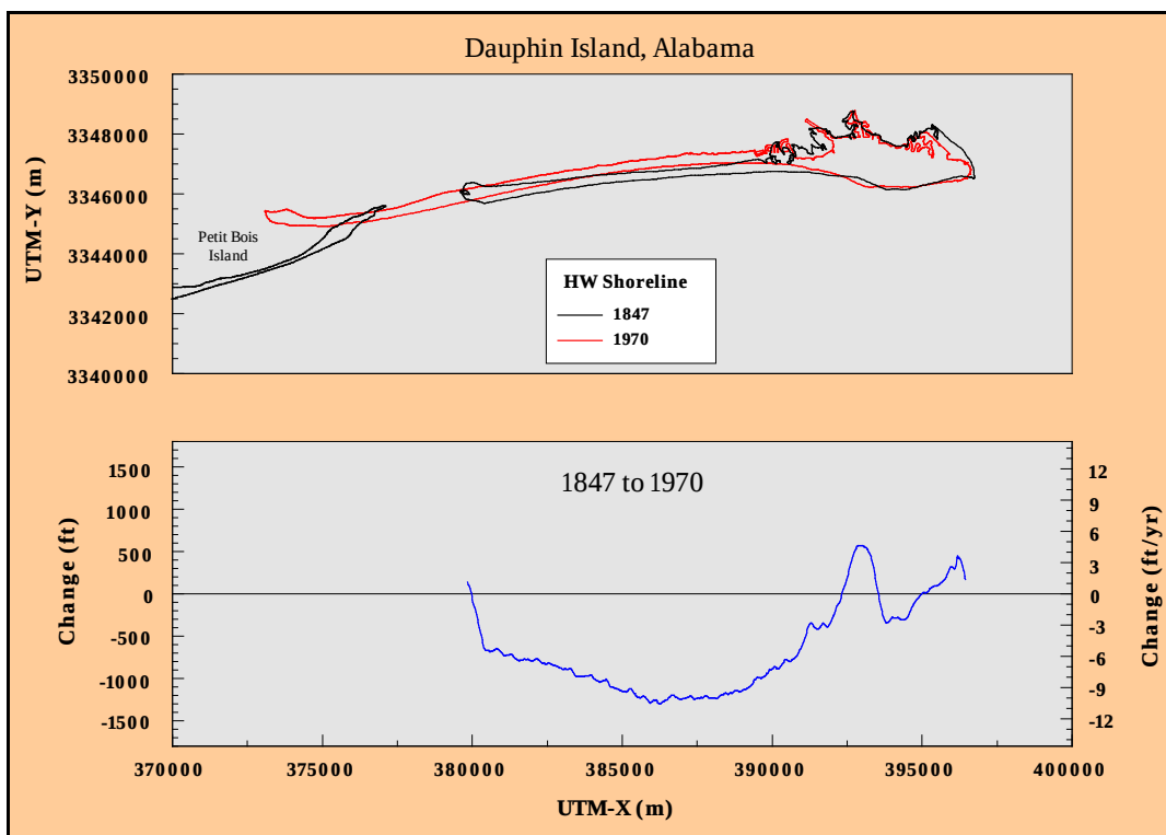
Figure C9. Historical shoreline position change, Dauphin Island, Alabama: 1847 to 1970.
