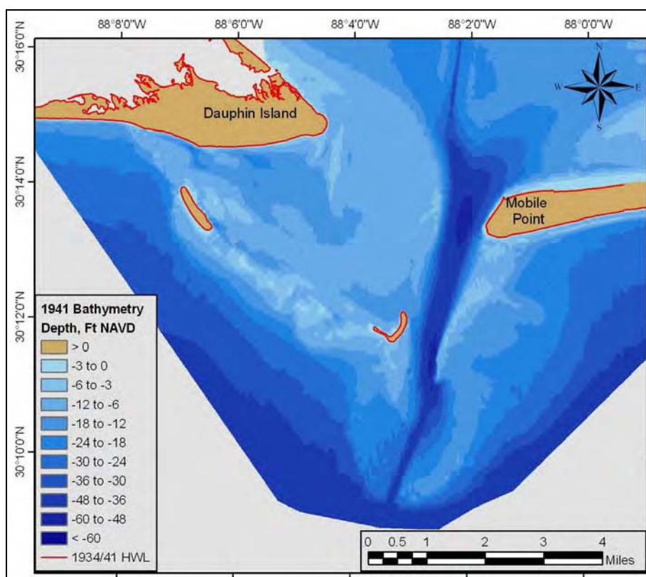
Figure 3-10. Bathymetric surface for Mobile Pass ebb-tidal delta and adjacent shores, 1941.
