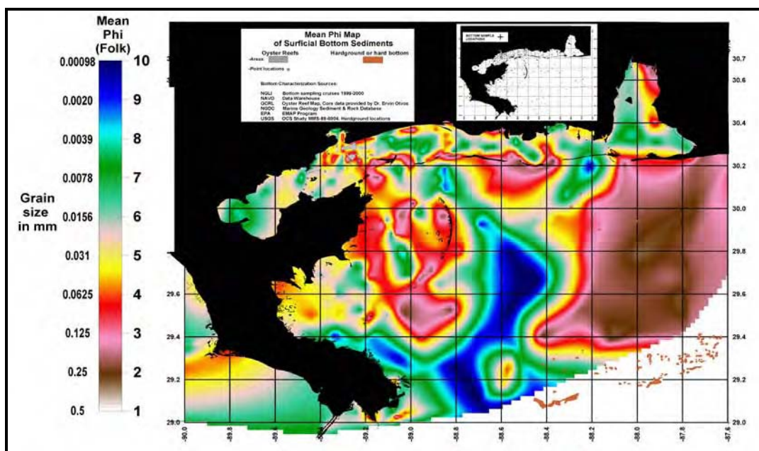
Figure 1-7. Map of sediment mean grain size in the Mississippi Bight (from Sawyer et al. 2001).
