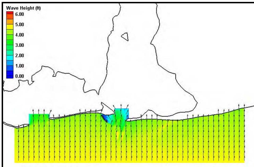
Figure H6. Coarse grid (200m x 200m) wave results for Case 6. Wave heights are shown by color while wave direction is indicated by the arrow direction.
