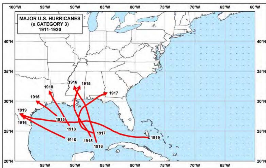
Figure A7. Hurricanes stronger than or equal to category 3 for the Gulf and Atlantic coasts – 1911 to 1920 (Blake et al. 2005).
