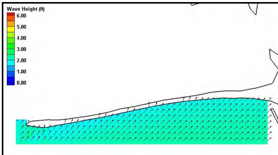
Figure H20. Fine grid (25m x 25m) wave results for Case 10, Dauphin Island. Wave heights are shown by color while wave direction is indicated by the arrow direction.
