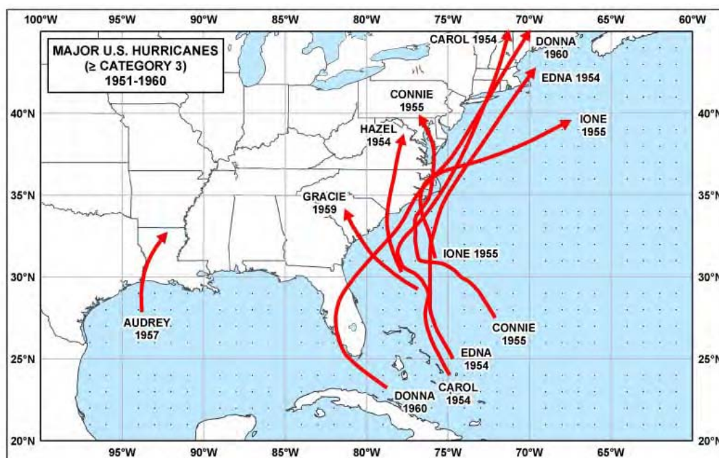
Figure A11. Hurricanes stronger than or equal to category 3 for the Gulf and Atlantic coasts – 1951 to 1960 (Blake et al. 2005).
