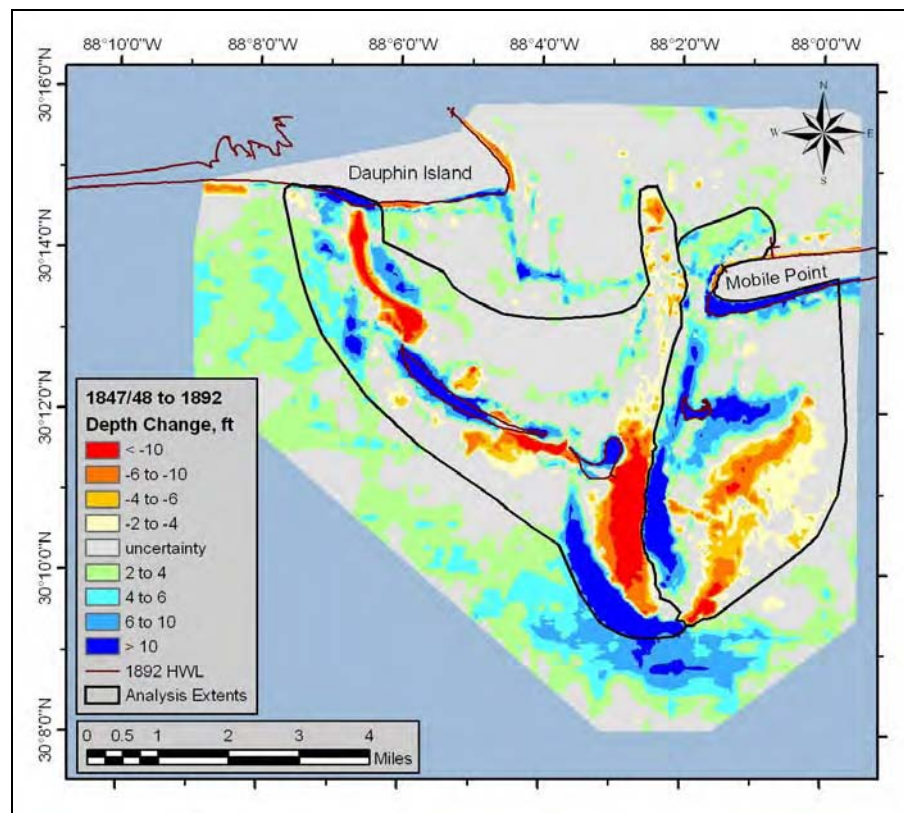
Figure G1. Analysis extent for calculating sand volume change - 1847/48 to 1892.
