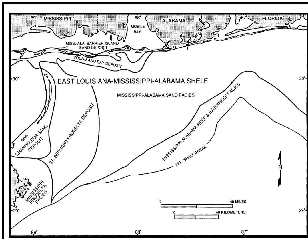
Figure 1-4. Sedimentary facies on the east Louisiana-Mississippi-Alabama shelf (after Ludwick, 1964; from Parker et al. 1997).
