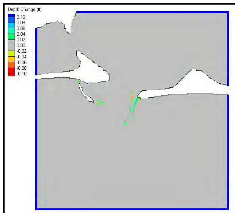
Figure 5-28. Bottom change results for 3 days of average tidal conditions only. Erosion is in yellow/red and accretion is in blue/green.
