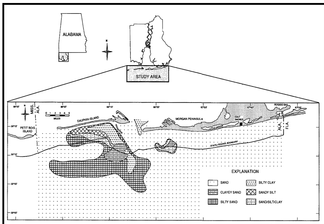
Figure 1-5. Surface sediment texture map (from USACE, 1984).
