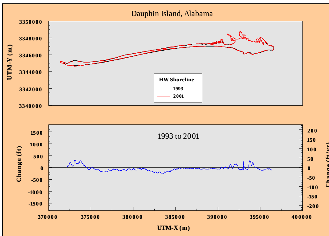
Figure C16. Historical shoreline position change, Dauphin Island, Alabama: 1993 to 2001.
