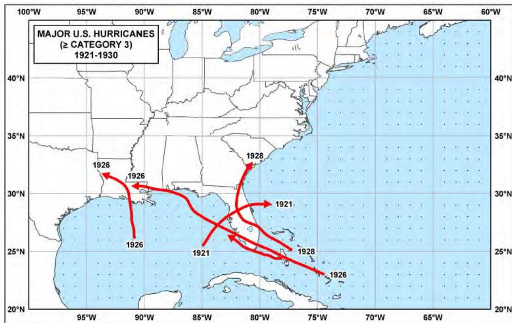
Figure A8. Hurricanes stronger than or equal to category 3 for the Gulf and Atlantic coasts – 1921 to 1930 (Blake et al. 2005).
