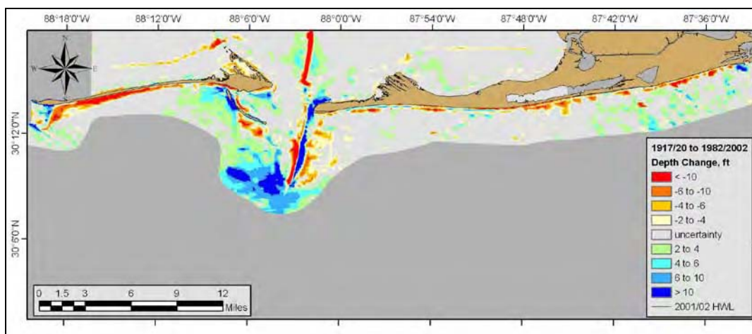
Figure 4-2. Bathymetric change between 1917/20 and 1982/2002 for the Alabama coastal zone. Hot colors represent erosion (yellow to red), and cool colors represent deposition (green to blue).
