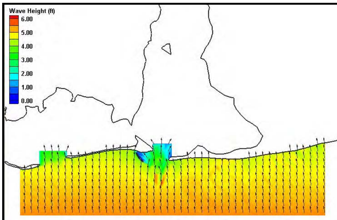
Figure H5. Coarse grid (200m x 200m) wave results for Case 5. Wave heights are shown by color while wave direction is indicated by the arrow direction.
