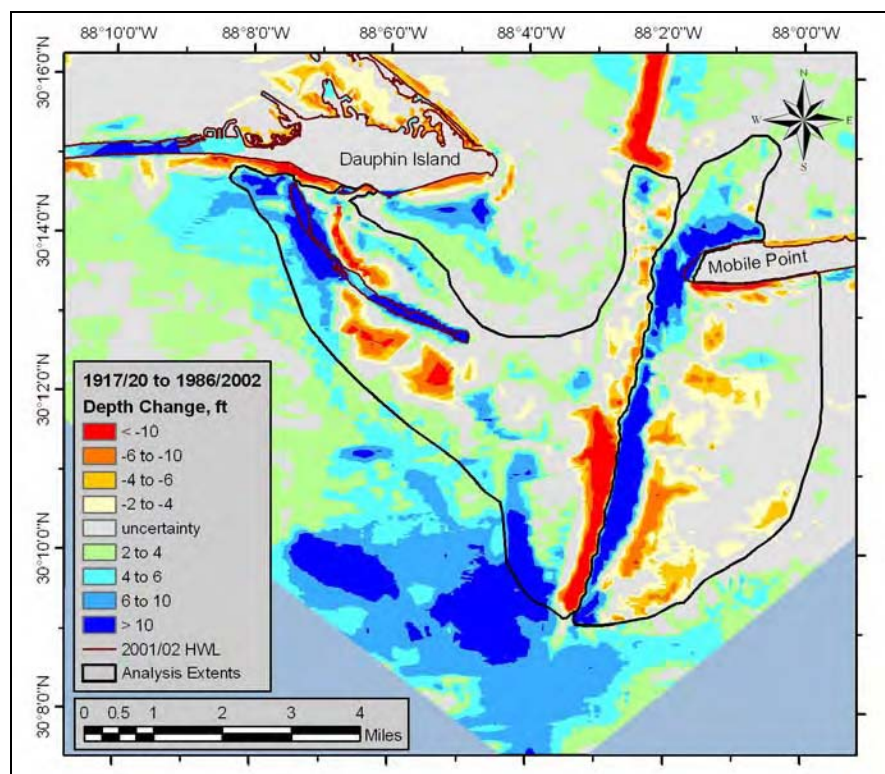
Figure G8. Analysis extent for calculating sand volume change – 1917/20 to 2002.
