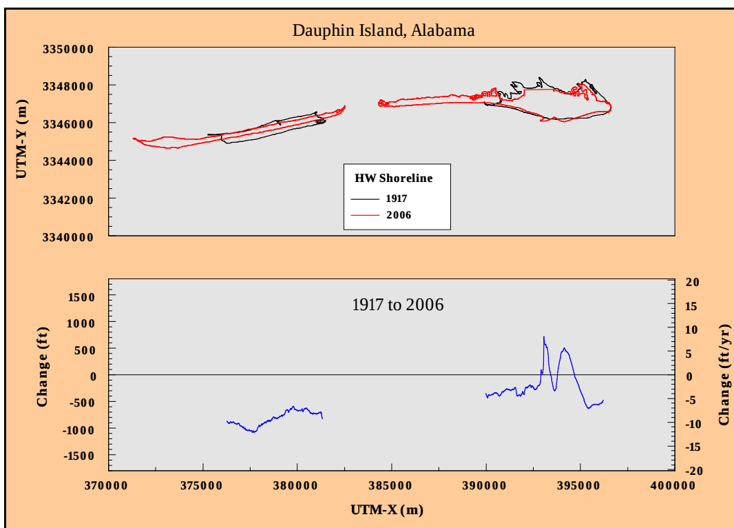
Figure C20. Historical shoreline position change, Dauphin Island, Alabama: 1917 to 2006.
