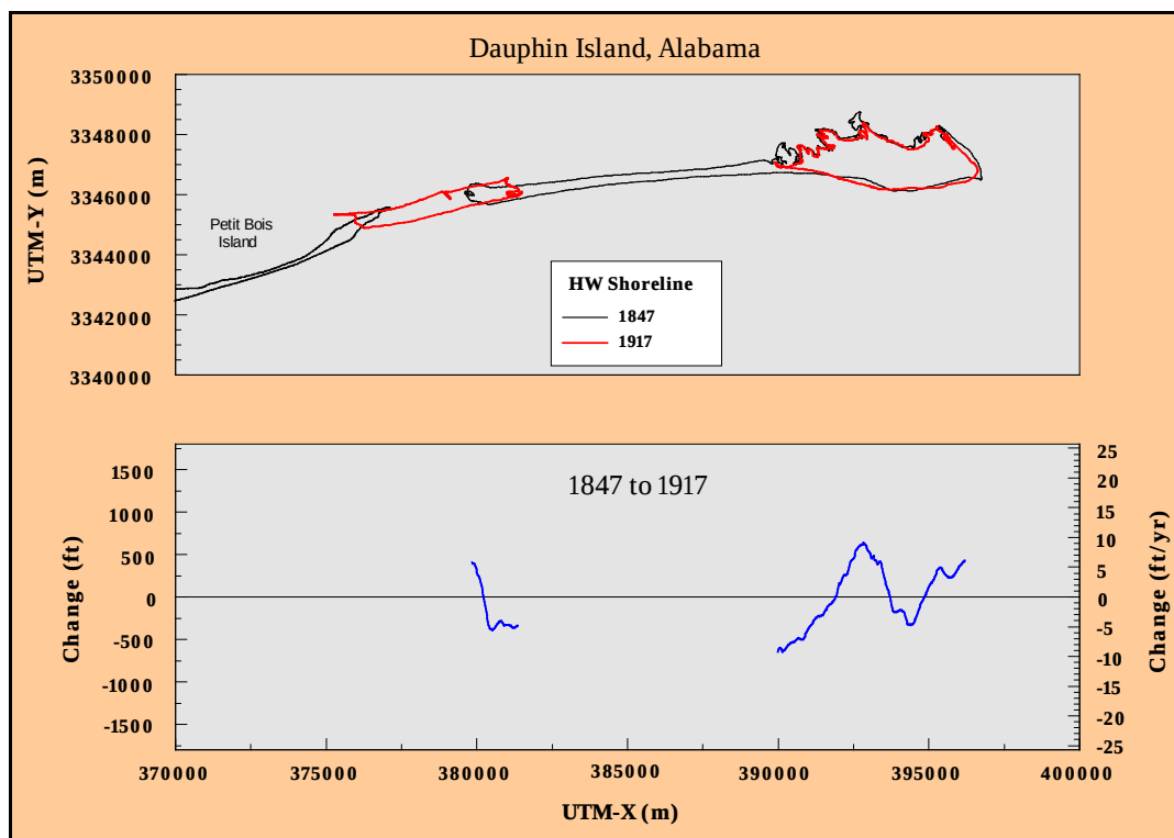
Figure C1. Historical shoreline position change, Dauphin Island, Alabama: 1847 to 1917.
