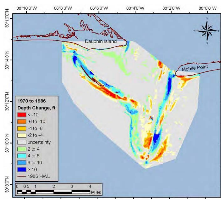
Figure 4-9. Bathymetric changes on the Mobile ebb-tidal delta, 1970 to 1986.
