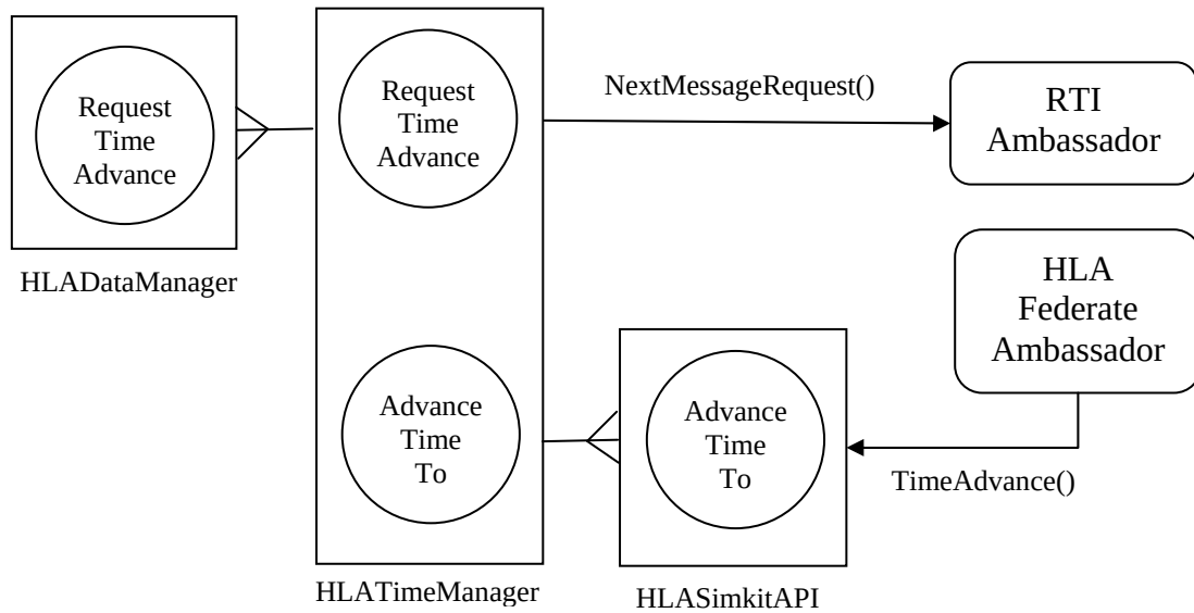
Figure 28. Time management interface through HLA event listening
