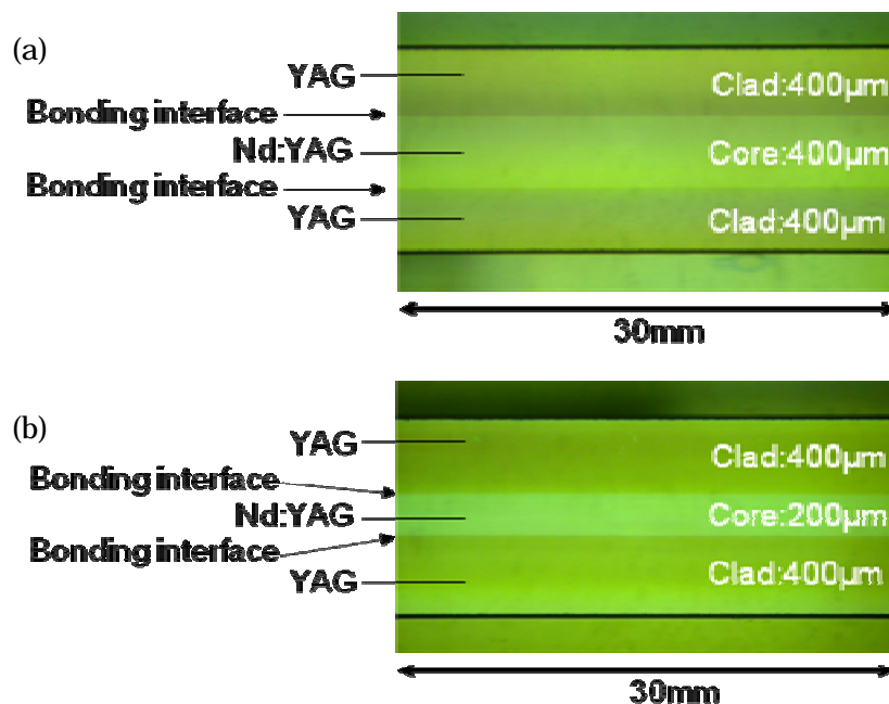
Fig.10 Cross-section of waveguide laser elements under a stereoscopic microscope (a) Sample with core thickness of 400 \mu\text{m} layer. (b) Sample with core thickness of 200 \mu\text{m} layer.
