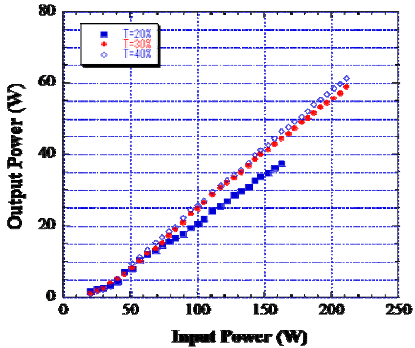
Fig.21 Laser performance at different transmittance of output coupler
