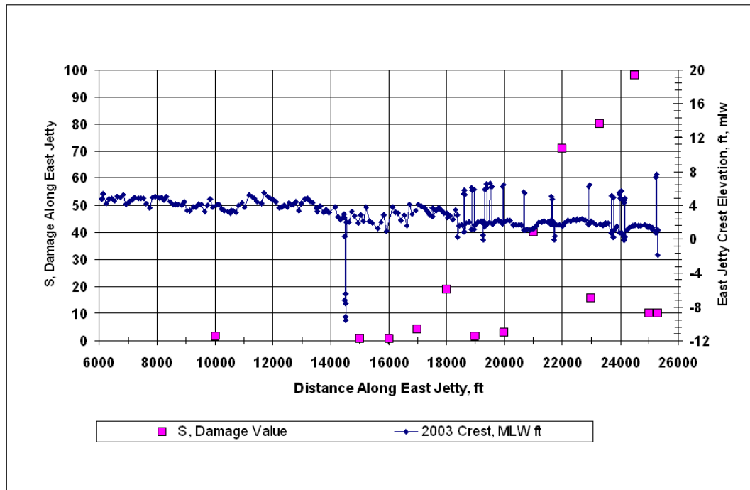
Figure 45. East jetty fifty-year damage values (2010-2060) along jetty for Sabine Pass wave climate and existing structure, plotted with 2003 jetty crest elevations.
