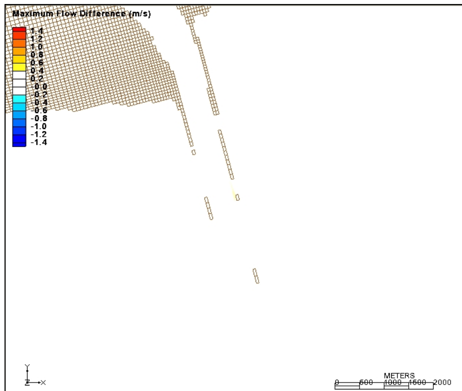
Figure 73. Difference in maximum flow magnitude between Plan 1 and existing conditions for the low-energy wave simulation in 2060.
