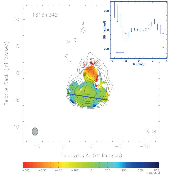
Figure 1. Rotation Measure image of J1613+342 in false color with a slice perpendicular to the jet axis inset. The zero point on the inset slice corresponds to the center of the jet, and the bar denotes the angular resolution. Image coordinates are only relative since no phase referencing was performed. The synthesized beam (shown in lower left) has dimensions 1.6 \times 1.2 mas in position angle 0^\circ . Contours are drawn from the 8 GHz total intensity image logarithmically at factor of two intervals with the first contour at 2 \text{ mJy beam}^{-1} . The Spearman correlation coefficient is -0.2 , and the reduced \chi^2 for a linear fit of the RM with position is 2.8.
