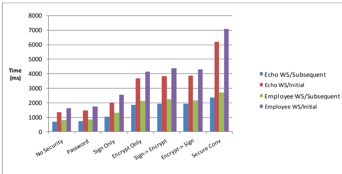
Figure 4: Startup Times per Mechanism/Service, Initial versus Subsequent Communications
