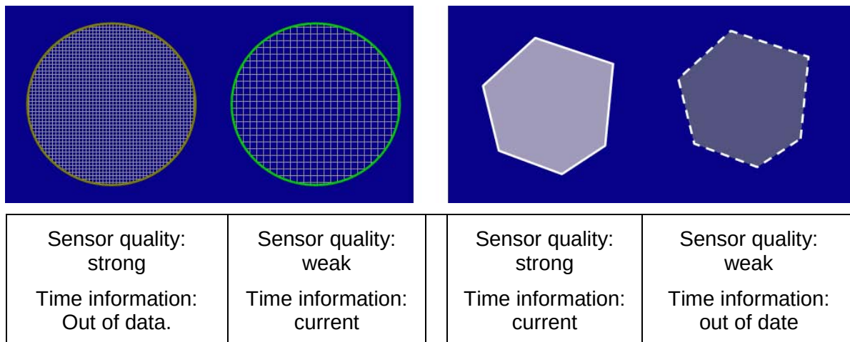
Figure 2: Sample of design concepts for sensor uncertainty, phase one. Sensor quality: Good quality was represented by either light grey or a fine hash; poor quality by a dark grey or coarse hash. Sensor time lateness was indicated by either the type of the swath border (current=solid/out of date=broken) or the border color (current=green/out of date=gold).
