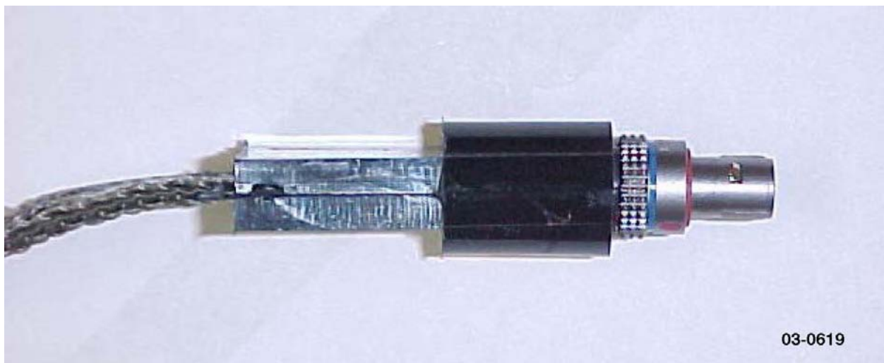
Figure 111. Prototype 5-pin lemo thermoset overmold (side view)
