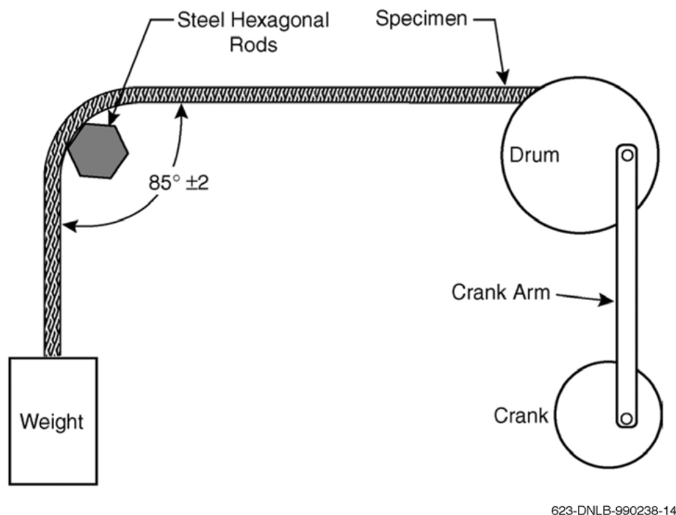
Figure 26. Abrasion over hex bar
