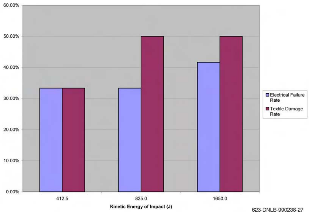
Figure 63. Effect of impact energy on cable failure rate
