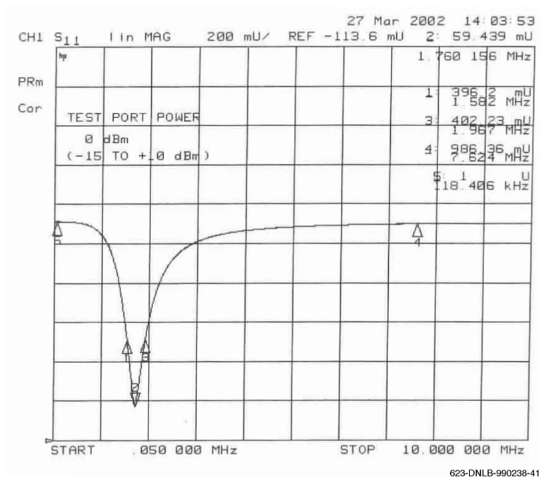
Figure 105. Reflection coefficient for 22 AWG silver coated copper wire air core transformer
