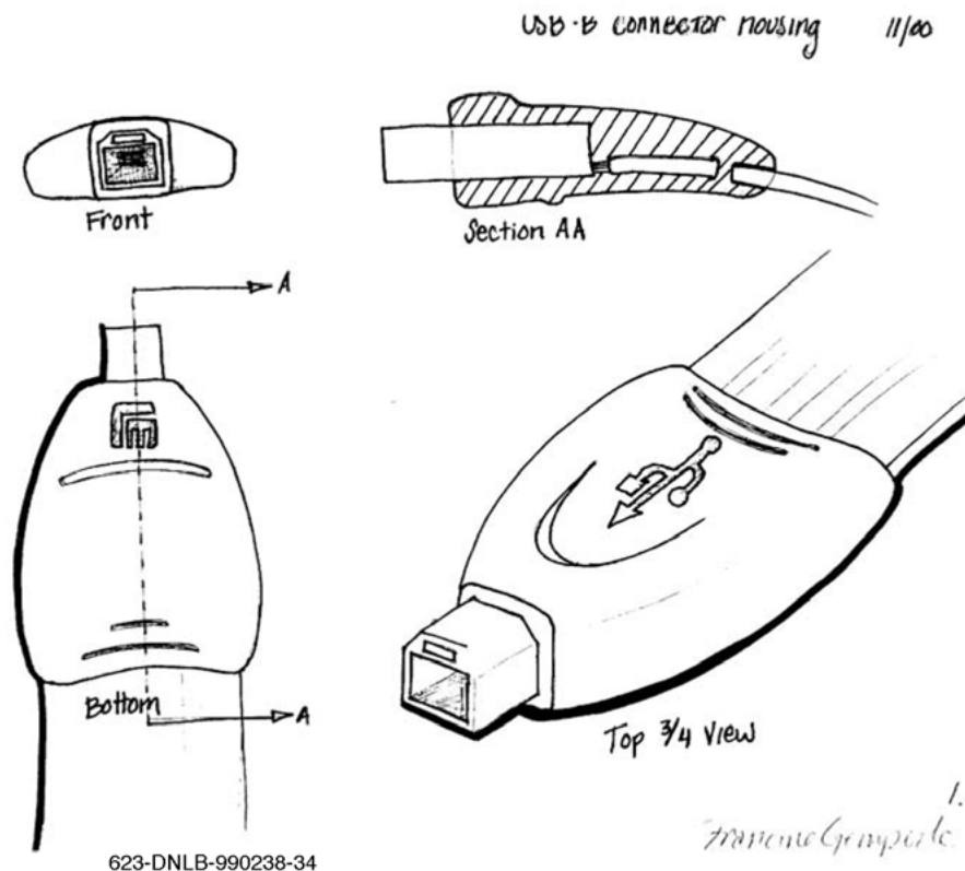
Figure 76. Preferred embodiment of USB Type B connector
