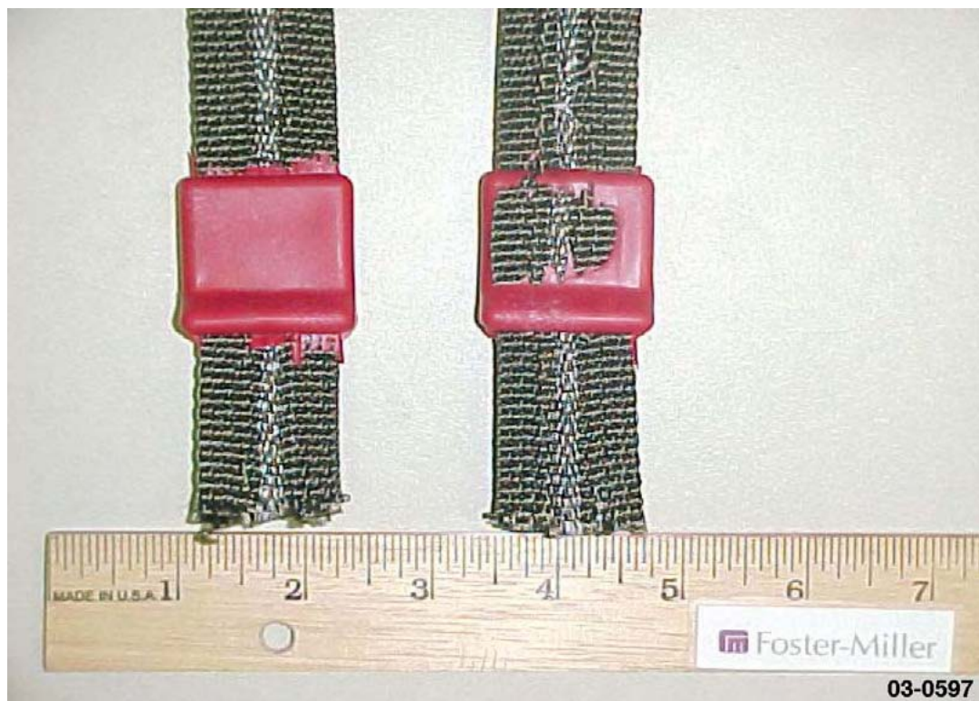
Figure 78. Sarlink test connector
