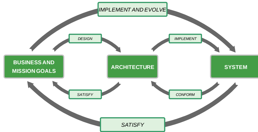
Figure 1: Architecture-Centric Engineering
