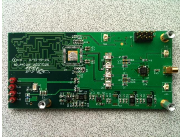
Figure 2 Waveform synthesizer with up-conversion for radar waveform generation.
