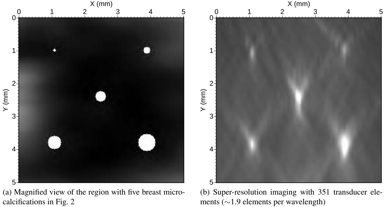
Figure 3: Magnified view of the region with embedded microcalcifications in Fig. 2 and the corresponding super-resolution imaging result obtained using a linear ultrasound array with 351 elements. All five microcalcifications can be clearly identified.
