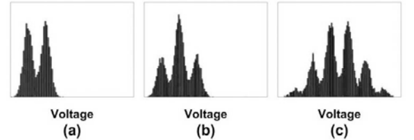
Fig. 12. Amplitude distribution function of the diffusion noise with 2, 3 and 6 particles in the presence of background noise.
