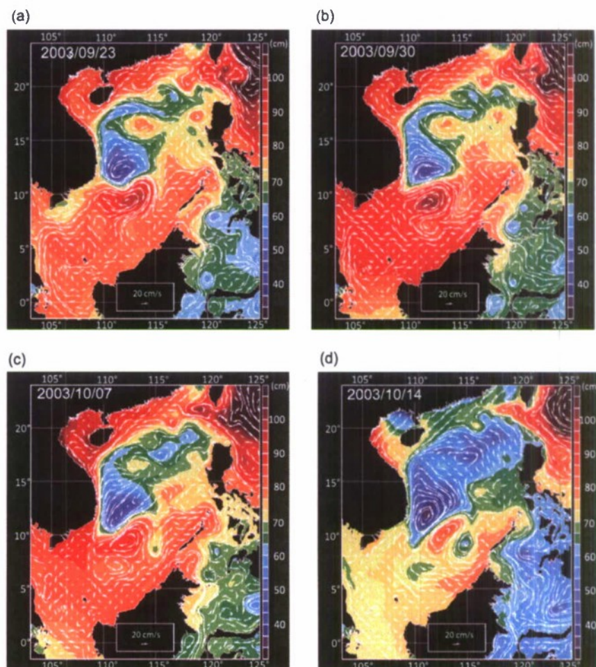
Figure 14. Same as Figure 12 except for (a) 23 September, (b) 30 September, (c) 7 October, and (d) 14 October in 2003.
