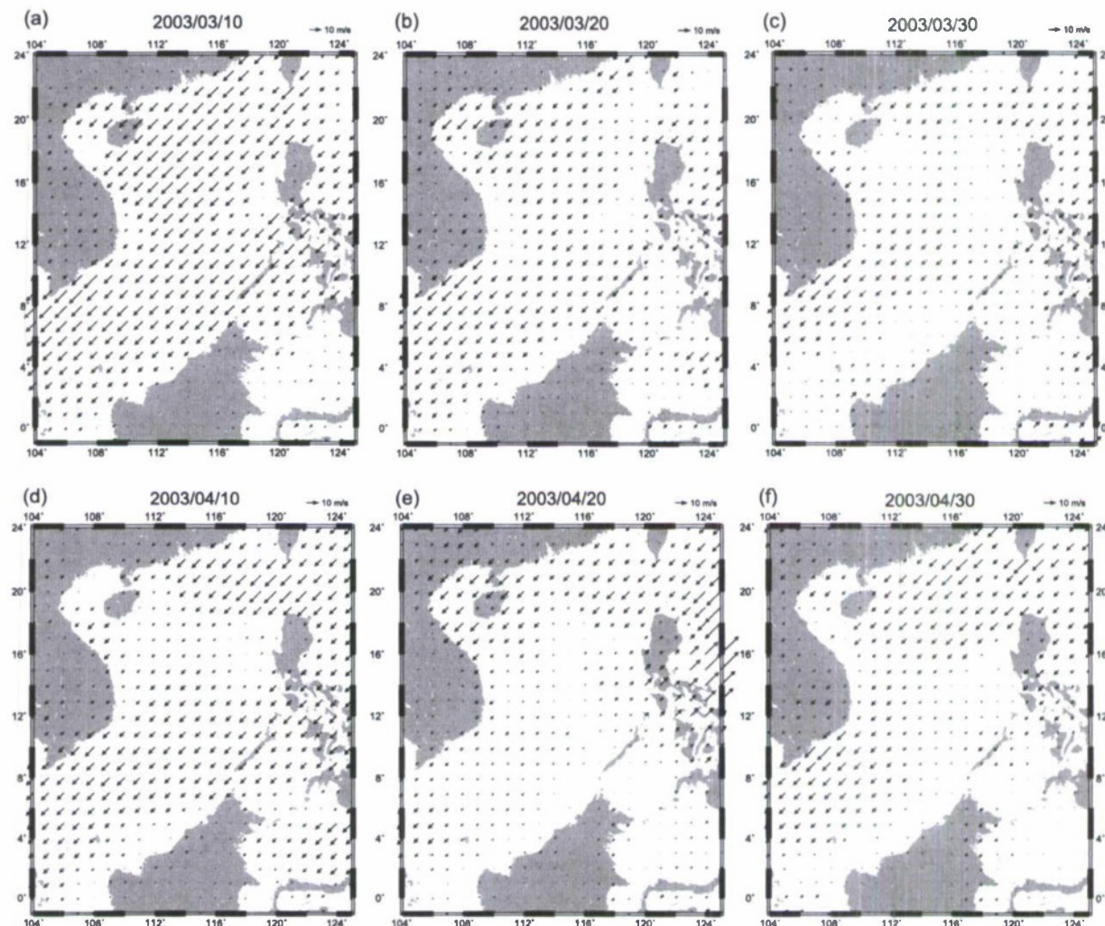
Figure 11. Wind fields from Navy Operational Global Atmospheric Prediction System (NOGAPS) on (a) 10 March, (b) 20 March, (c) 30 March, (d) 10 April, (e) 20 April, and (f) 30 April.
