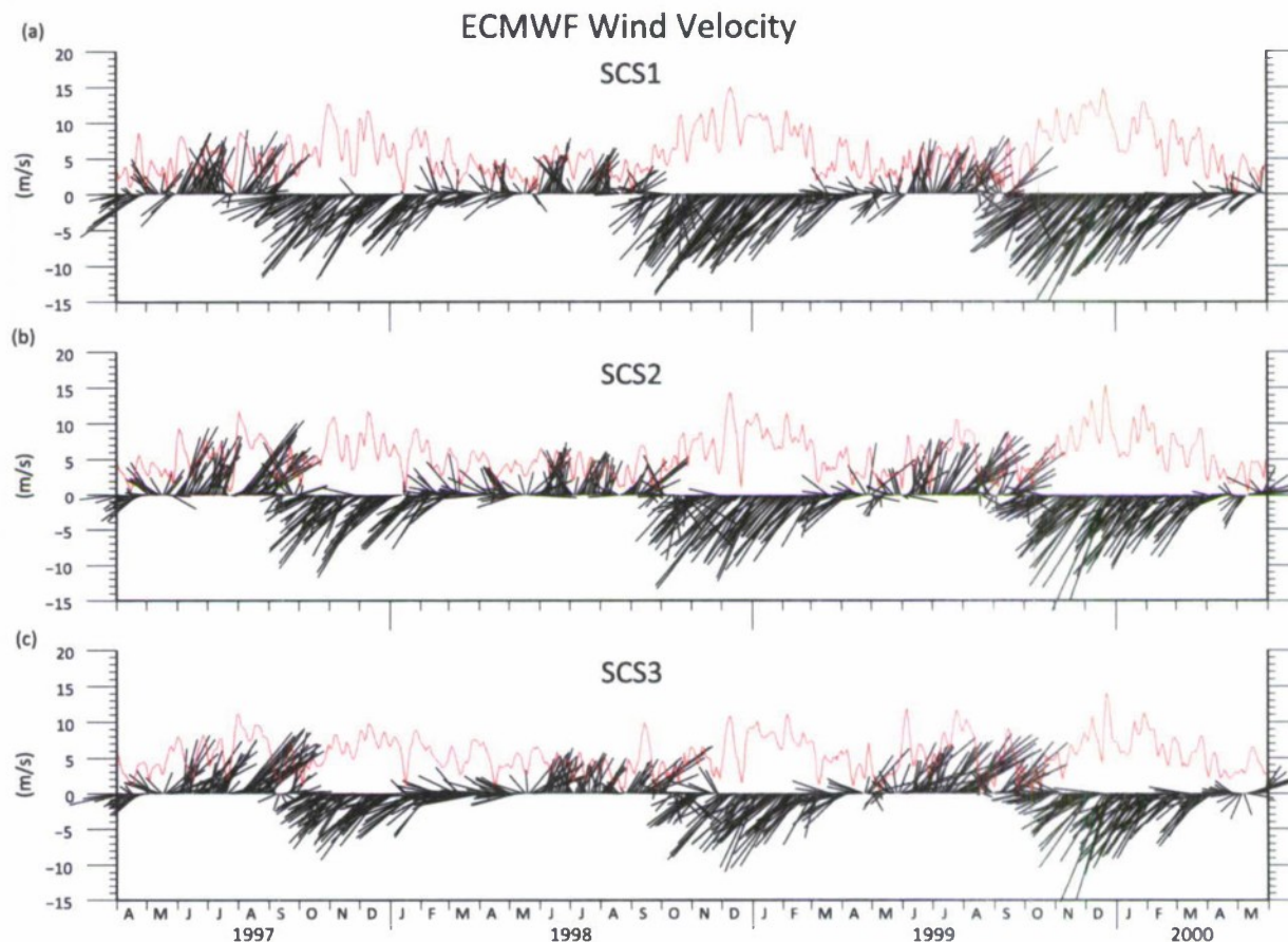
Figure 3. Wind stick (black) diagrams and wind speeds (red) at 10 m height after 96 h low-pass filtration over (a) SCS1, (b) SCS2, and (c) SCS3, from European Centre for Medium-Range Weather Forecasts (ECMWF) 40 Year Re-analysis (ERA-40).
