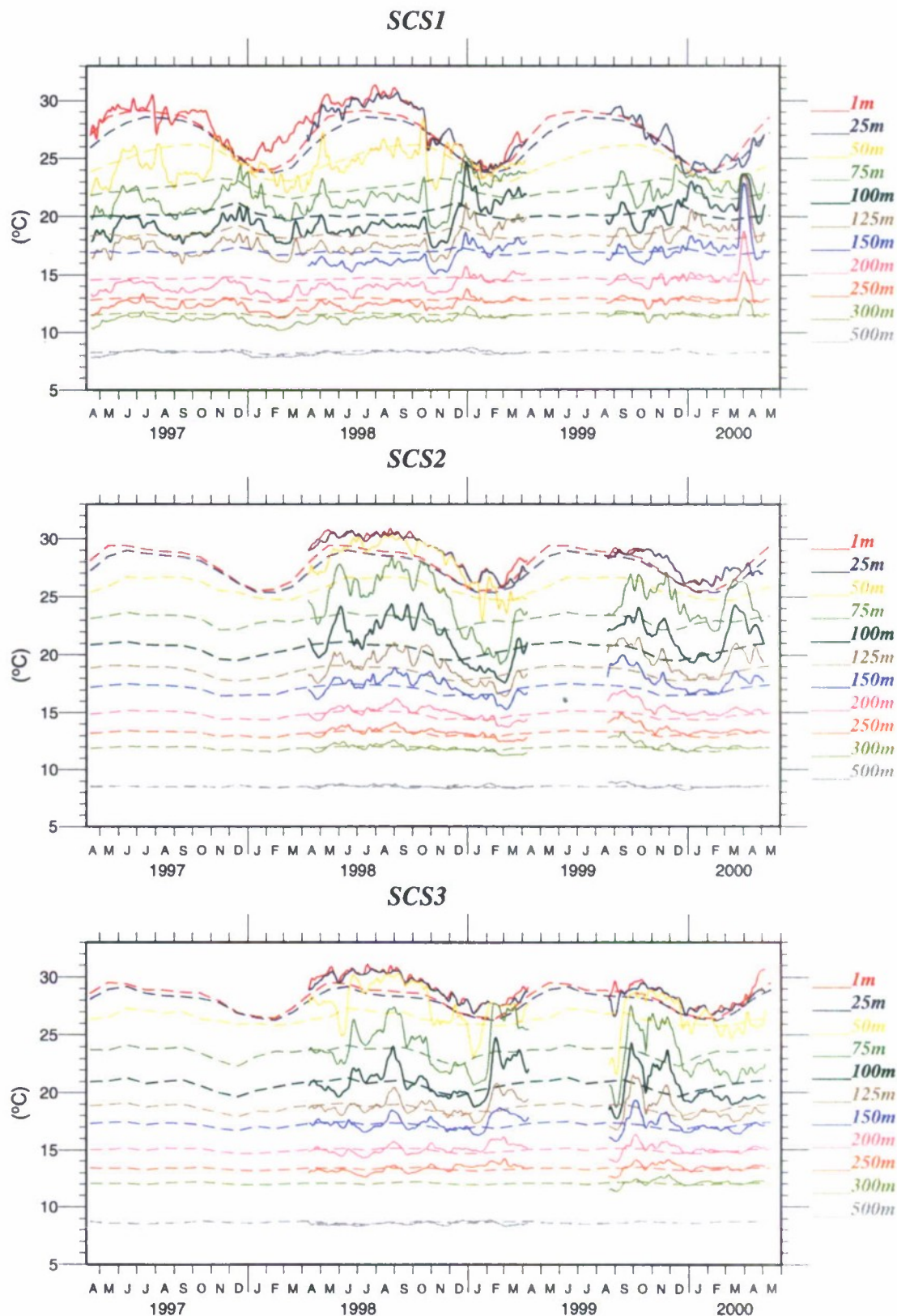
Figure 8. Time series (solid curves) of 96 h low-passed temperature at different depths at (a) SCS1, (b) SCS2, and (c) SCS3. Superimposed are corresponding time series (dashed curves) from World Ocean Atlas 2005 (WOA05).
