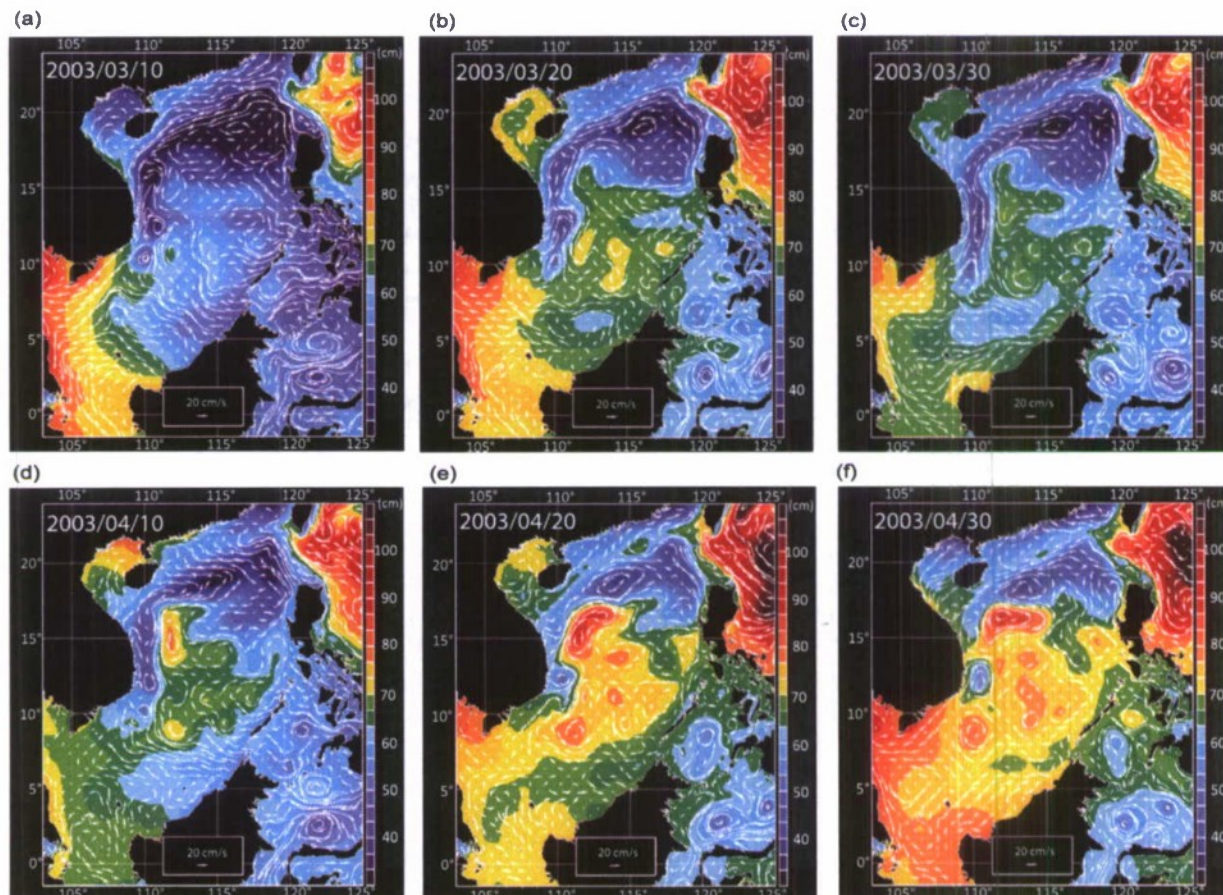
Figure 12. Sea surface height contours and currents (white arrows) from East Asian Sea Ocean Now-cast/Forecast System (EASNFS) on (a) 10 March, (b) 20 March, (c) 30 March, (d) 10 April, (e) 20 April, and (f) 30 April in 2003.
