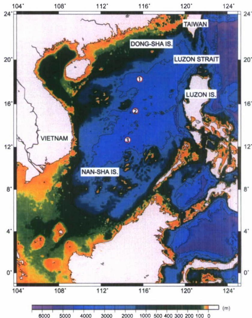
Figure 1. ATLAS buoy stations (SCS1, SCS2, and SCS3) and bathymetry in the South China Sea.
