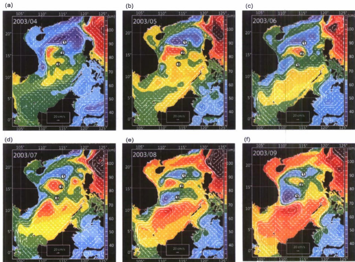
Figure 13. Same as Figure 12 except for monthly averages in (a) April, (b) May, (c) June, (d) July, (e) August, and (f) September of 2003. Buoy locations are labeled as 1, 2, and 3.
