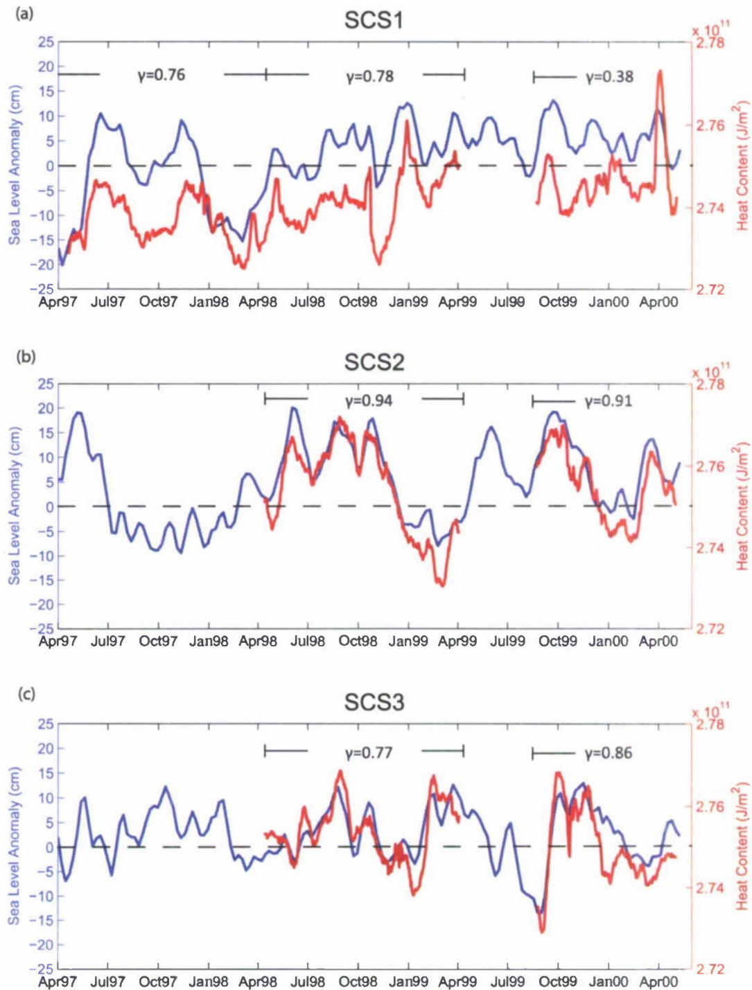
Figure 9. Heat content (red curves) in the top 250 m at (a) SCS1, (b) SCS2, and (c) SCS3, superimposed on sea level anomaly (SLA) time series (blue curves) derived from archiving, validation, and interpretation of satellite oceanographic data (AVISO). Black dash line is a reference for zero SLA. On top is the correlation coefficient ( \gamma ) between heat content and SLA in each measurement period.
