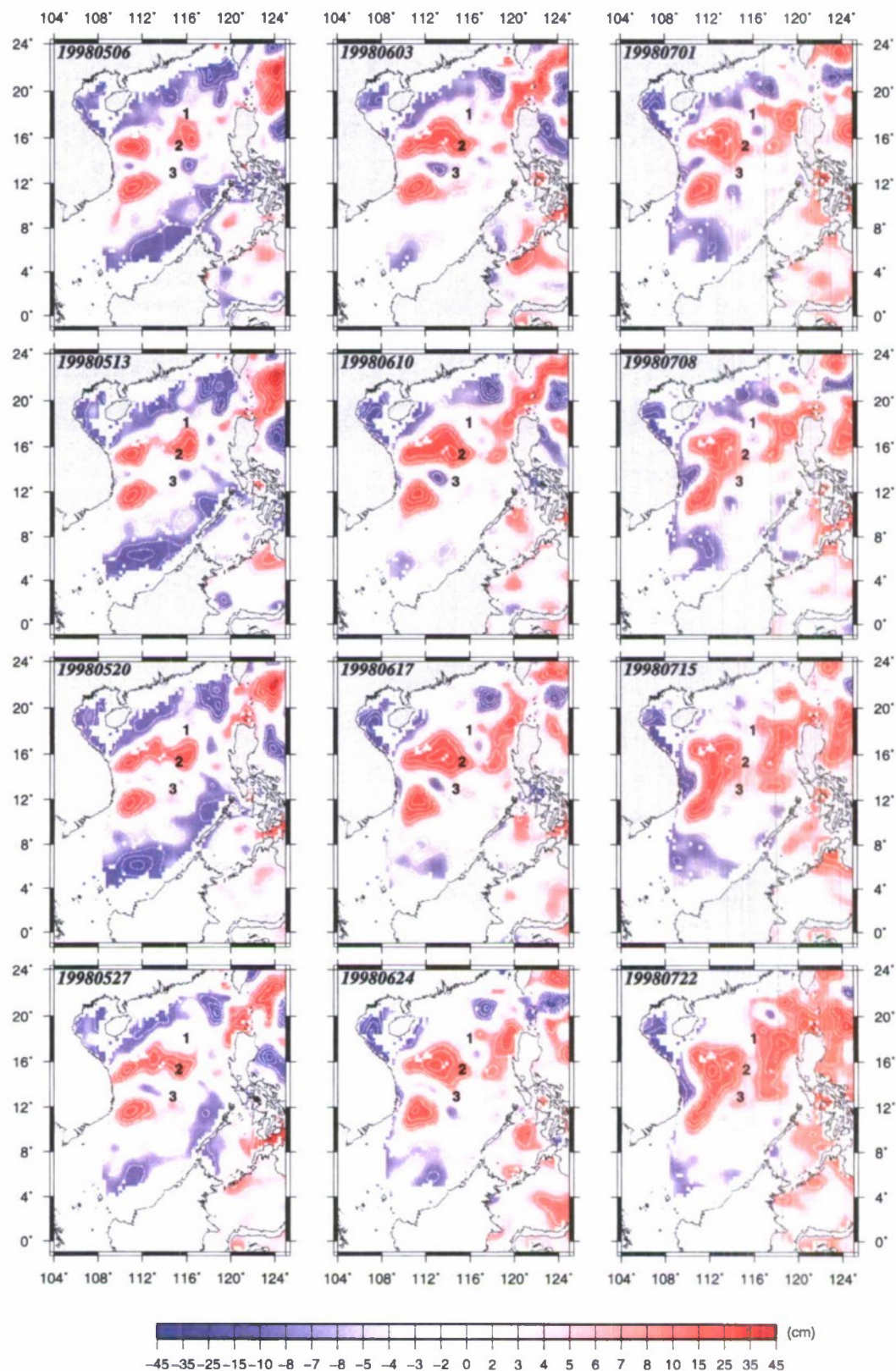
Figure 10. AVISO sea level anomalies (SLA) from 6 May to 22 July 1998 at 7 d intervals. The sequence is from top to bottom and then from left to right. Buoy locations are labeled as 1, 2, and 3. Gray shading indicates areas shallower than 200 m.
