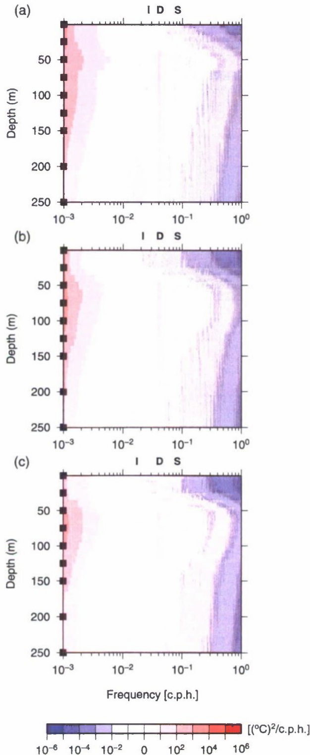
Figure 6. Variance spectrum of temperature in the top 250 m from April 1998 to April 1999 at (a) SCS1, (b) SCS2, and (c) SCS3. Solid squares on left are measurement depths. Marked on top (S, D, and I) are semidiurnal, diurnal, and inertial frequency, respectively. The inertial period is 38.3 h at SCS1, 45.4 h at SCS2, and 54.7 h at SCS3.
