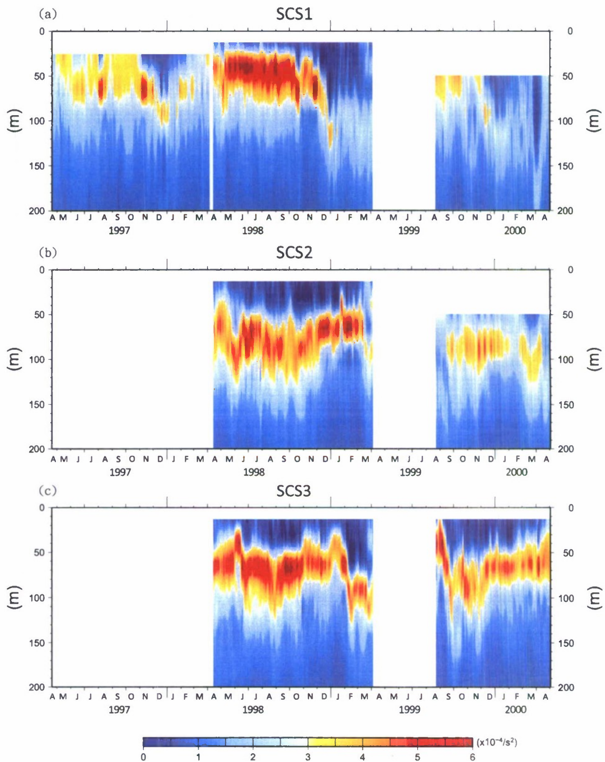
Figure 7. Brunt-Väisälä frequency square ( N^2 ) in the top 200 m at (a) SCS1, (b) SCS2, and (c) SCS3.
