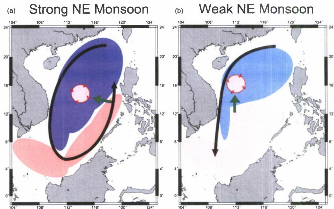
Figure 15. Schematics showing genesis of the spring-summer warm (anticyclonic) eddy in the central South China Sea after (a) a strong NE winter monsoon and (b) a weak NE winter monsoon. Black arrows illustrate basin-scale cyclonic gyres in winter. Darker blue indicates greater sea level depression induced by the winter NE monsoon, whereas darker pink illustrates higher sea level elevation above the mean. Green arrows illustrate warm eddy genesis and subsequent movement.
