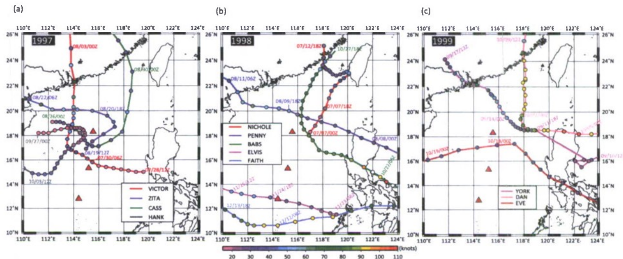
Figure 5. (a) Typhoon and tropical storm tracks dotted 6-hourly in 1997 and buoy locations (red triangles). Dot color indicates maximum wind speed in knots. Victor and Zita are Category 1; Cass and Hank are tropical storms. (b) Corresponding features in 1998: Nichole, Penny, and Elvis, tropical storms; Babs, Category 4; Faith, Category 2. (c) Corresponding features in 1999: York, Category 1; Dan, Category 3; Eve, tropical storm.
