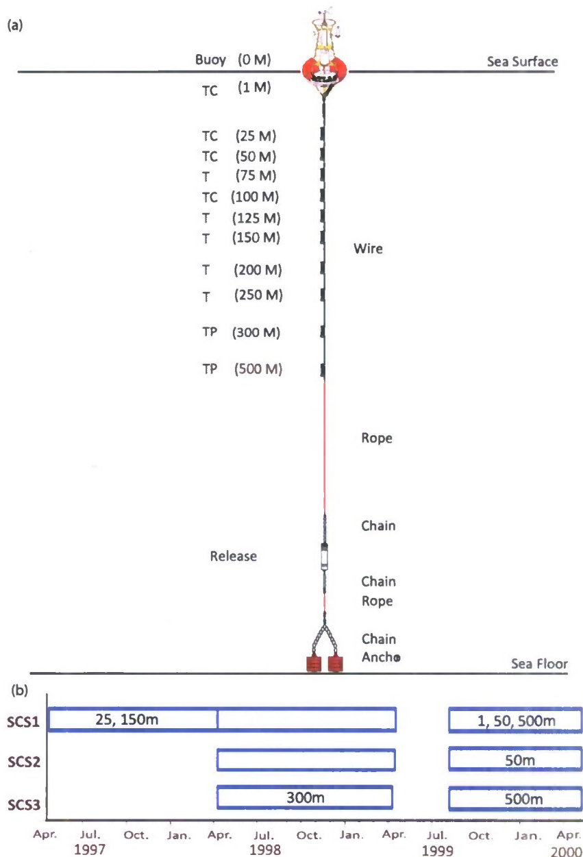
Figure 2. (a) ATLAS mooring design: T, temperature sensor, TC, temperature-conductivity sensor, TP, temperature-pressure sensor. (b) Periods of deployment and depths of lost data in each period.
