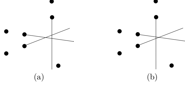
Figure 6: Different swap cell decompositions with the same order type.
