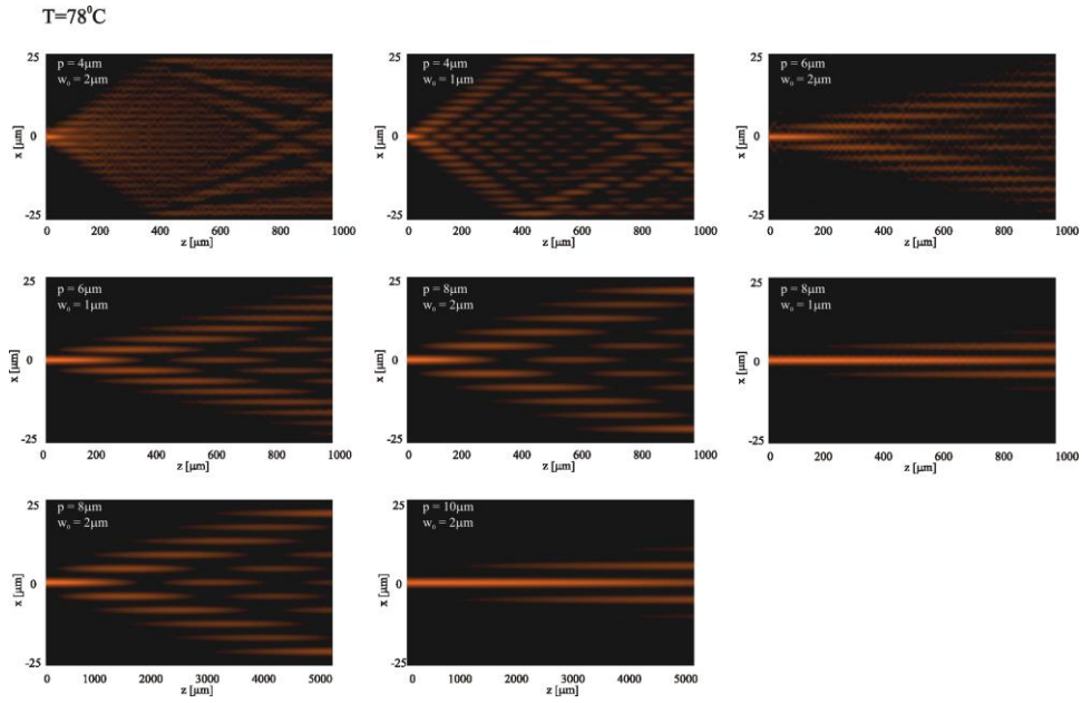
Fig. 3. Simulations of light propagation at 78^\circ\text{C} versus medium birefringence, chirality pitch and beam waist.
