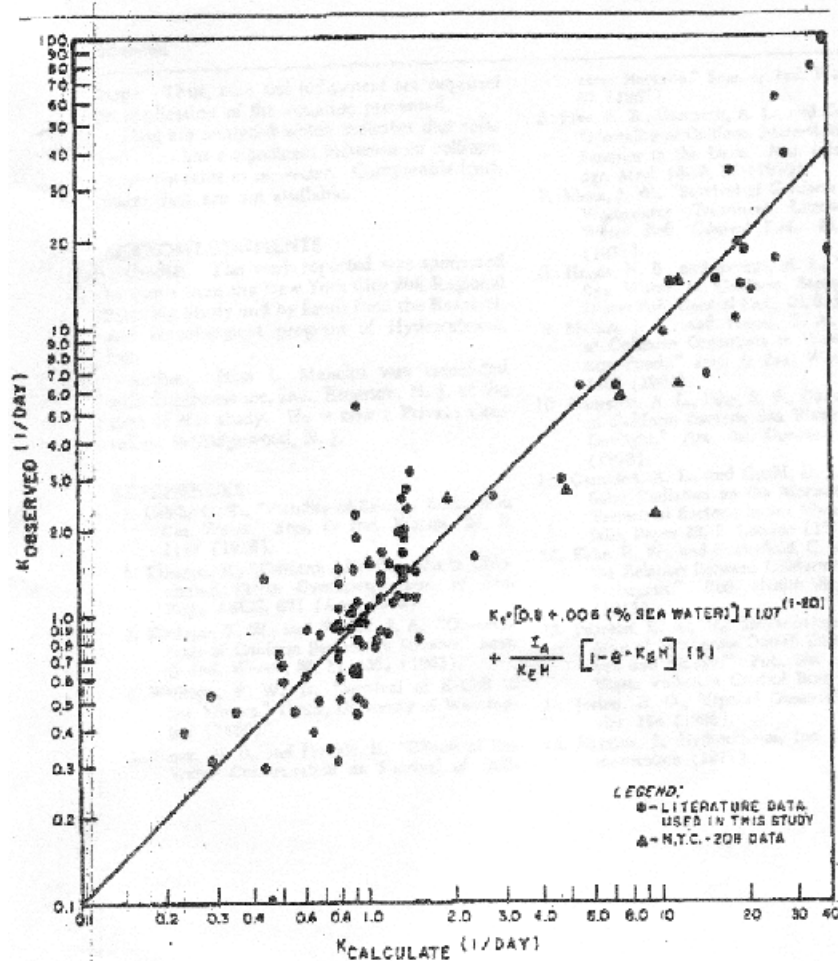
FIGURE 8. Calculated versus observed coliform mortality rates.
