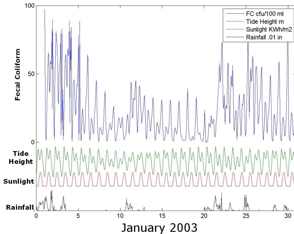
Figure 4-7. Example of simulation results for the grid cell at the mouth of Clear Creek showing the fluctuation of FC concentrations as a function of storm intensity (rainfall), solar radiation (KWh/m 2 ), and tide height (meters).
