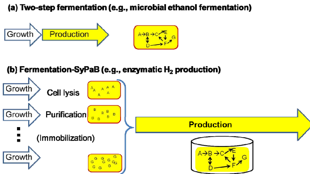
Figure 8. Process complexity comparison of microbial (ethanol) fermentation involving two steps—microorganism growth and ethanol fermentation (a) and a typical SyPaB involving protein production by microbial fermentation, protein purification and/or immobilization, and biotransformation by using the stabilized enzyme mixture (b).
