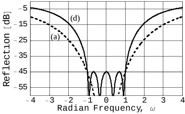
Fig. 7. A comparison of the prototype reflection responses of equal- q maximally-flat design example (a) (dashed curve) and equal- q equiripple design example (d) (solid curve).
