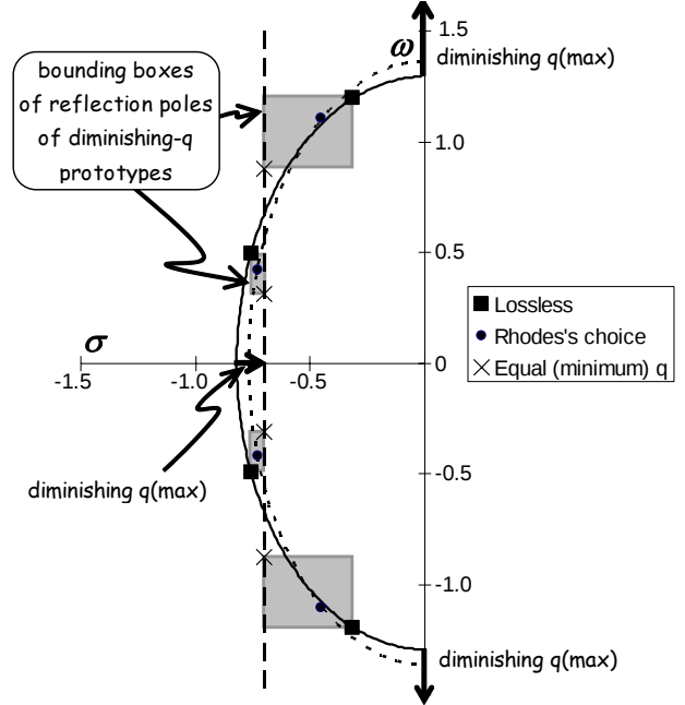
Fig. 5. Prototype LHP equiripple reflection poles for n=4 , plotted in the complex s=\sigma+j\omega plane, for three different sets of shunt admittance unloaded Qs, showing the trend in the semi-major and semi-minor axes of the ellipses through the poles as the maximum q of the shunt admittances diminishes.
