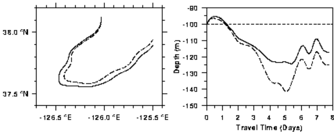
Figure 2. (left) At 100 m, horizontal water parcel trajectories computed from the geostrophic velocities (dashed line) and the higher-order gradient wind velocities (solid line); (right) net vertical displacement, computed by integrating the quasigeostrophic vertical velocity (dashed line) and higher-order vertical velocity (solid line) along the geostrophic trajectory shown at left. The displacement computed from the higher-order vertical velocity is less than the quasigeostrophic displacement, illustrating the importance of including higher-order dynamics.
