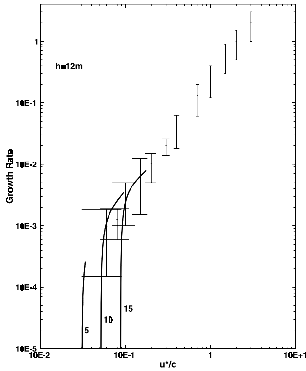
Figure 1. Linearized growth rate of wind induced waves in shallow water for depth h = 12\text{m} . Solid curves: theory for U_{10} = 5, 10, \text{ and } 15 \text{ m/s} . Error brackets show range of experimental data by Plant (1982).
